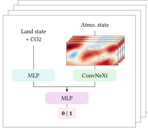
Figure 3. Diagram of the Combined Model. Includes a simple MLP for the Land-State plus a ConvNeXt model for the Atmosphere state, which are then combined using a final MLP that does the binary classification. An ensemble of 20 members is used during training to add robustness and treat the model’s epistemic uncertainty.
