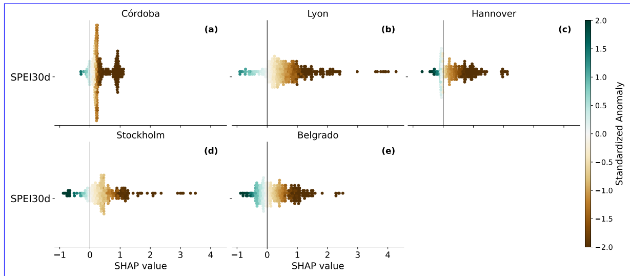
Figure D3. Same plot as in Fig. 6 but for the model using E-OBS observational data and the SPEI 30 days index as a proxy for the soil moisture feature.
