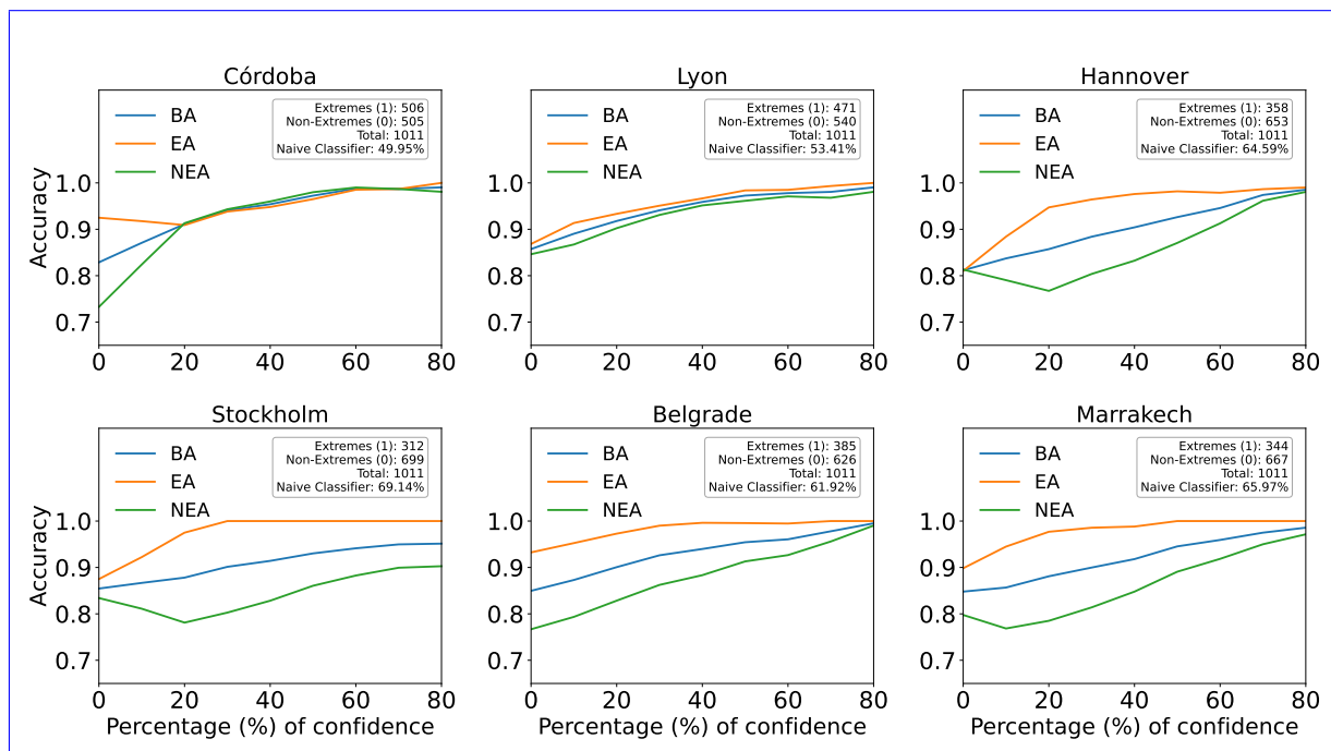
Figure B4. Same plot as in Fig. B2 but for the 80th percentile definition of extreme.
