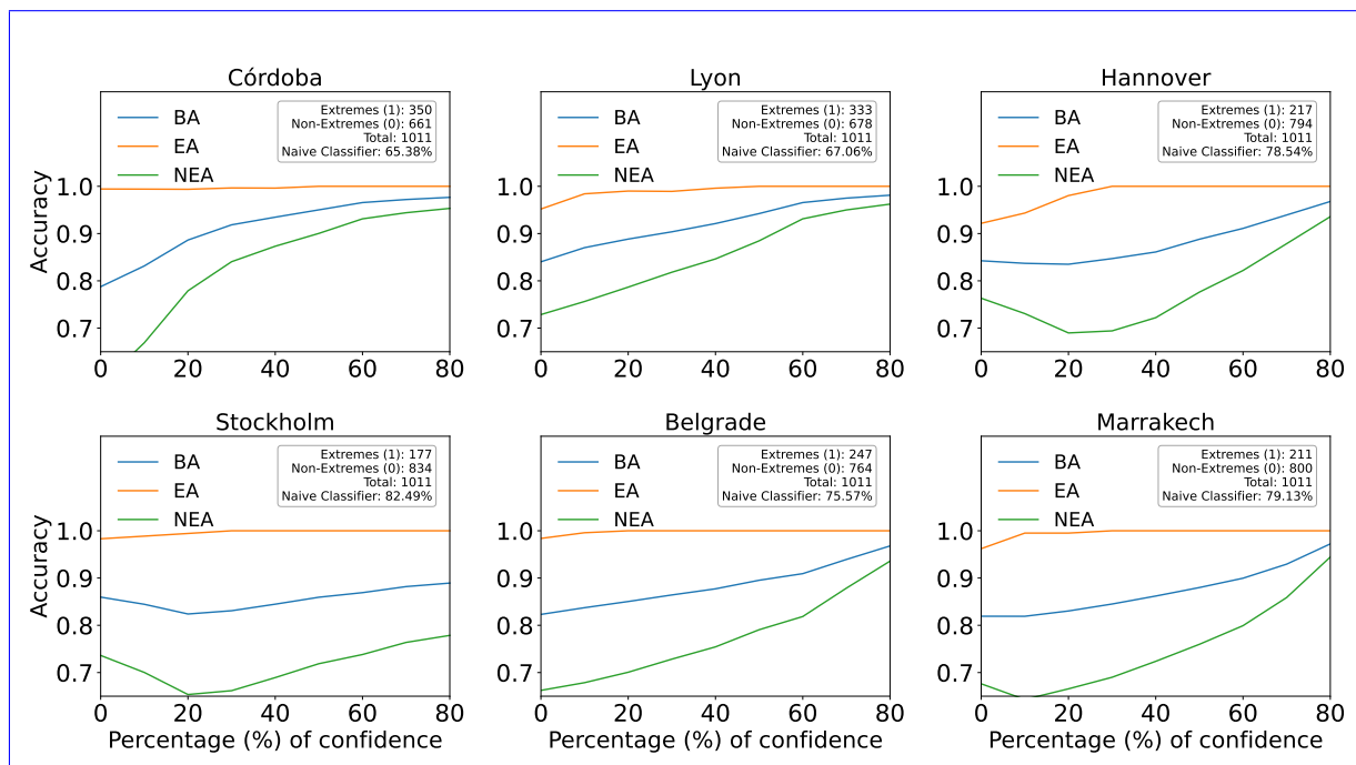
Figure B5. Same plot as in Fig. B2 but for the 95th percentile definition of extreme.
