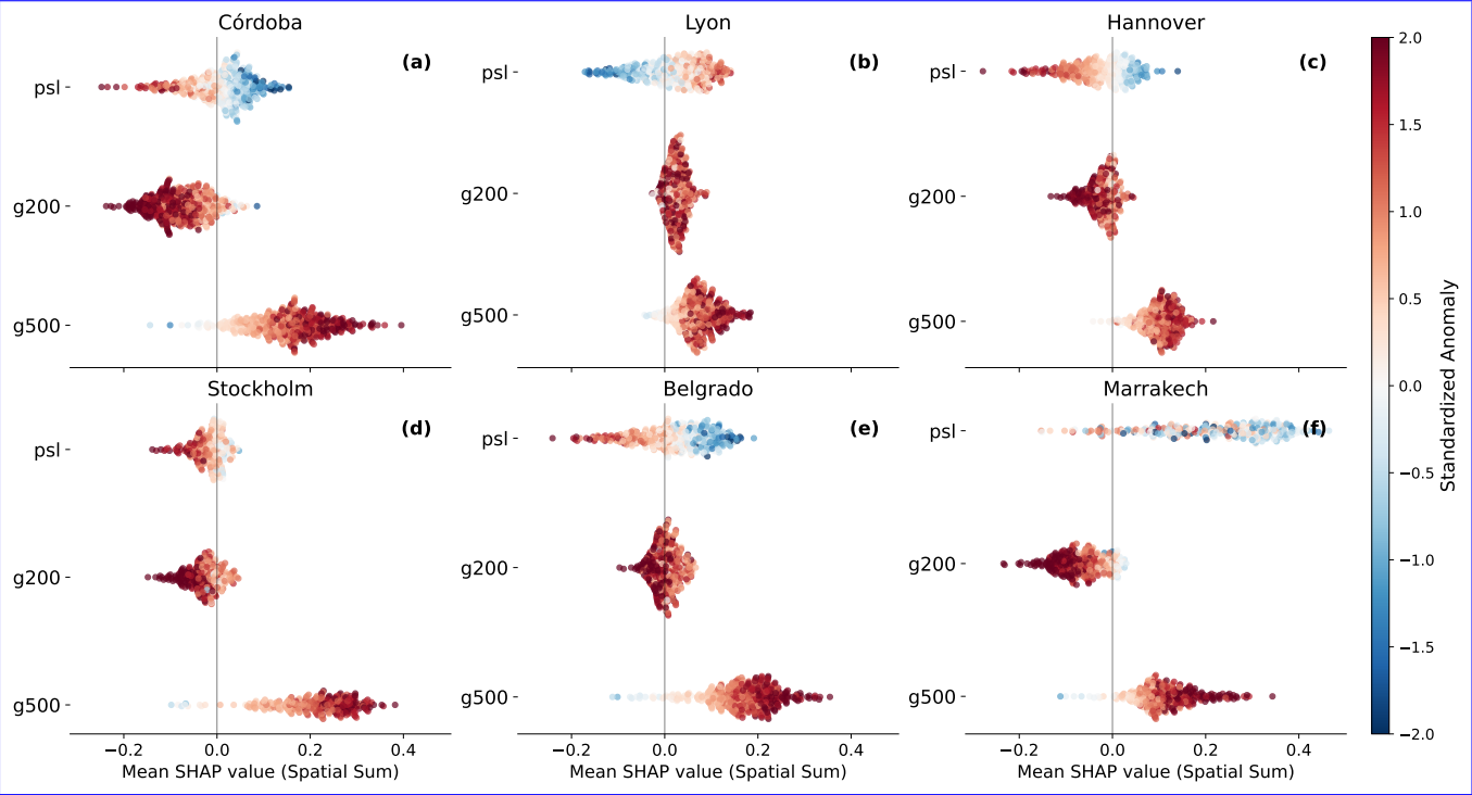
Figure D1. Same plot as in Fig. 6 but for the atmospheric circulation features. We sum up the SHAP values and averaged the standardized anomalies of the circulation variables in a 400km by 400km region surrounding the target location.
