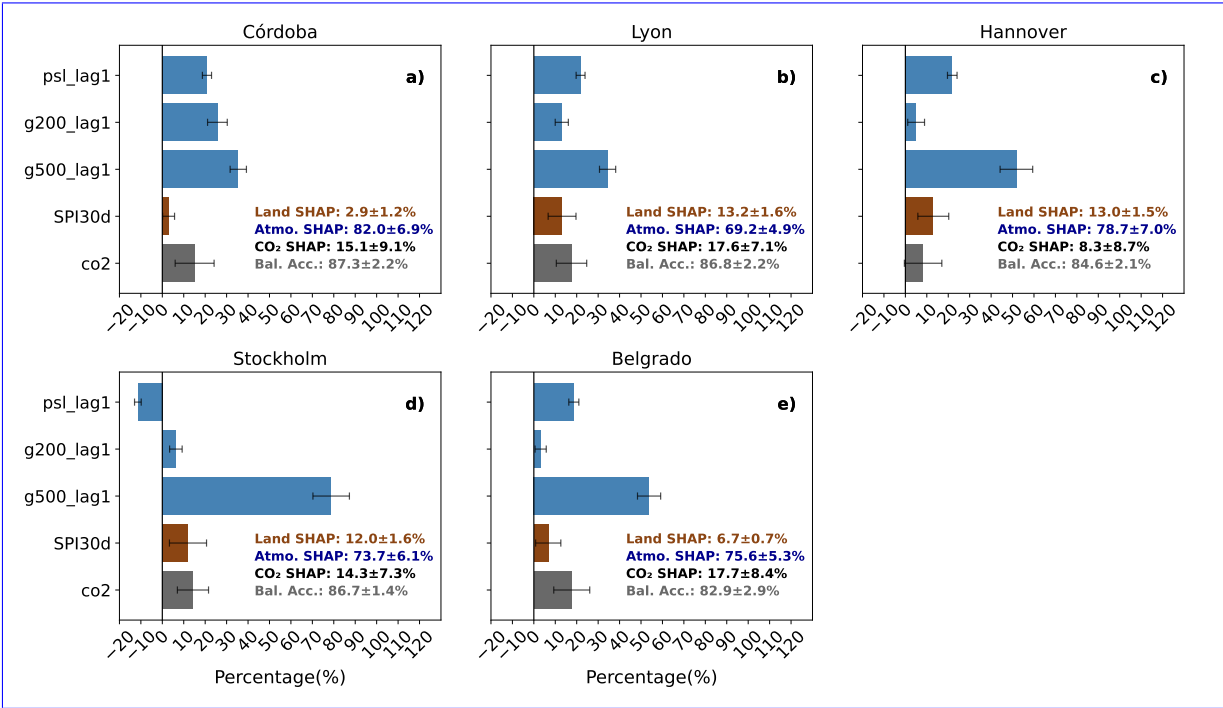
Figure D4. Same plot as in Fig. 5 but for the model using E-OBS observational data and the SPI 30 days index as a proxy for the soil moisture feature.
