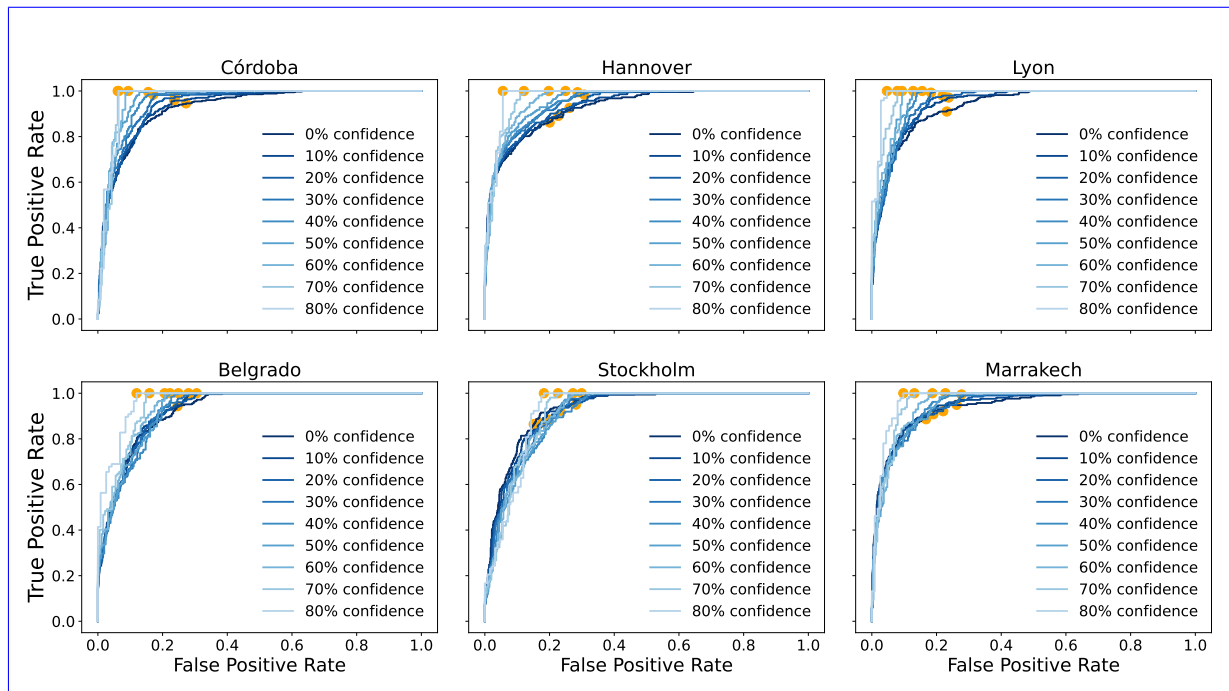
Figure B3. Change in ROC curves for the Combined Model for different percentages of confidence using the 90th percentile extreme definition. In the x-axis the false positive rate and in the y-axis the true positive rate. The legend shows the different percentages of confidence taken.
