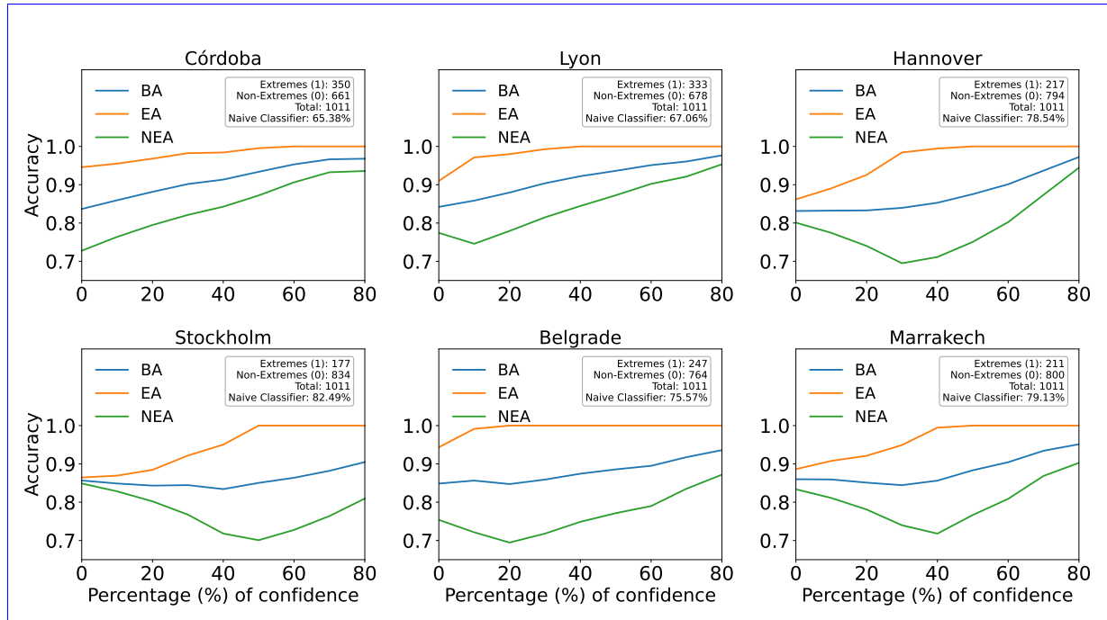
Figure B2. Change in accuracies for the Combined Model for different percentages of confidence using the 90th percentile extreme definition. In the x-axis the percentage of confidence taken, and in the y-axis the accuracies. EA, NEA and BA in the legend stand for extreme accuracy, non-extreme accuracy and balanced accuracy respectively. The text box shows the sample size and the random chance of the naive classifier.
