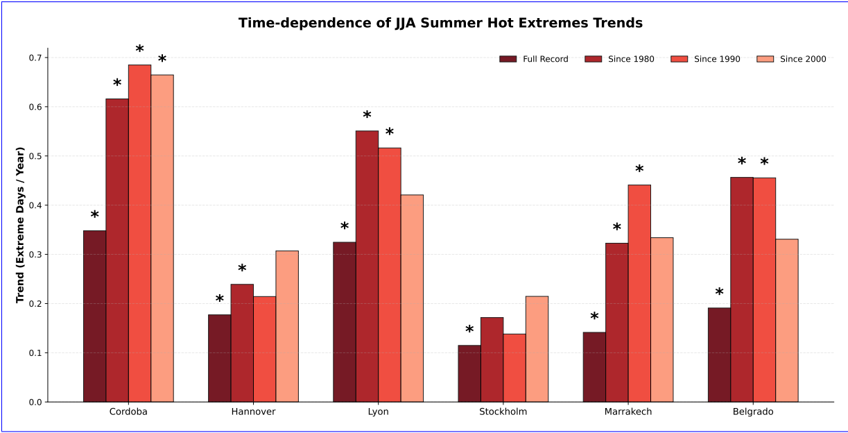
Figure B1. Trends in JJA Summer Hot Extremes across different time periods. Bars represent the slope coefficient (trend magnitude) of a linear regression applied to the yearly count of extreme days for four periods: the full available record (dark red), since 1980 (red), since 1990 (light red), and since 2000 (lightest red). Asterisks (*) indicate trends that are statistically significant at the 95% confidence level, determined using a t-test on the slope coefficient.
