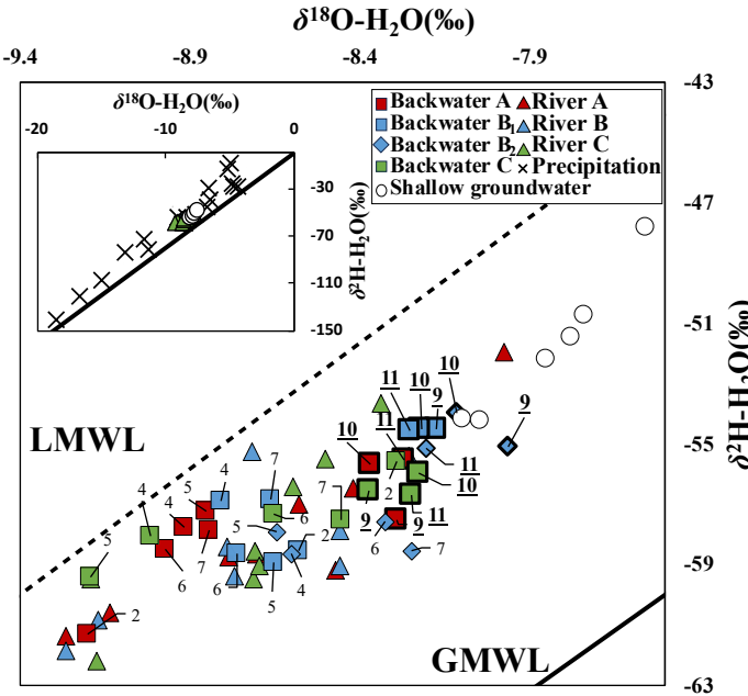
255 Figure 4 Overall diagram (upper left) of hydrogen and oxygen isotope ratios ( \delta^2\text{H} , \delta^{18}\text{O} ) in rivers, spring water at backwater, and shallow groundwater during the survey period and enlarged diagram. GMWL and LMWL represent the Global Meteoric Water Line ( \delta^2\text{H} = 8\delta^{18}\text{O} + 10 ) and the Local Meteoric Water Line ( \delta^2\text{H} = 8.3\delta^{18}\text{O} + 18 ), respectively. The numbers attached to each symbol indicate the month of sampling. The data obtained in autumn is indicated by symbols enclosed in thick lines and the month of sampling underlined. 260
