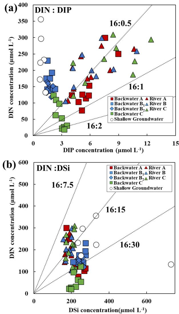
Figure 9 (a) DIN and PO_4^{3-} concentrations and (b) DIN and DSi concentrations of spring water in each backwaters, river water, and shallow groundwater plotted with dotted lines indicating typical composition
