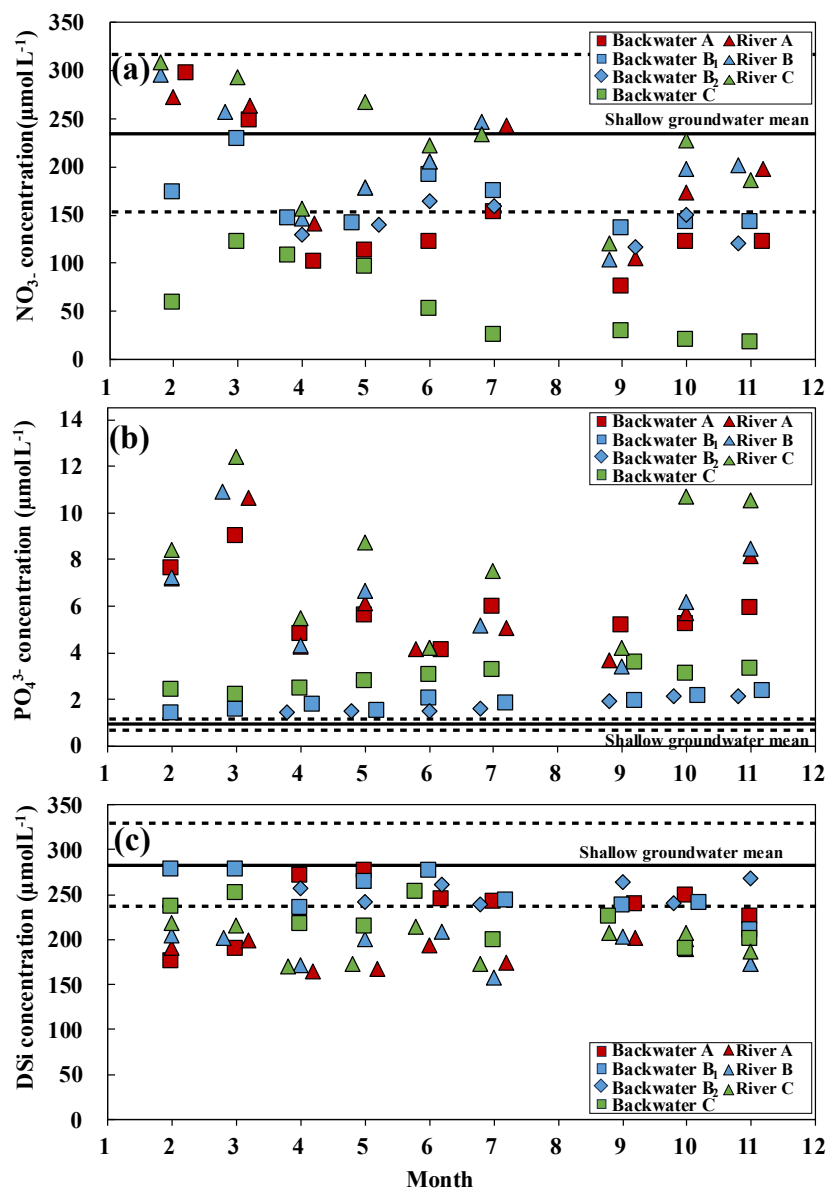
295 Figure 7 Seasonal variation in (a) \text{NO}_3^- , (b) \text{PO}_4^{3-} , and (c) \text{DSi} concentrations of backwater spring water and adjacent rivers. The solid line and broken lines in each graph indicate the average and standard deviation of shallow groundwater, respectively.
