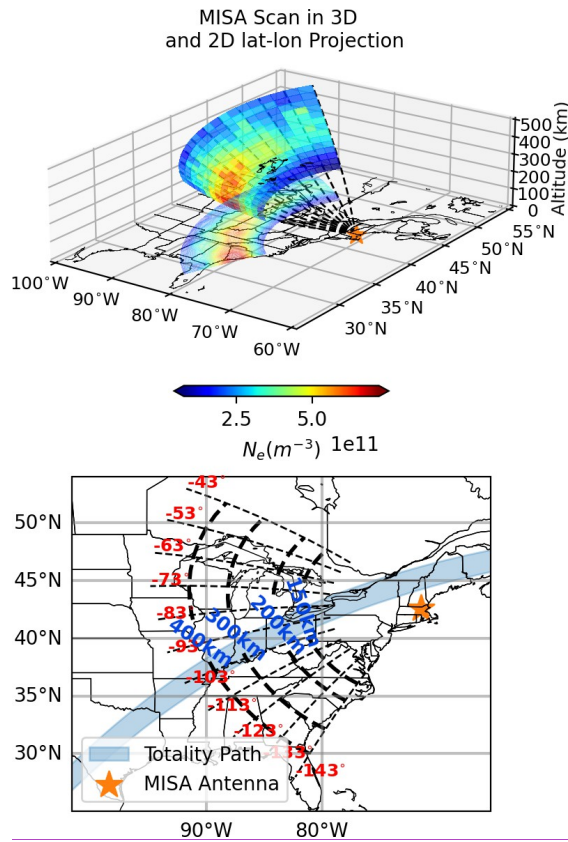
Figure 1. Upper panel shows N_e measurements from a 6° elevation MISA scanning experiment on the day of the eclipse. The latitude-longitude projection is displayed on the 0 km altitude plane. The second panel illustrates the approximate azimuth angles and altitudes of the MISA steerable antenna main beam across different scans on Apr 8, 2024 on a 2D plane. Totality path is superimposed on the diagram.
