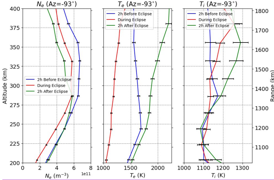
Figure 3. Altitude profiles of the observed N_e (left), T_e (middle) and T_i (right) 2 hrs prior to the eclipse (blue), during the eclipse (red) and 2 hrs after the eclipse (green).
