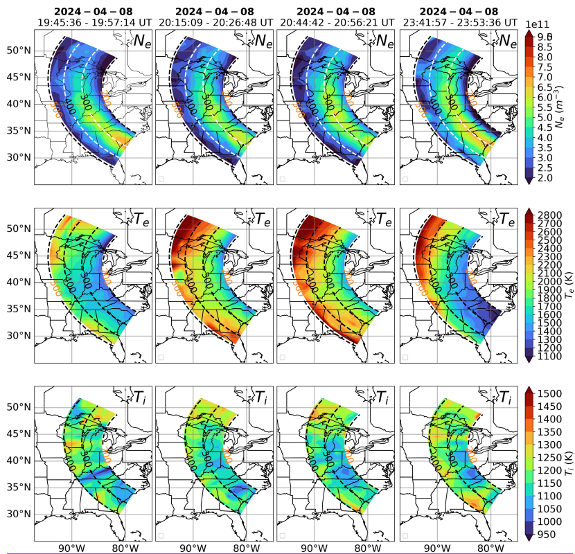
Figure 6. Same as Figure 5 but for four subsequent scans. The first three columns display consecutive scans that occur immediately after those in Figure 5, and the fourth column shows the scan which occurs at the end of the day (23:41 - 23:53 UT) to evaluate whether or not the parameters have recovered to pre-eclipse levels.
