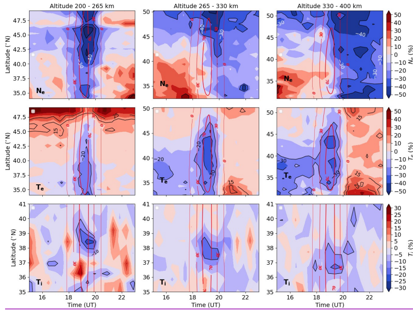
Figure 13. Each column of this figure displays the percent difference between data and model for N_e , T_e , T_i at a given latitude over the time interval of 15 - 24 UT and for parameters averaged over three equal altitude sub-intervals from 200 - 400 km: 200 - 265 km (left column), 265 - 330 km (middle column), and 330 - 400 km (right column). Eclipse obscuration percentage is shown using red contour lines. The largest drops in N_e from 40 - 50 % occur above 40°N. T_e decreases are seen from 18 -20 UT and do not persist later in the day as for N_e . T_i decreases from 10 -15 % along a narrow range of latitudes which correspond closely to the path of the totality.
