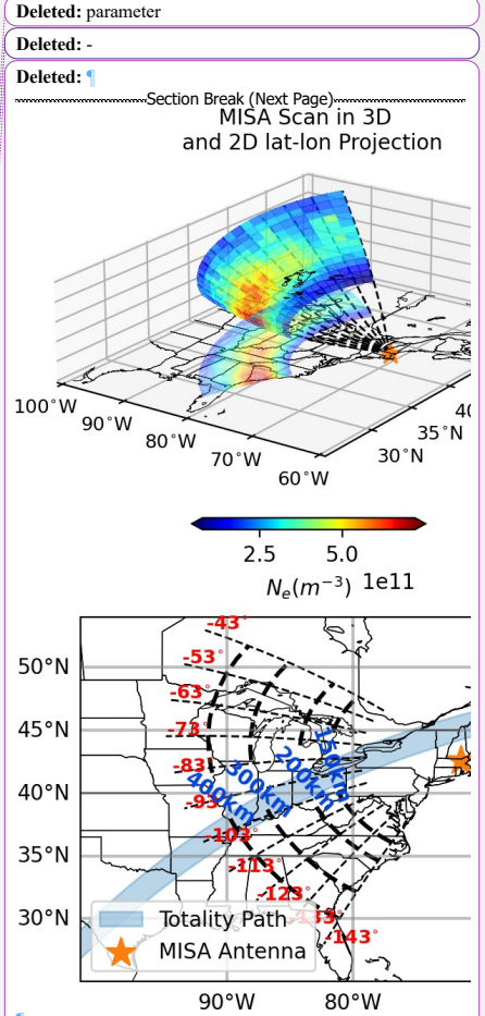
Figure 1. Upper panel shows N_e measurements from a 6° elevation MISA scanning experiment on the day of the eclipse. The latitude-longitude projection is displayed on the 0 km altitude plane. The second panel illustrates the approximate azimuth angles and altitudes of the MISA steerable antenna main beam across different scans on Apr 8, 2024 on a 2D plane. Totality path is superimposed on the MISA scanning region.
