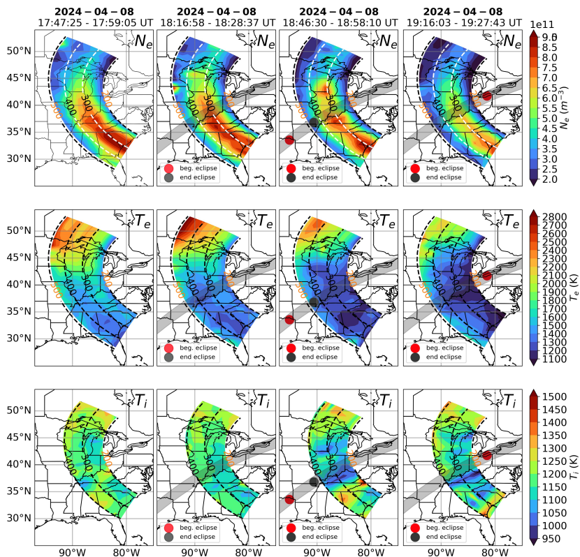
Figure 5. Azimuthal scans of N_e (top row), T_e (middle row), and T_i (bottom row) parameters on the day of the eclipse (Apr 8, 2024) at four different times: prior to the eclipse passing over the scanning area, when the totality path overlaps with the furthest processed ranges of the scanning area ( > 500 km altitude), when the totality path overlaps the nearest ranges of the scanning area ( < 150 km altitude), and when the totality has moved eastward away from the scanning area. Red circles show the position of the totality during the first azimuthal scan and black circles show the position of the totality during the last azimuthal scan. Mild drop in N_e (second column) can be seen around 300 km when the totality approaches the furthest scanning area and continues to decrease much more in the next hour shown. The drop in T_e occurs at most latitudes and longitudes of the scanning region before the totality appears overhead, whereas N_e drops are visible when the totality is overhead. White or black dashed circular contour lines indicate the scanning altitude. Grey semi-transparent thick line indicates the path
