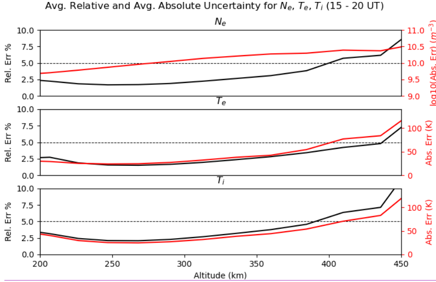
Figure 4. Altitude profiles of relative (in black) and absolute errors (in red) of N_e , T_e and T_i averaged over 15 - 20 UT and across all azimuths.
