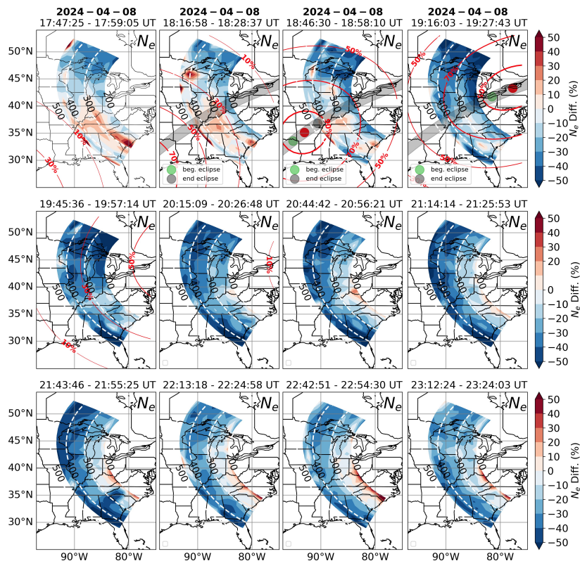
Figure 7. Percent difference MISA scan figures that show a difference between N_e observations and model predictions on Apr 8, 2024 for 12 consecutive MISA low elevation scans that cover the period before, during, and after the eclipse. Altitude contour lines and position of totality are shown as in previous figures along with eclipse obscuration percentage (red contour lines). N_e decreases are visible for the first time in the third scan and continue further in the fourth and fifth scans. Subsequent scans show F1 region recovery of N_e and topside persistence of decreased N_e values. Largest drops (40 - 50%) of N_e appear at various latitudes and altitudes after the passage of the eclipse.
