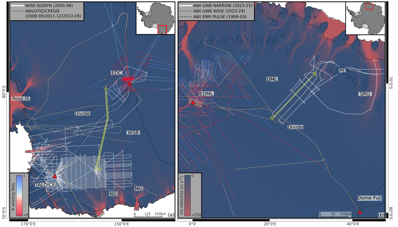
Figure 1. Map of the airborne radar datasets used in this study for WSB (a) and DML (b) regions. (a) BAS WISE-ISODYN survey (white solid lines) and a combination of individual flight lines (grey dashed lines) from AWI (EMR 60ns pulse data, otherwise referred to in this paper as "short-pulse"; 2008–09), CReSIS (MCoRDS; 2013–19), and UTIG (HiCARS; 2011–12) (Table 1). (b) newly acquired AWI UWB (narrowband) CHARISO survey lines (white solid lines; 2023–25) and a combination of individual flight lines (grey lines) from AWI's EMR (short-pulse; 1999–03; solid lines) and UWB (wideband mode; 2022–23; dashed lines) radars (Table 1). Also shown are the previously published IRH datasets used in this study to tie our IRHs to existing age–depth profiles from Winter et al. (2019) and Cavitte et al. (2021) over WSB (a) and Franke et al. (2025a) over DML (b), with the colorscale representing the number of IRHs traced at a particular position (ranging from 1 to >8 in both (a) and (b)). The background map shows modern ice-flow speeds from Rignot et al. (2017) in m/a. The black lines represent the RINGS/Bedmap3 grounding line from Pritchard et al. (2025) and the main drainage basin boundaries are from IMBIE (2018). The red triangles depict the location of the deep ice cores used in this study to date IRHs. The two yellow rectangles in (a) and (b) represent the location of profiles A-A' and B-B' shown in Figure 3 for the data-model comparison. Abbreviations on (a) and (b) are as follows: EDC (EPICA Dome C), EDML (EPICA Dronning Maud Land), Mertz Glacier (MG), Ninnis Glacier (NG), Belgium's Princess Elizabeth Station (PE), Ross IS (Ross Ice Shelf), SRG (Sør-Rondanebreen Glacier). Note that throughout the paper, grid-west, grid-east, and grid-south are defined relative to the map grid orientation shown here and not to geographic north.
