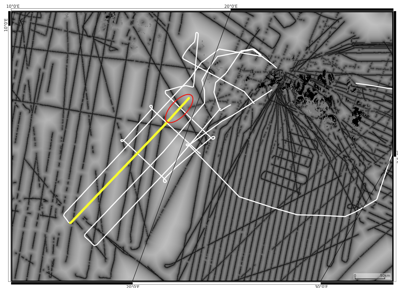
Figure B1. Bed uncertainty from the Bedmap3 dataset over DML, where dark grey lines represent the underlying data used to grid the final data product, and the light gray spacing represents gaps between known survey lines where the interpolation is conducted. Overlaid on top are the new CHARISO radar lines acquired as part of this paper (and which were not integrated in the latest iteration of the Bedmap gridding product), and in yellow the profile B-B' from Figure 3b, with the last ~40 km circled in red.
