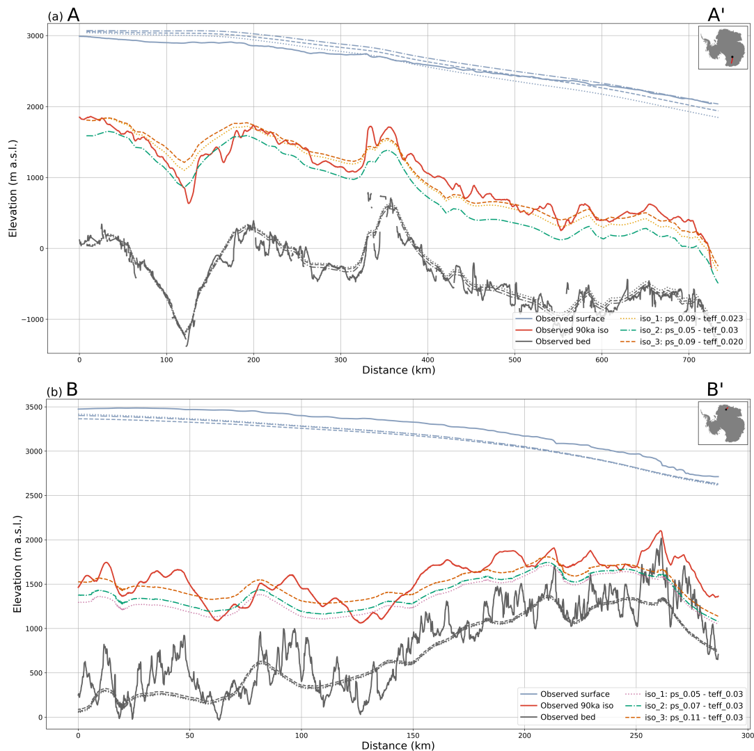
Figure 3. Comparison of the 90-ka isochrone from observations and model simulations generated in this study, along profiles A-A' (WSB, a) and B-B' (DML, b) crossing the ice divide (start) to fast-flowing ice downstream (end). The solid lines represent the observed (i.e., picked) ice surface, bed and isochrone elevations from the radar data. The non-solid lines (dashed, dashed-dotted, and dotted) represent three simulations that were ran to simulate an accurate paleo-evolution of the two catchments. For each observed surface, bed and isochrone from the radar, we show the three corresponding modelled surfaces, isochrones, and beds which were transiently simulated by the model. Exact location of profiles A–A' and B–B' is shown in Figure 1. The abbreviations "ps" and "teff" in the plot legends refer respectively to the precipitation scaling and till effective pressure parameters mentioned in Section 3.2.1, and the "iso" numbers (ranging from 1 to 3) preceding these refer to each of the three simulations matching the specific parameter values for "ps" and "teff" in the legends. For simplicity, we refer to each of these simulations in the text and in Table C1 using this "iso" numbering abbreviation.
