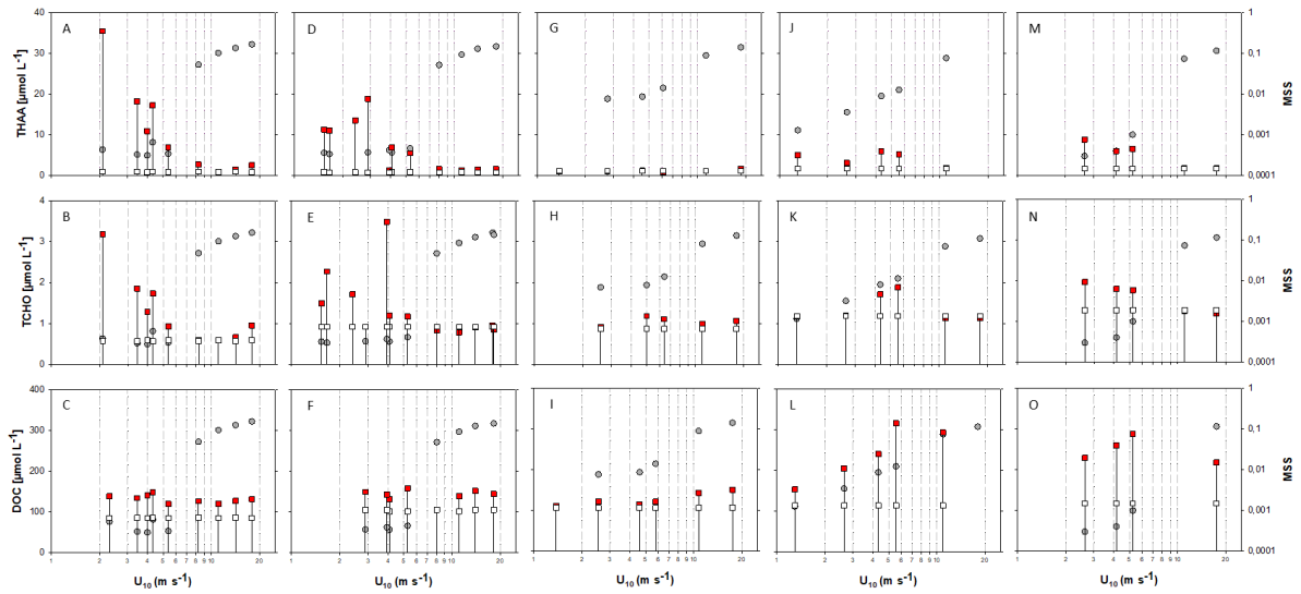
Figure 5A-O: Changes in organic matter components in the SML (red rectangles ) and ULW (grey rectangles ) at different wind speeds ( U_{10} ), and associated MSS values (grey circles). For better coverage of wind speeds, samples with similarities in SML biopolymer concentrations and surface coverage were pooled , specifically, samples were grouped for days 2 and 4: A-C and days 9 and 11: D-F. Day 15: G-I, day 22: J-L, day 24: M-O. Drop lines show indicate associated SML-ULW pairs.
