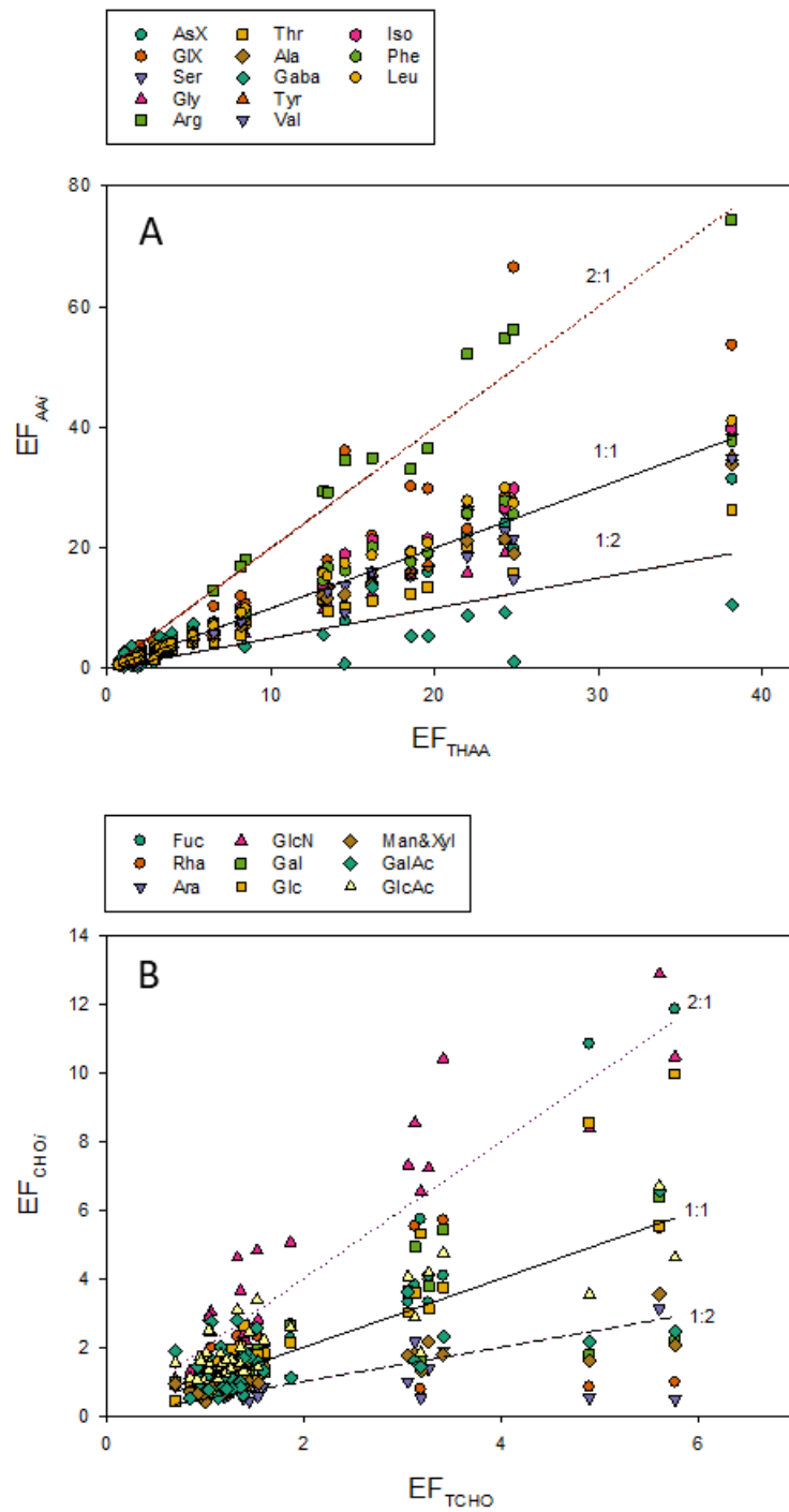
511 Figure 7A, B: Relationships between Enrichment Factors (EFs) of individual amino acids ( EF_{AAi} ) and total 512 hydrolysable amino acids ( EF_{THAA} ) (A) and between EFs of individual sugars ( EF_{CHOi} ) and total combined 513 carbohydrates ( EF_{TCHO} ) (B). Lines shown for reference: 2-fold enrichment (2:1), no enrichment (1:1) and 514 2-fold depletion (1:2).
