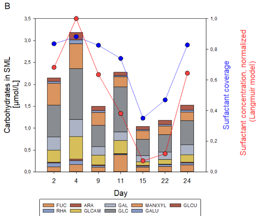
Figure 2A, B: Concentration/composition of (a) THAA and (b) THCO in the SML at low initial wind speed (1.3-2.0 ms -1 ) and variation of surfactant surface coverage (sc, blue circles), as well as normalized reduced bulk SML surfactant concentration (c*/c max , red circles). Based on a dataset first published in Engel et al. (2018).
