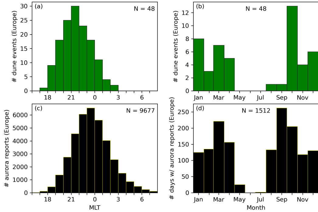
Figure C1. Same as Fig. 3 but considering only the Skywarden reports from the European sector.
