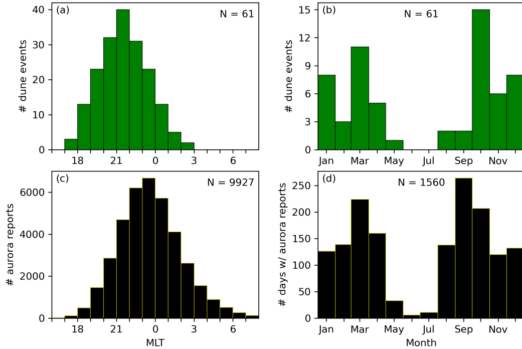
Figure 3. (a) MLT distribution of the dune observations, combining reports from multiple observers during each event. (b) Monthly distribution of individual dune aurora events. (c) MLT distribution of all aurora observation times. (d) Monthly distribution of individual days with aurora observations in Skywarden.
