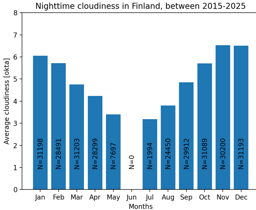
Figure B2. Average nighttime cloudiness in Finland (expressed in okta) based on the Finnish Meteorological Institute’s open data hourly values cloud-okta values, during 2015–2025. Nighttime hours are defined when the Sun’s elevation is at least 10^\circ below the horizon (i.e. solar zenith angle greater than 100^\circ ). The number of nighttime days contributing to a given month’s statistics is indicated in the corresponding bar of the diagram.
