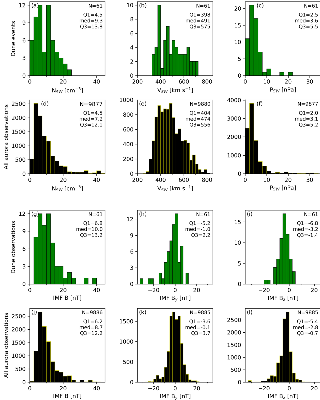
Figure 5. Solar wind and IMF parameters associated with dune events (green histograms) and all aurora observations (black histograms). The considered parameters are: (a,d) solar wind proton number density; (b,e) solar wind speed; (c,f) solar wind dynamic pressure; (g,j) IMF magnitude; (h,k) IMF B_y component; and (i,l) IMF B_z component.
