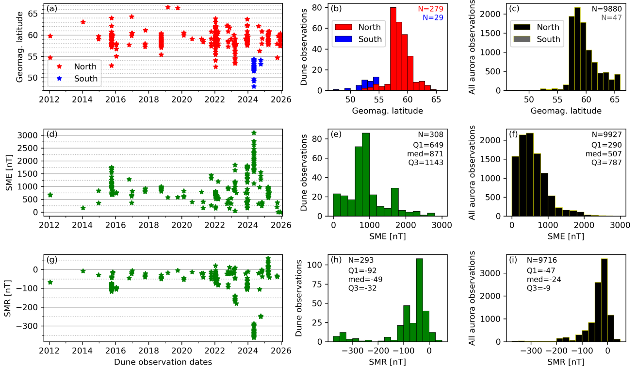
Figure 6. (a) Geomagnetic latitude of dune observations (individual reports) as a function of the observation dates, and (b) corresponding distribution. Northern-hemisphere latitudes are shown in red and southern-hemisphere latitudes (projected to the northern hemisphere) in blue. (c) Geomagnetic latitude distribution of all aurora observations; northern-hemisphere latitudes are shown in black and southern-hemisphere latitudes in grey. (d) SME index of dune observations as a function of the observation dates, and (e) corresponding distribution. (f) SME index distribution of all aurora observations. (g–i) Same for the SMR index.
