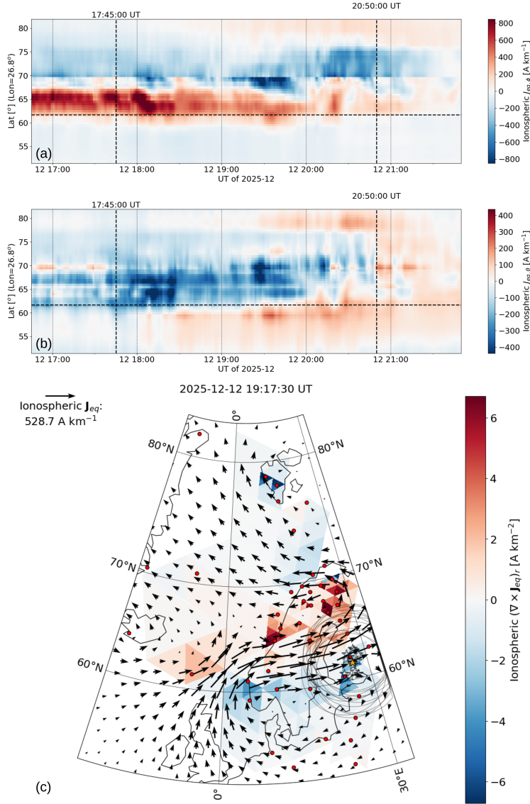
Figure 7. Equivalent current analysis applied to dune observations in the Finnish sector during the 12 December 2025 event. (a) \phi (positive eastwards) component of the equivalent currents. The horizontal dashed line indicates the average geographic latitude of the dune observations; the vertical dashed lines indicate the earliest and latest dune observations. (b) \theta (positive southwards) component of the equivalent currents. (c) Map of the equivalent currents at 19:17:30 UT. The colour scale indicates the curl of the calculated equivalent currents, with positive (negative) values being a proxy for upward (downward) field-aligned currents. The arrows indicate the direction and magnitude (scale given in the top-left corner of the panel) of the horizontal currents. The locations of the dune observers during this event are indicated with white stars; they are surrounded with circles representing the uncertainty in the actual location of the dunes (see text). The yellow star shows the mean location of the retained dune observations, and magnetometer stations used in the SECS analysis are shown with red dots.
