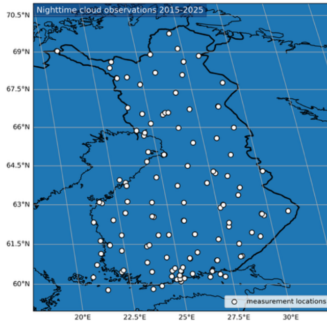
Figure B1. Locations of the cloud-okta-observing weather stations, based on FMI's open data cloud-okta measurements, within [20, 32]^\circ E and [59, 71]^\circ N.
