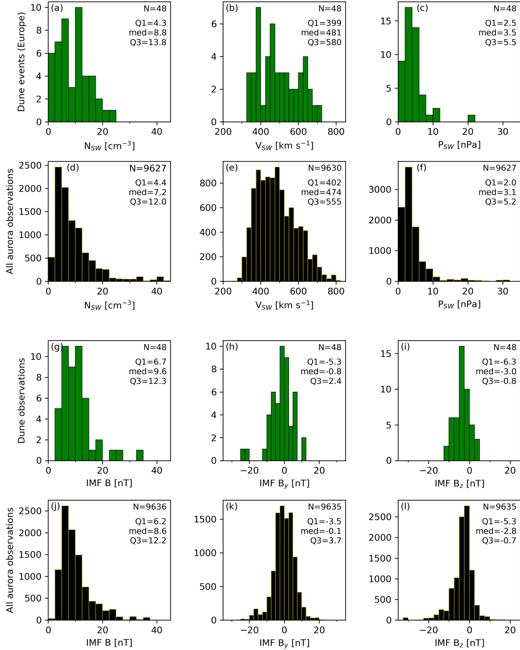
Figure C3. Same as Fig. 5 but considering only the Skywarden reports from the European sector.
