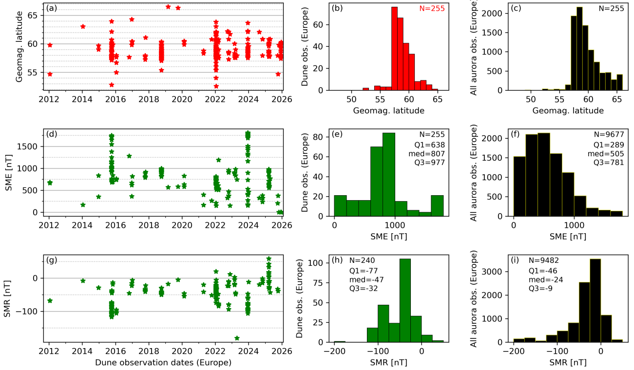
Figure C4. Same as Fig. 6 but considering only the Skywarden reports from the European sector.
