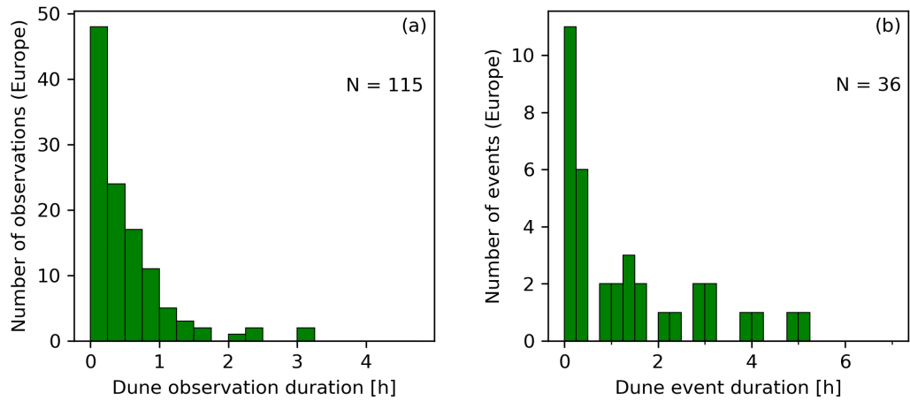
Figure C2. Same as Fig. 4 but considering only the Skywarden reports from the European sector.
