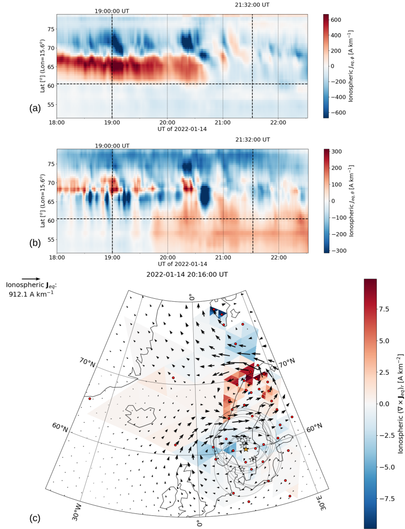
Figure 8. Equivalent current analysis applied to dune observations in the Swedish sector during the 14 January 2022 event. Same format as Fig. 227.
