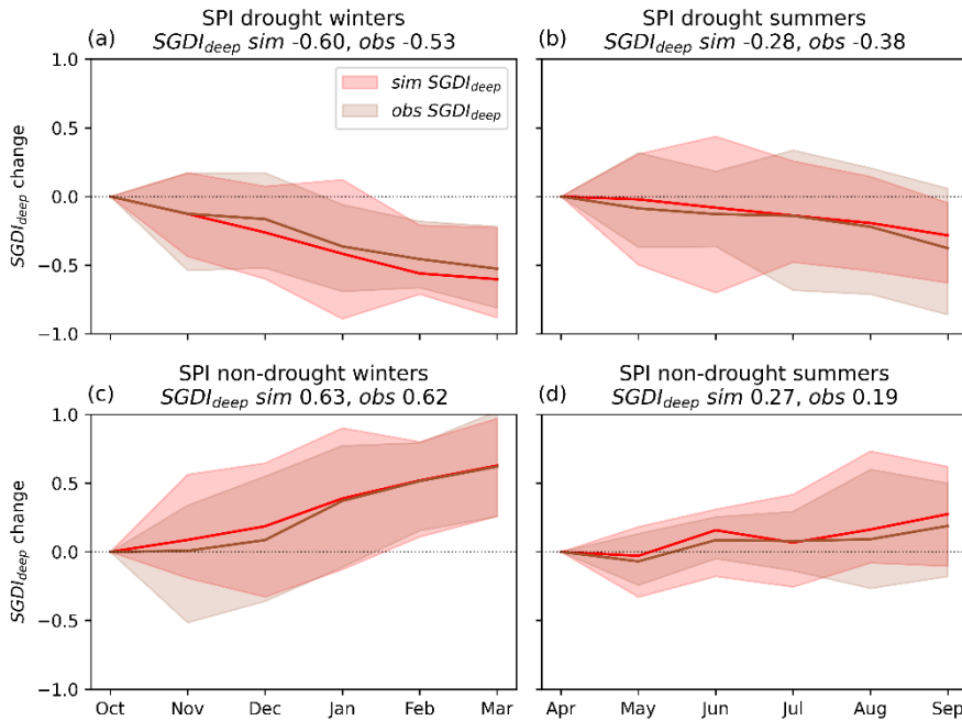
595 Figure 10. Seasonal dependency of deep groundwater ( SGDI_{deep} ) drought response to SPI droughts. (a): Years with drought winters (defined by SPI_{acc6} in March < -0.5 ) and their respective SGDI_{deep} development, normalized to the start of the season (10%/90% intervals shaded, mean as bold line). (b): Years with drought summers ( SPI_{acc6} September < -0.5 ). (c) Years with non-drought winters ( SPI_{acc6} March > 0.5 ). (d) Years with non-drought summers ( SPI_{acc6} September > 0.5 ).
