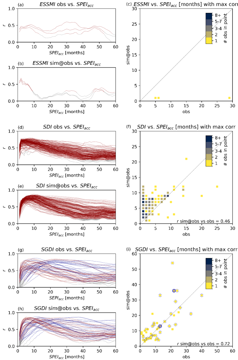
805 Figure C 12: (equivalent to Fig. 5, but using SPEI instead of SPI) Left column: Correlation coefficients of SPEI accumulation 810 periods against observed and simulated time series of ESSMI (a,b), SDI (d,e) and SGDI (g,h), respectively. Significant correlations ( p < 0.01 ) in red (or blue for wells representing SGDI deep ), remaining in grey. Right column: scatter plots of optimal accumulation period of SPEI for correlation to ESSMI at the 3 CRN stations (c), SDI at the 153 streamflow stations (f), and SGDI at the 53 groundwater wells (i), where wells representing SGDI deep are marked with blue outlines (two wells in same point: thick blue outline). Optimal SPEI accumulation period for simulated time series along y-axis, and for observed time series along x-axis.
