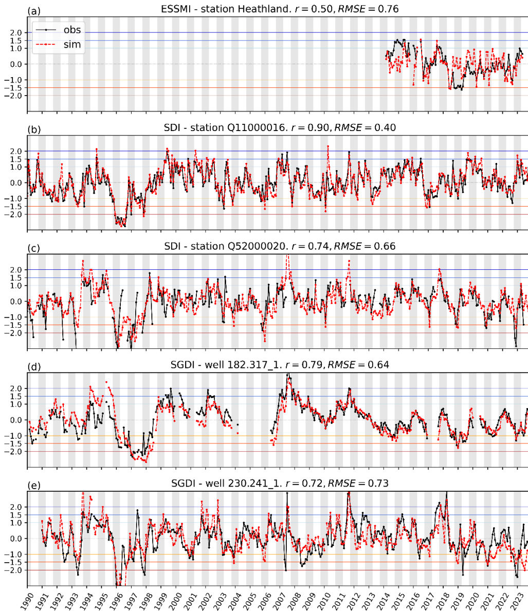
425 Figure 3. Examples of observed drought indices (black), compared to simulated values (red) at example CRN stations (a), streamflow stations (b, c) or wells (d, e). Winter periods (October to March) with grey background. Thresholds for moderate, severe, and extreme droughts (and wet conditions) are marked with horizontal lines.
