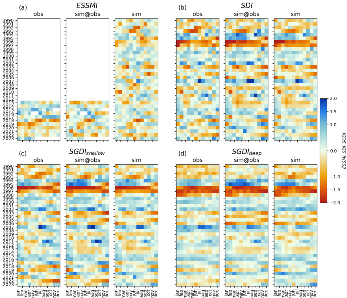
555 Figure 7. Mean monthly drought indices for ESSMI (a), SDI (b), SGDI shallow (c) and SGDI deep (d). Each panel shows from left to right: Mean obs drought indices, mean sim@obs drought indices, mean sim drought indices across all of Denmark.
