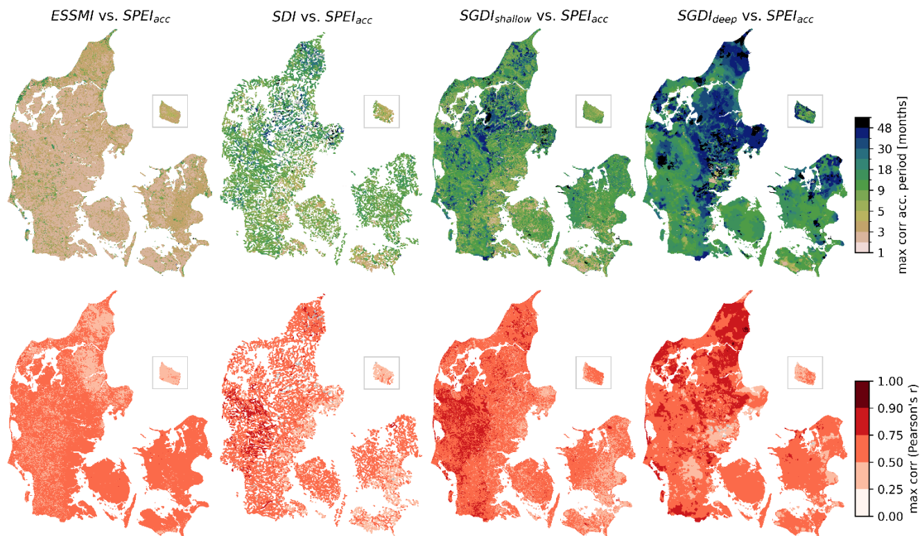
825 | Figure C 45: (equivalent to Figure 6, but using SPEI instead of SPI and only during dry anomalies defined by SPEI < 0 ) Top row: Accumulation period of SPEI_{acc} yielding maximum correlation with hydrological drought index per DK-model q-point or grid. Bottom row: Maximum correlation between hydrologic drought index and SPEI_{acc} of respective accumulation period. Non-significant correlations ( p > 0.01 ) are masked grey (e.g. isolated areas for SDI and SGDI_{deep} in eastern Jutland)
