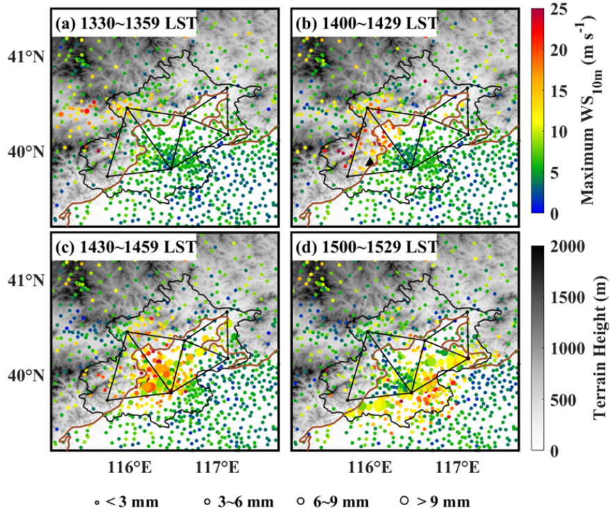
Figure 3. Terrain height (gray shadings; m) over Beijing and surrounding areas superimposed with the maximum 10 m wind speed (shading of dots, m s -1 ) observed during (a) 1330-1359 LST, (b) 1400-1429 LST, (c) 1430-1459 LST, and (d) 1500-1529 LST. The size of dots denoted the accumulated rainfall in 30 minutes. Black small
