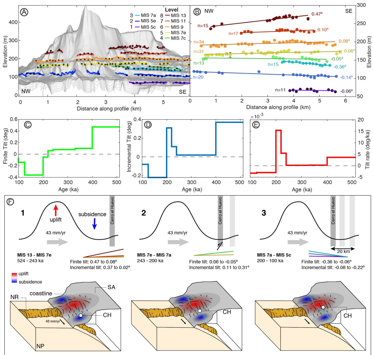
Figure 6: Distribution of shoreline-angle elevations, tilt angles and deformation mechanisms. A) Shoreline-angle mapping overlapping a stacked swath and inner edges. Notice the coherence between inner edge level and shoreline angles. B) Tilt estimates from linear regressions of shoreline angles across marine-terrace levels ( n = number of shoreline angles). C) Finite tilt estimated from linear regressions, representing cumulative deformation. D) Incremental tilt is the difference between successive finite tilts, represents the deformation accumulated between terrace levels. E) Tilt rate calculated as incremental tilt divided by the corresponding time interval. F) Conceptual model using three time slices to explain changes in tilt angles: Slice 1: between MIS 13 and 7e Cerro El Huevo (CH) was located at the margin of the subsiding zone (northward tilt); Slice 2: between MIS 7e and 7a CH was near the hinge between uplift and subsidence (almost no tilt), the short-lived incremental tilt increase is attributed to crustal faults (See text for details); Slice 3: between MIS 7a and MIS 5c CH reached the flank of the uplifting bulge (southward tilt). NR: Nazca Ridge, NP: Nazca plate, SA: South American plate.
