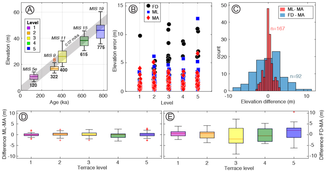
Figure 9: Statistics of different shoreline-angle mapping methods applied along the Sahel Ridge, NE Algeria. A) Shoreline-angle elevations versus marine terrace ages. Age assignments for levels 1-3 follow Authemayou et al. (2017), while the ages of levels 4 and 5 are based on the extrapolation of uplift rate. B) Shoreline-angle elevation errors for each mapped shoreline, note the higher errors for shoreline angles mapped using FABDEM (FD). C) Distributions of elevation differences between manually (MA) and machine-learning (ML) mapped shoreline-angles using ICESat-2 profiles, and between FABDEM and ICESat-2 manual mapping (FD-MA). Notice the higher dispersion of the results based on FABDEM mapping. D) Boxplots showing the difference in elevations between machine-learning and manual mapping both using ICESat-2 profiles. E) Boxplots showing the difference in elevations between FD and MA shoreline angles.
