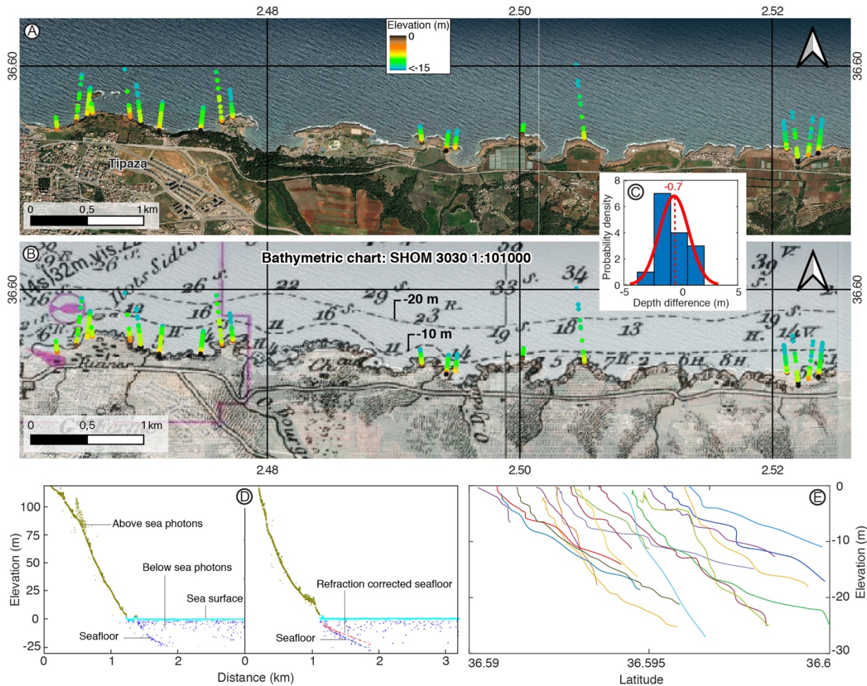
Figure 7: Example application of the TerraceM ICESat-2 bathymetric module at the locality of Tipaza, Algeria. A) Location of the 19 ICESat-2 photon profiles used for bathymetry extraction. B) Bathymetric chart SHOM 3030 used to compare bathymetry estimates. C) Histogram and normal probability distribution of the differences between the 10 m bathymetric contour line and the ICESat bathymetry. The mean difference is 0.7 m. D) Example of automatically classified profiles and the clear delineation of the seafloor, which is afterwards corrected by water diffraction to obtain a bathymetric profile. E) Stacked bathymetric profiles displaying the seafloor morphology and the maximum depth reached by photons. Panel A uses open BING® imagery as background.
