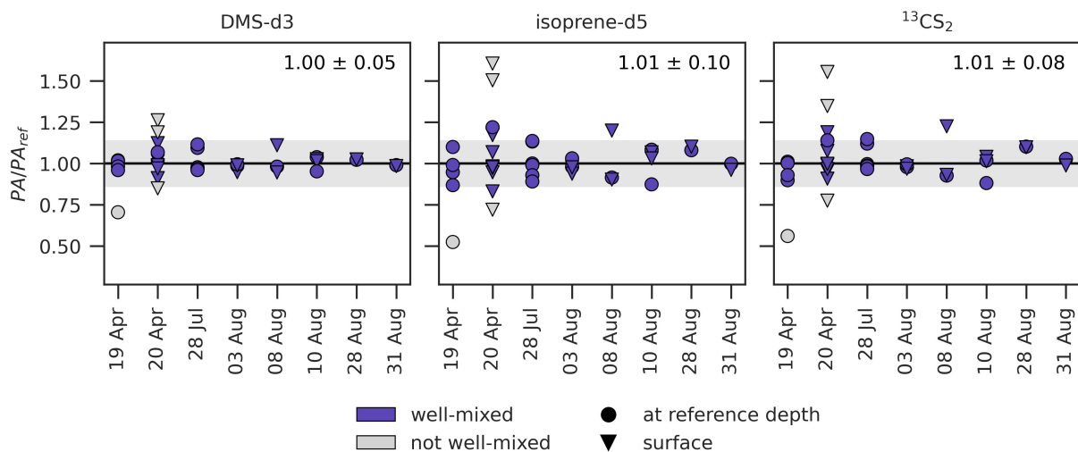
Figure 3 Test for uniform trace gas concentration in the tanks (well-mixed). The ratios PA/PA_{ref} ( n = 37 ) are shown against date for DMS-d3 (left), isoprene-d5 (middle) and ^{13}CS_2 (right). Black horizontal line depicts PA = PA_{ref} (i.e., well-mixed). Grey shaded area indicates \pm 14.1\% uncertainty, calculated by error propagation. Grey points ( n = 4 ) were identified as not well-mixed. Mean and standard deviation for PA/PA_{ref} is indicated in upper right of each subplot (excluding grey points). April samplings belong to experiment B, all other samplings are experiment C. All three treatments (FW, AS, AS with surfactants) are included.
