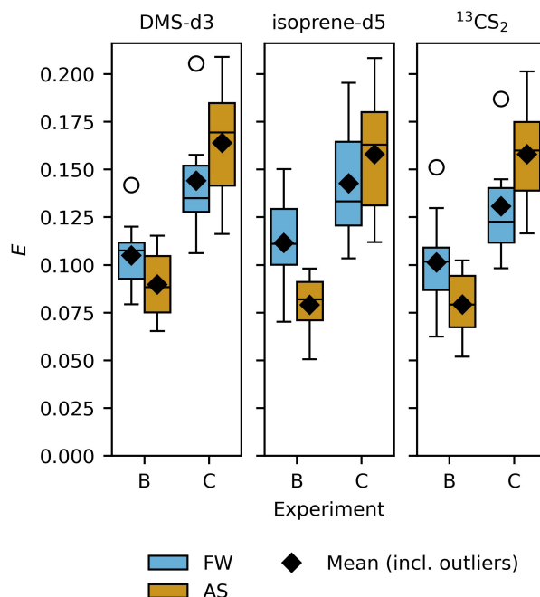
435 Figure 5 Sampling efficiency ( E ) for DMS-d3 (left), isoprene-d5 (middle) and ^{13}\text{CS}_2 (right), separated by experiment, coloured by treatments fresh water (FW, blue) and artificial seawater (AS, orange). Box width shows 25 to 75 percentile, centre line denotes the median, diamonds denote the mean, open circles denote outliers, and whiskers show minimum and maximum. The number of data points in experiment B is n_{FW} = 11 ( n_{FW} = 10 for isoprene-d5) and n_{AS} = 6 , in experiment C n_{FW} = 6 and n_{AS} = 7 .
