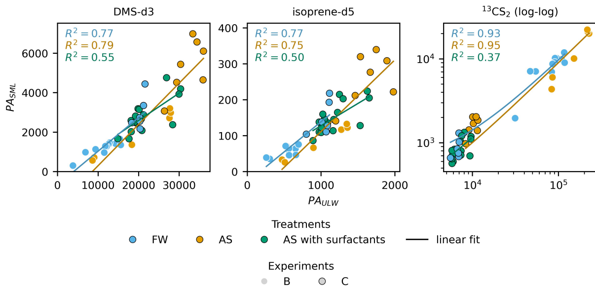
400 Figure 4 Correlation of SML and ULW PA for DMS-d3 (left), isoprene-d5 (middle) and 13 CS 2 (right), grouped by treatments fresh water (FW) and artificial seawater (AS) without and with surfactants. Linear fits for 13 CS 2 were performed on the non-logged data, log-log scale is only used to better visualize the very low values.
