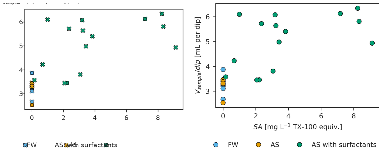
Figure 2 Sample volume collected per dip against SA in experiment C. in experiment C with the glass plate increases with SA.
