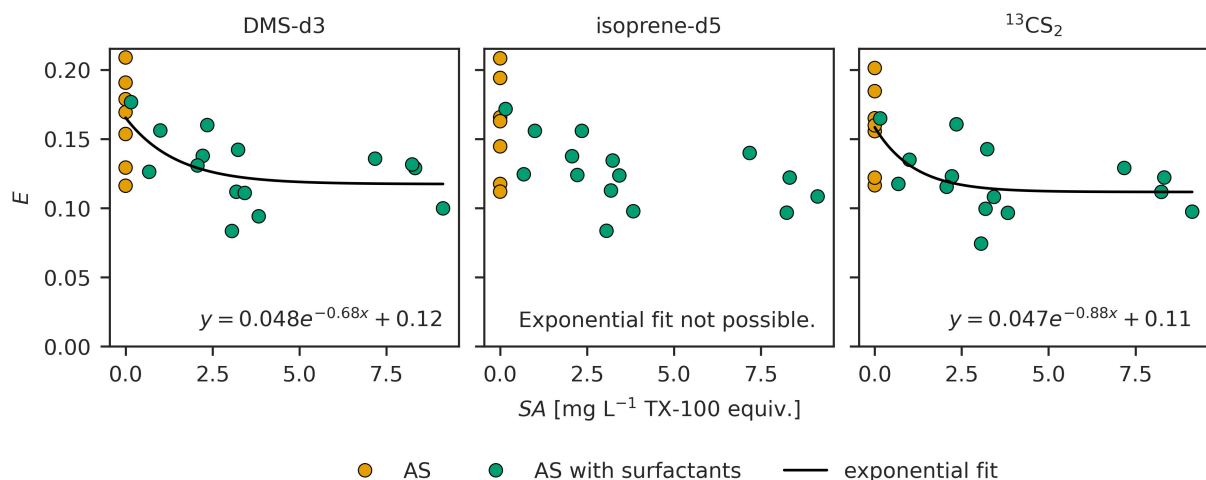
505 Figure 7 Sampling efficiency for DMS-d3 (left), isoprene-d5 (middle) and ^{13}\text{CS}_2 (right) against surface activity (SA) in experiment C. Exponential fit is added as aid for visualization.
