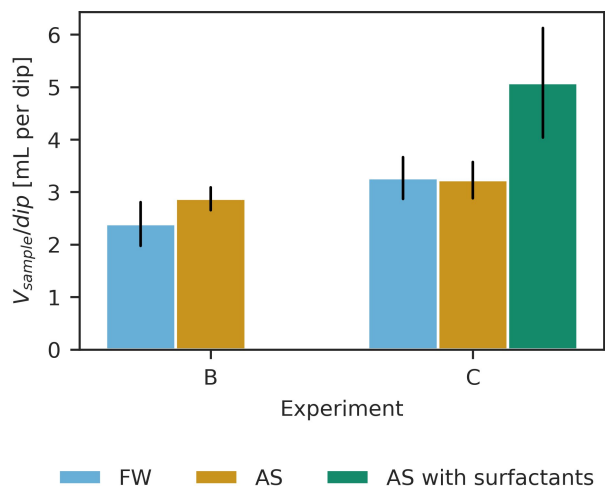
Figure 1 Collected sample volume V_{sample} for SML samples per dip of the glass plate in the three treatments. Black lines indicate standard deviation.
