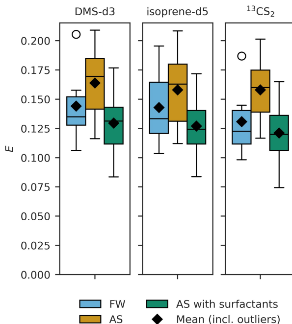
Figure 6 Sampling efficiency for DMS-d3 (left), isoprene-d5 (middle) and ^{13}\text{CS}_2 (right) when artificial surfactants are added to artificial seawater (AS with surfactants) from experiment C ( S_p = 31.1 \pm 2.9 ). Fresh water (FW) and artificial seawater without surfactants (AS) are depicted as well for reference. Box width shows 25 to 75 percentile, centre line denotes the median, diamonds denote the mean, open circles denote outliers, and whiskers show minimum and maximum. The number of data points is n_{FW} = 6 , n_{AS} = 7 and n_{SA} = 16 .
