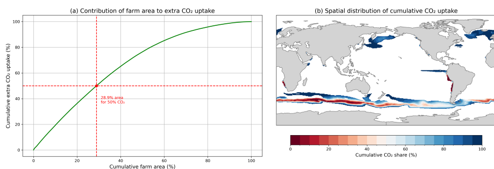
Figure 7. Large variation in CO 2 uptake within macroalgal cultivation areas. (a) Model grid cells are sorted by their quantitative contributions to additional CO 2 uptake and then the associated cultivation area and CO 2 uptake are accumulated. (b) Geographical distribution of cultivation area which contributes the most to additional CO 2 . Deep red regions are those that contribute most to CO 2 uptake, while deep blue regions contribute least.
