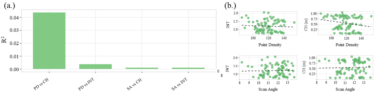
865 Figure B4. Panel (a) summarizes the coefficients of determination ( R^2 ) between point density (PD), scan angle (SA), LiDAR crop height (CH), and normalized LiDAR intensity (INT). Panel (b) presents the corresponding scatter plots for PD versus INT, PD versus CH, SA versus INT, and SA versus CH. The weak relationships observed for both CH and normalized INT indicate that the selected acquisition parameters (double-grid flight pattern, 50% overlap, and maximum scan angle of 25°) effectively minimized the influence of scan angle and point density on these LiDAR features used for above-ground biomass estimation.
