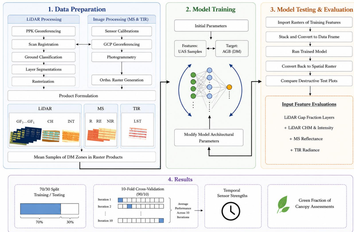
185 Figure 4: Overview of the methodological framework used for UAV-based aboveground biomass (AGB) estimation. UAV-derived LiDAR, multispectral (MS), and thermal infrared (TIR) observations were processed into standardized structural, spectral, and thermal feature sets and evaluated using a common artificial neural network (ANN) framework with repeated stratified cross- validation. A tiered feature addition strategy was employed, beginning with LiDAR multi-layer gap fraction (GF) and progressively incorporating crop height (CH), normalized LiDAR intensity (INT), multispectral reflectance, and thermal observations to 190 systematically assess the complementary contribution of individual sensor features and multi-sensor combinations for winter wheat AGB estimation.
