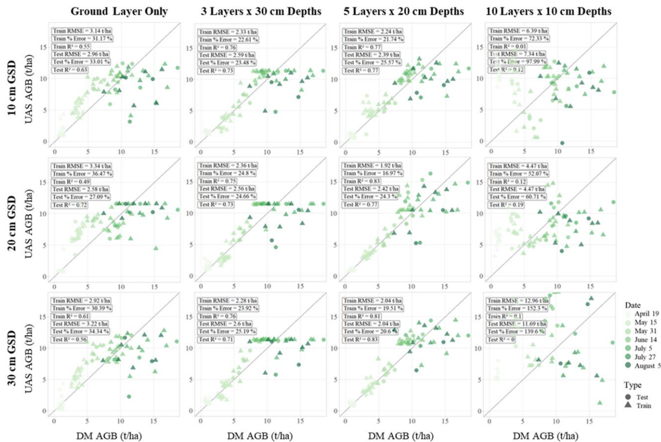
880 Figure B6. Observed versus predicted above-ground biomass (AGB) for ANN models trained using different LiDAR gap fraction (GF) parameterizations. Columns represent increasing vertical segmentation, ranging from the conventional ground-based gap fraction (GF GND ) to 3 × 30 cm, 5 × 20 cm, and 10 × 10 cm multi-layer GF configurations, while rows represent decreasing horizontal ground sampling distance (GSD) from 30 cm to 20 cm and 10 cm. Marker color indicates acquisition date and marker shape distinguishes training and testing samples. Training and testing RMSE, relative error, and R 2 are reported within each panel. The 885 5 × 20 cm GF configuration with a 30 cm GSD achieved the best overall balance between model accuracy and generalization, whereas the finest 10 × 10 cm segmentation exhibited substantially reduced testing performance, indicating increased sensitivity to sparse point distributions and model overfitting.
