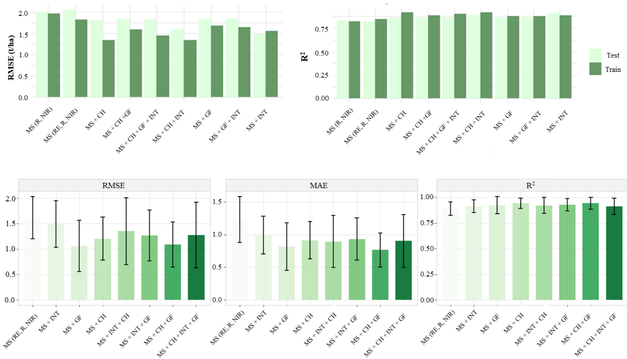
420 Figure 10. Biomass estimation performance using multispectral (MS) reflectance individually and in combination with LiDAR- derived crop height (CH), 5 layer gap fraction (GF), and normalized intensity (INT). The 5 layer GF configuration corresponds to the optimal parameterization identified in Figure 7 (20 cm layer depth; 30 cm GSD). Top: 70/30 holdout training and testing performance. Bottom: Repeated stratified 10-fold cross-validation showing mean RMSE, MAE, and R² with error bars representing variability among folds.
