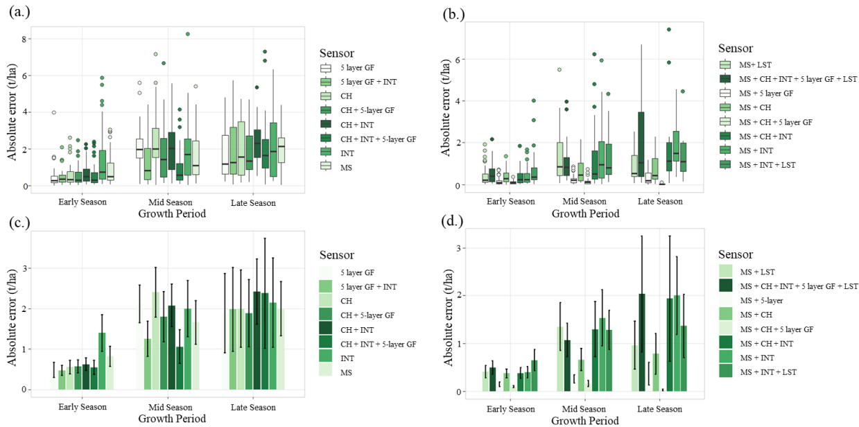
930 Figure B10. The left panels show the best-performing single-sensor feature combinations, while the right panels show the best-performing multi-sensor fusion models. The top panels present the distribution of absolute prediction errors (t ha -1 ) as boxplots, and the bottom panels summarize the corresponding mean absolute prediction errors ( \pm SD) for each growth period. Growth periods were defined as early season (19 April–31 May), mid-season (14 June–5 July), and late season (27 July–5 August). These results complement the analyses presented in the main manuscript by illustrating the magnitude and variability of biomass prediction errors throughout crop development and across the evaluated sensor configurations. 935
