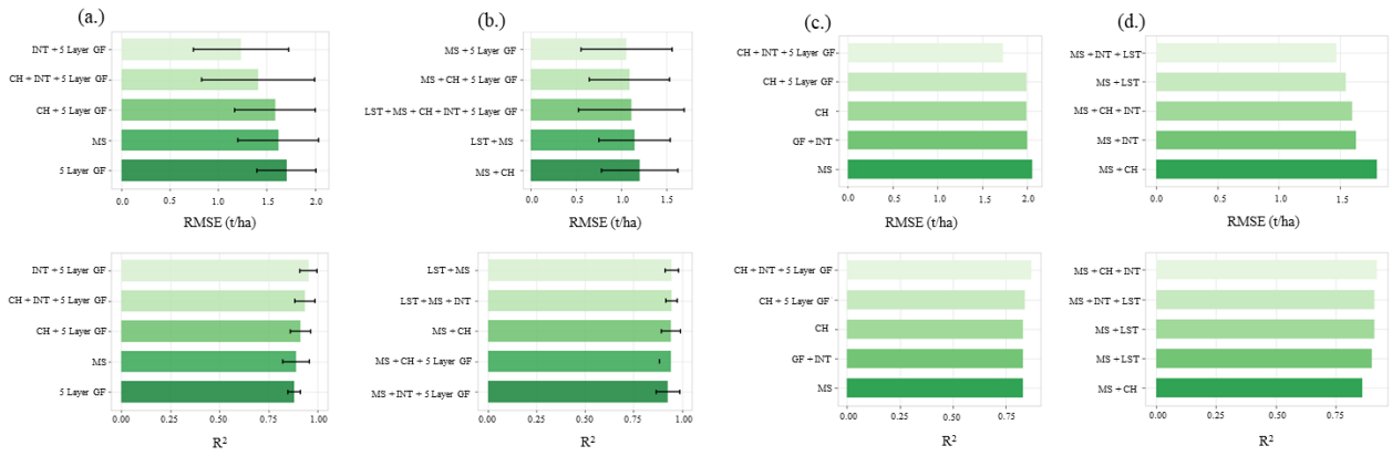
Figure 12. Ranking of the five best-performing single-sensor and multi-sensor feature combinations based on the 70/30 holdout evaluation (left) and repeated stratified 10-fold cross-validation (right). Rankings are shown separately for RMSE and R^2 . Error bars represent variability among cross-validation folds where applicable. LiDAR-derived features consistently dominate the single-sensor rankings, while several complementary LiDAR–multispectral–thermal combinations achieve similarly high performance in the multi-sensor comparison.
