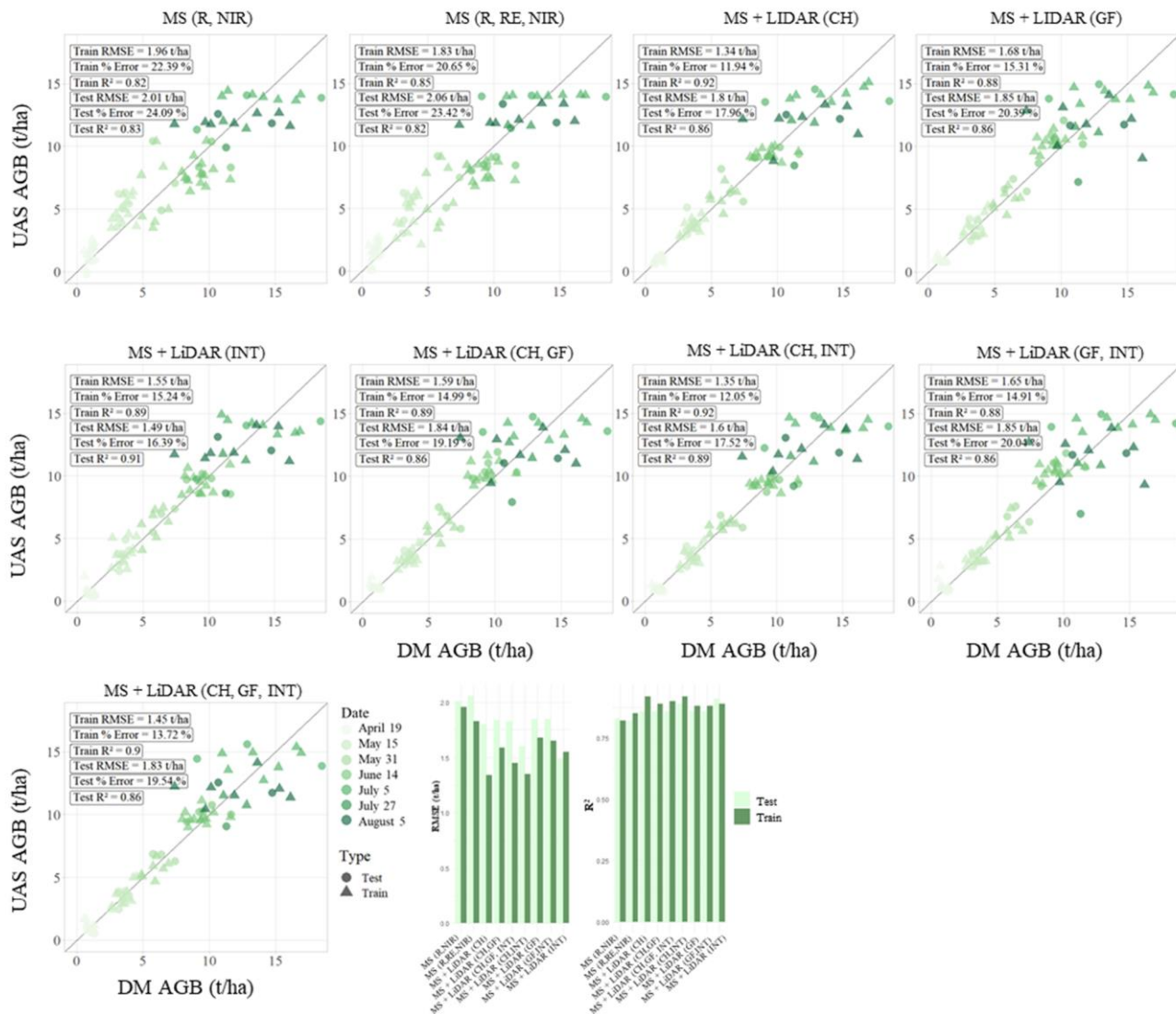
900 Figure B8. Observed versus predicted above-ground biomass (AGB) for ANN models using multispectral (MS) reflectance (Red, Red-edge, and Near-Infrared (NIR)) individually and in combination with LiDAR-derived crop height (CH), five-layer multi-layer gap fraction (GF; 20 cm layer depth), and field-normalized LiDAR intensity (INT). All models were generated using the optimal 30 cm ground sampling distance (GSD) identified in the GF sensitivity analysis. Marker color indicates acquisition date and marker shape distinguishes training and testing samples. Training and testing RMSE, relative error, and R2 are reported within each panel. 905 The accompanying summary plots compare testing RMSE and R2 across the evaluated feature combinations, illustrating the improvement achieved by integrating multispectral reflectance with complementary LiDAR-derived structural and normalized intensity information.
