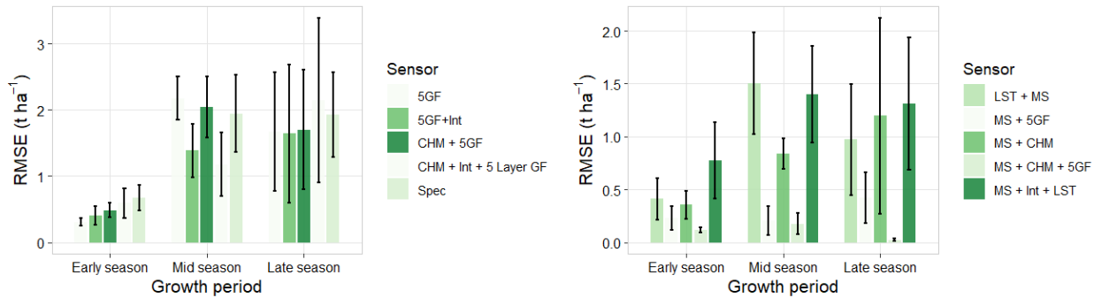
Figure 13: Growth-stage evaluation of the best-performing sensor configurations using repeated stratified 10-fold cross-validation. Left: Top five single-sensor feature combinations. Right: Top five multi-sensor feature combinations. Early season corresponds to April 19–May 31, mid season to June 14–July 5, and late season to July 27–August 5. Error bars represent variability among cross-validation folds and illustrate the increasing uncertainty associated with later developmental stages.
