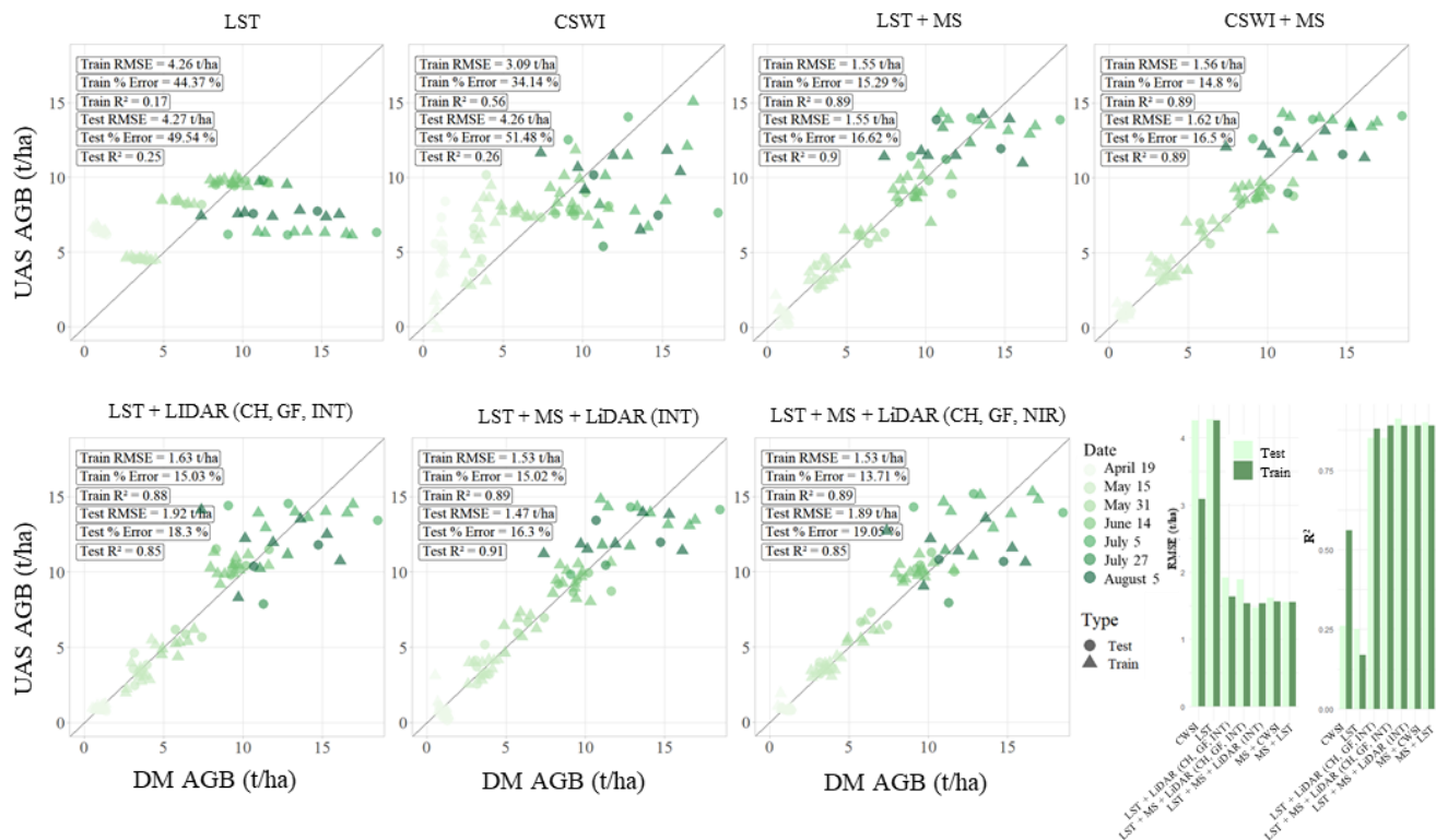
880 Figure B9. Observed versus predicted above-ground biomass (AGB) for ANN models using thermal infrared (TIR) features, including land surface temperature (LST) and the Crop Water Stress Index (CWSI), individually and in combination with multispectral (MS; Red, Red-edge, and Near-Infrared (NIR)) reflectance and LiDAR-derived canopy height (CH), five-layer multi-layer gap fraction (GF; 20 cm layer depth), and normalized LiDAR intensity (INT). All models were generated using the optimal 30 cm ground sampling distance (GSD) identified in the GF sensitivity analysis. Marker color indicates acquisition date and marker shape distinguishes training and testing samples. Training and testing RMSE, relative error, and R2 are reported within each panel. The accompanying summary plots compare testing RMSE and R2 across the evaluated feature combinations, illustrating the limited predictive capability of TIR features alone and their complementary contribution when integrated with multispectral reflectance and LiDAR-derived structural information
