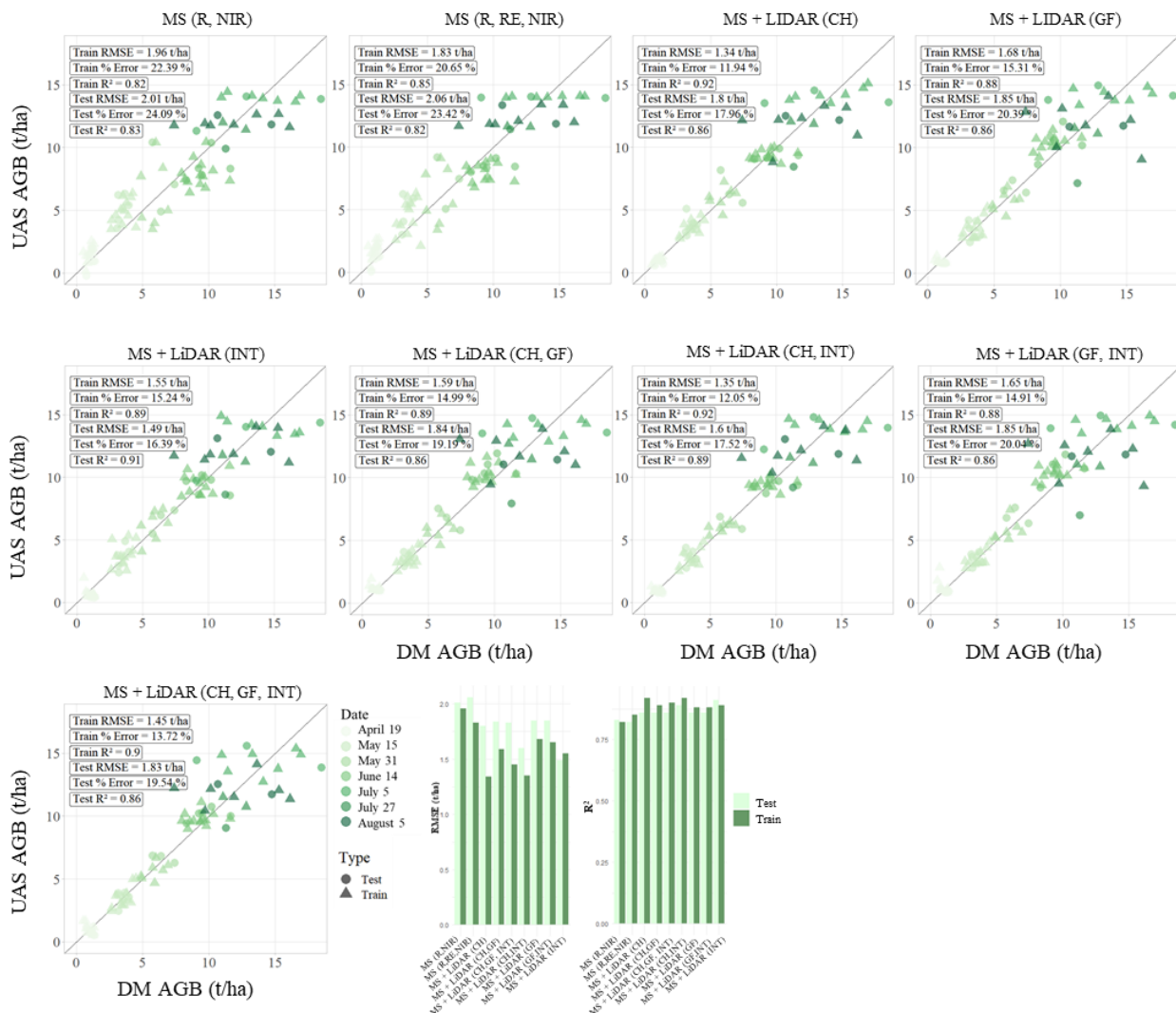
870 Figure B8. Observed versus predicted above-ground biomass (AGB) for ANN models using multispectral (MS) reflectance (Red, Red-edge, and Near-Infrared (NIR)) individually and in combination with LiDAR-derived canopy height (CH), five-layer multi-layer gap fraction (GF; 20 cm layer depth), and field-normalized LiDAR intensity (INT). All models were generated using the optimal 30 cm ground sampling distance (GSD) identified in the GF sensitivity analysis. Marker color indicates acquisition date and marker shape distinguishes training and testing samples. Training and testing RMSE, relative error, and R2 are reported within 875 each panel. The accompanying summary plots compare testing RMSE and R2 across the evaluated feature combinations, illustrating the improvement achieved by integrating multispectral reflectance with complementary LiDAR-derived structural and normalized intensity information.
