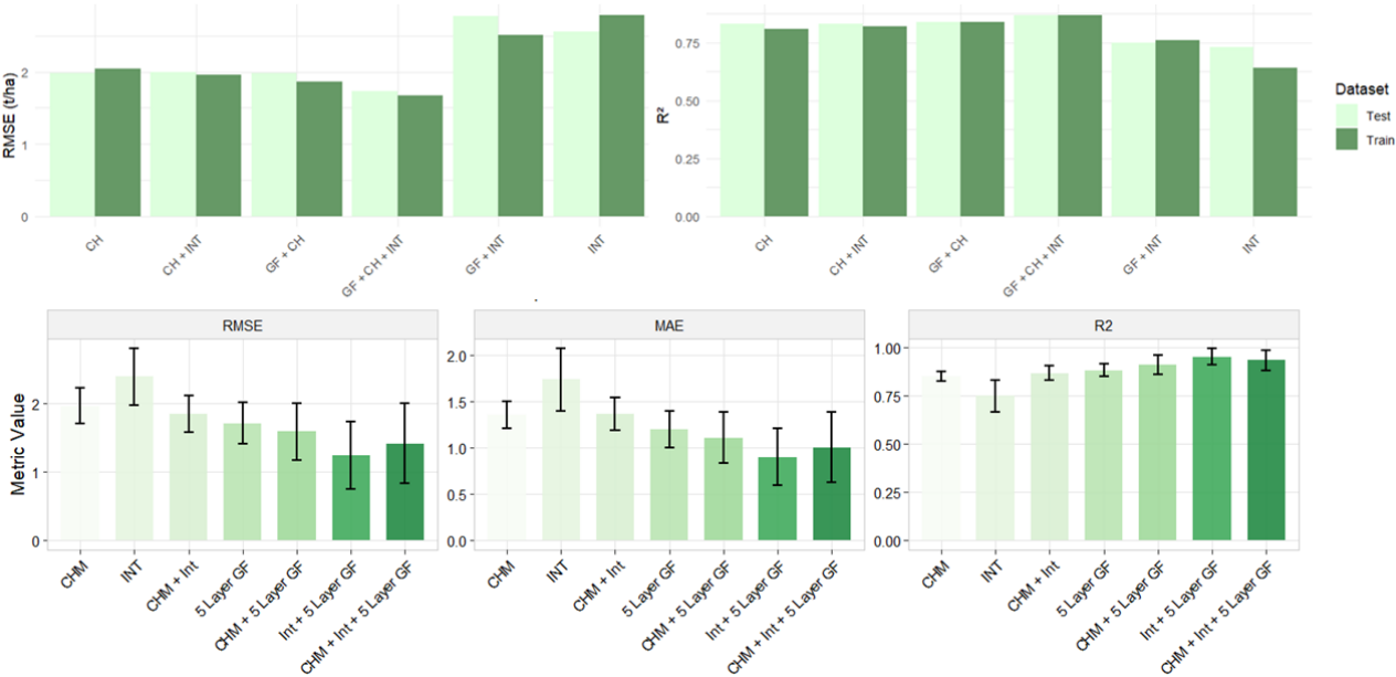
Figure 9. Performance of LiDAR-derived feature combinations for AGB estimation using the optimal 5 layer gap fraction (GF) parameterization (20 cm layer depth; 30 cm GSD). Canopy height (CH), normalized intensity (INT), and five-layer GF were evaluated individually and in combination. (a) Results from the 70/30 training–testing holdout evaluation showing training (dark green) and testing (light green) RMSE and R² values. (b) Results from repeated stratified 10-fold cross-validation, showing mean RMSE, MAE, and R² with error bars representing variability among folds.
