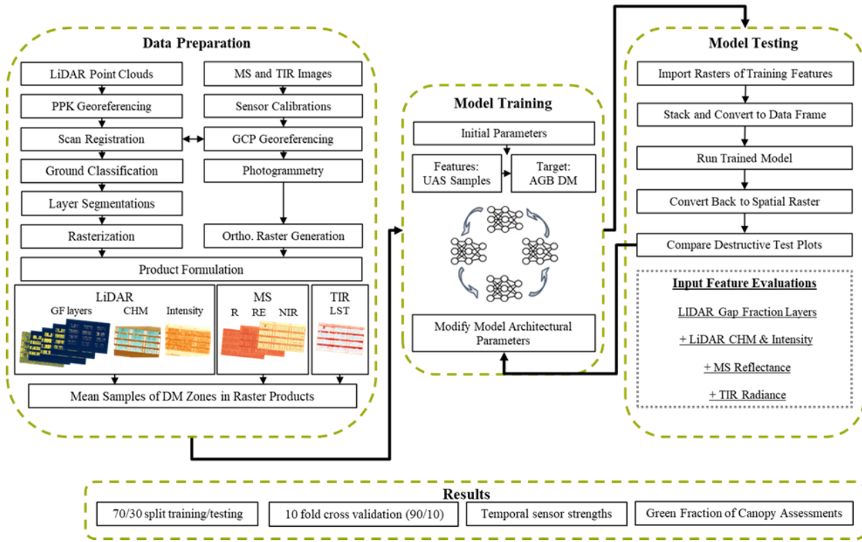
Figure 4: Overview of the methodological framework used for UAV-based aboveground biomass (AGB) estimation. UAV-derived LiDAR, multispectral (MS), and thermal infrared (TIR) observations were processed into standardized structural, spectral, and thermal feature sets and evaluated using a common artificial neural network (ANN) framework with repeated stratified cross-validation. A tiered feature addition strategy was employed, beginning with LiDAR multi-layer gap fraction (GF) and progressively incorporating canopy height (CH), normalized LiDAR intensity (INT), multispectral reflectance, and thermal observations to systematically assess the complementary contribution of individual sensor features and multi-sensor combinations for winter wheat AGB estimation.
