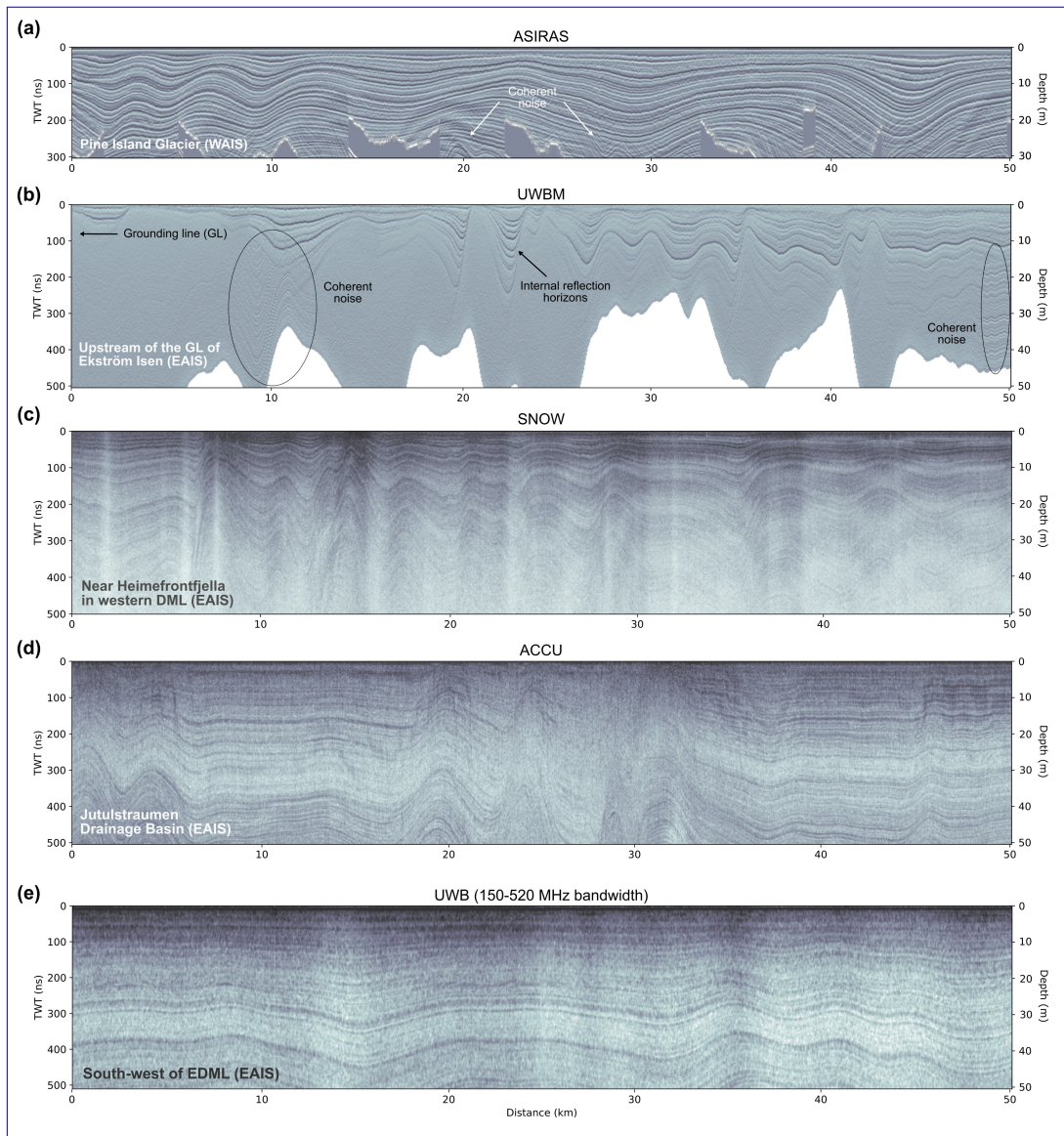
Figure 4. Examples of radargrams focusing on the first 50m depth below the surface. (a) ASIRAS; profile ID: ASR_L1B_01_20141203T130418_132058, (b) UWBM; profile ID: UWBM_20221205_99_[019-021]019-021 ], (c) SNOW; profile ID: SNOW_20140102T074743_081922, (d) ACCU; profile ID: ACCU_20131230T090855_094516, (e) UWB in wideband mode; profile ID: Data_20231211_02_006_standard . For TWT-to-depth (two-way travel time) conversion we used an average electromagnetic wave speed in the upper 50 m of 2 \cdot 10^9 \text{ m s}^{-1} , which corresponds to an average ordinary relative dielectric permittivity \epsilon'_r of 2.25. The location of the radar profile is annotated in the lower left corner of the radargram and shown in Figure 3 . All radargrams are time-zeroed at the ice surface reflection.
