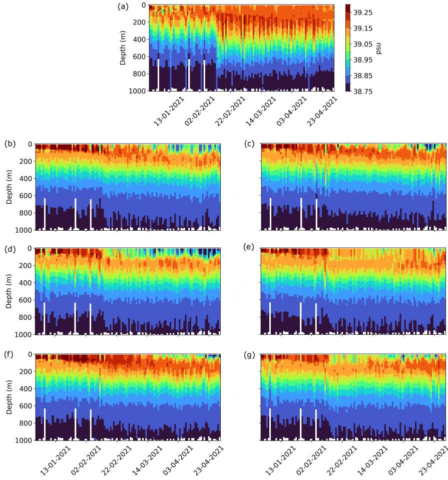
660 Figure 11: (a) Hovmöller diagram of salinity observations from available Argo floats in the Rhodes Gyre region (Fig. 1a) between January and April 2021. (b–g) Hovmöller diagrams of salinity for different vertical mixing schemes and convective adjustment settings: (b) Richardson-dependent mixing scheme with EVD activated, and (c) without EVD activated; (d) TKE closure scheme with EVD activated, and (e) without EVD activated; (f) GLS scheme with EVD activated, and (g) without EVD activated. All panels share the colour scale in panel (a).
