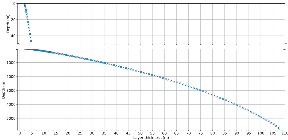
Figure 2: Vertical layer thickness as a function of depth. A zoom of the upper 50 m highlights the fine vertical discretization within the mixed layer.
