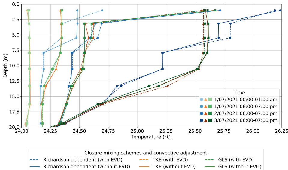
735 Figure 13: Temperature profiles at a site (27.5°E, 34.4°N) in the Rhodes Gyre region at different times of the day (see legend in the inset) and for different closure schemes and convective adjustment settings (see bottom legend).
