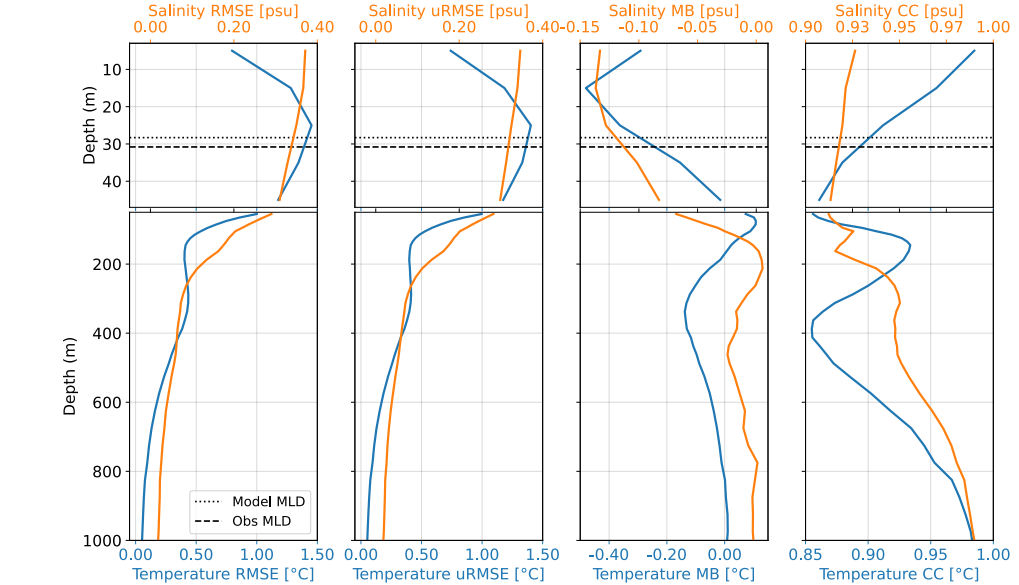
Figure 5: Basin-averaged temperature (blue) and salinity (orange) error profiles for 2020–2021 in the control simulation (Exp-PP+ in Table 1). Panels from left to right: root mean squared error (RMSE), unbiased root mean squared error (uRMSE), mean bias (MB), and cross-correlation coefficient (CC). The definitions of these metrics are in Appendix C. Dashed lines represent the two-year basin average values of the MLD for observations and control simulation.
