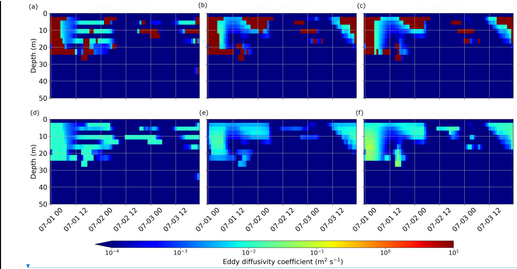
Figure 12: Hovmöller diagrams of the hourly eddy diffusivity coefficient between 1 and 3 July 2021 (upper 50 m) for the six simulations with (a) Richardson-number dependent scheme with EVD, (b) TKE with EVD, (c) GLS with EVD, (d) Richardson-number dependent scheme without EVD, (e) TKE without EVD, (f) GLS without EVD.
