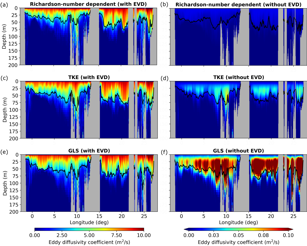
355 Figure 3: Vertical eddy diffusivity coefficient along the zonal section at 37.5°N (black line in Fig. 1a) averaged over January 2021 for different model configurations: (a) Richardson-dependent mixing scheme with EVD activated, and (b) without EVD activated; (c) TKE closure scheme with EVD activated, and (d) without EVD activated; (e) GLS scheme with EVD activated, and (f) without EVD activated. The black contours in each panel denote the depth of the mixed layer, while grey shading indicates land. Note the different eddy diffusivity scales for the experiments with and without EVD.
