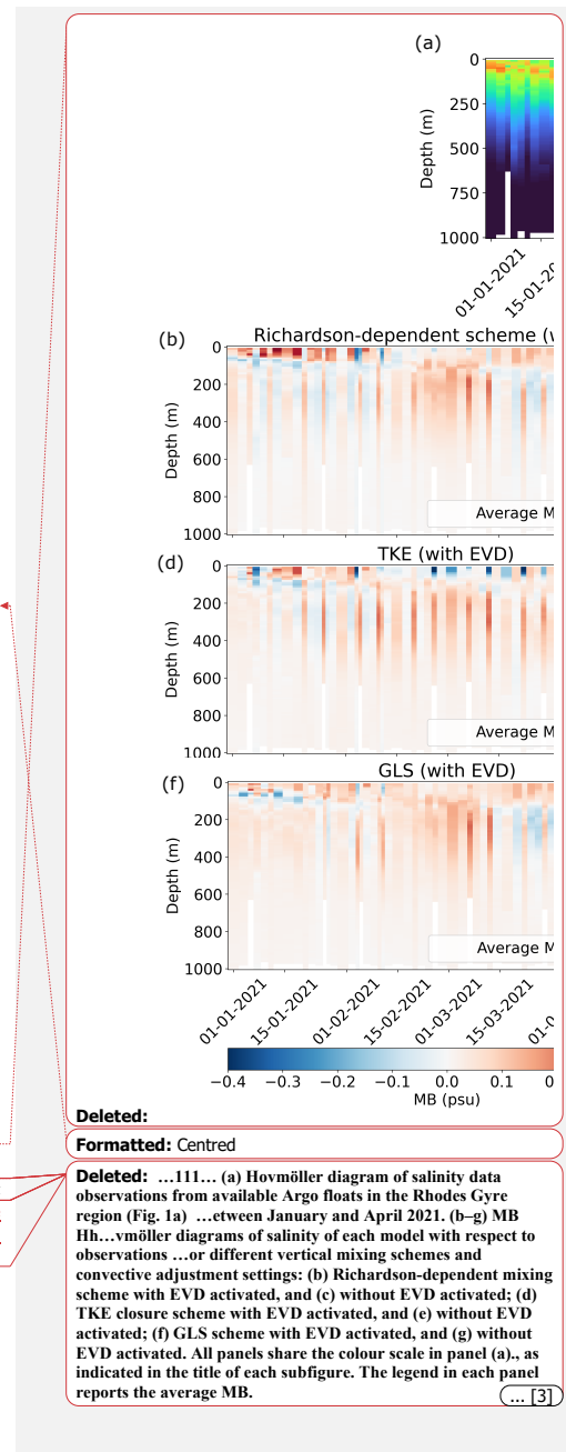
Figure 11: (a) Hovmöller diagram of salinity observations from available Argo floats in the Rhodes Gyre region (Fig. 1a) between January and April 2021. (b–g) Hovmöller diagrams of salinity for different vertical mixing schemes and convective adjustment settings: (b) Richardson-dependent mixing scheme with EVD activated, and (c) without EVD activated; (d) TKE closure scheme with EVD activated, and (e) without EVD activated; (f) GLS scheme with EVD activated, and (g) without EVD activated. All panels share the colour scale in panel (a).
