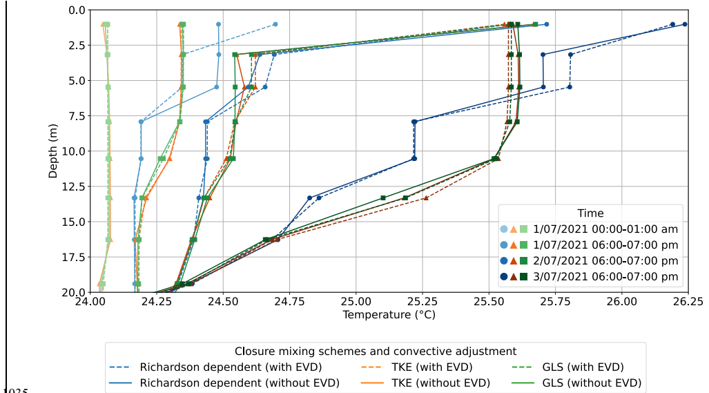
Figure 13: Temperature profiles at a site (27.5°E, 34.4°N) in the Rhodes Gyre region at different times of the day (see legend in the inset) and for different closure schemes and convective adjustment settings (see bottom legend).
