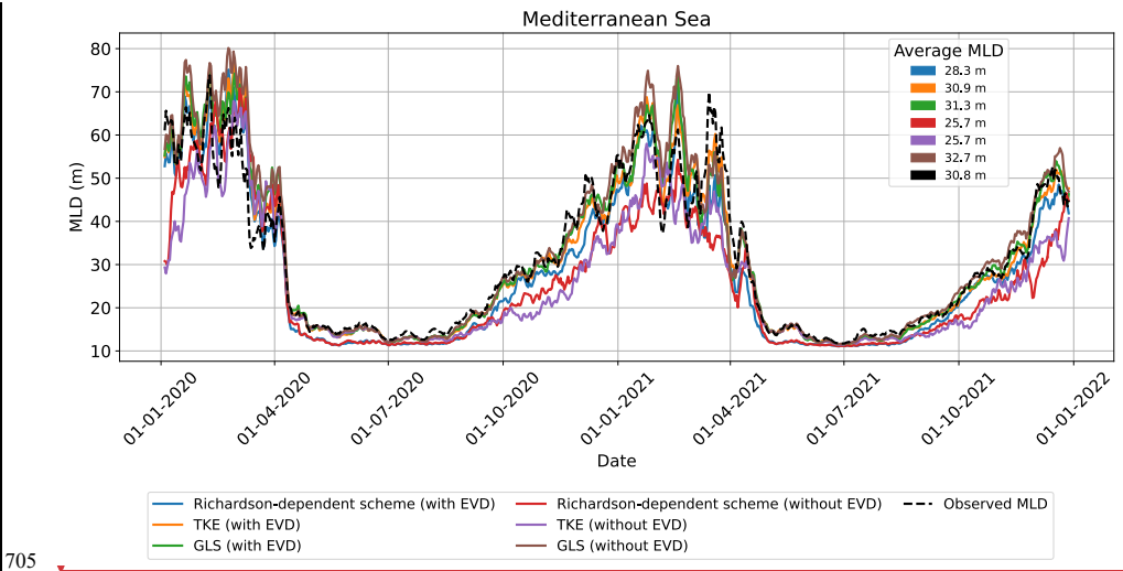
705 Figure 8: Time evolution of basin-averaged MLD for varying vertical mixing schemes, with and without convection parameterisation (configurations listed in Table 1). The black dashed line represents the MLD from Argo observations. A 7-day moving average has been applied to both model outputs and observations.
