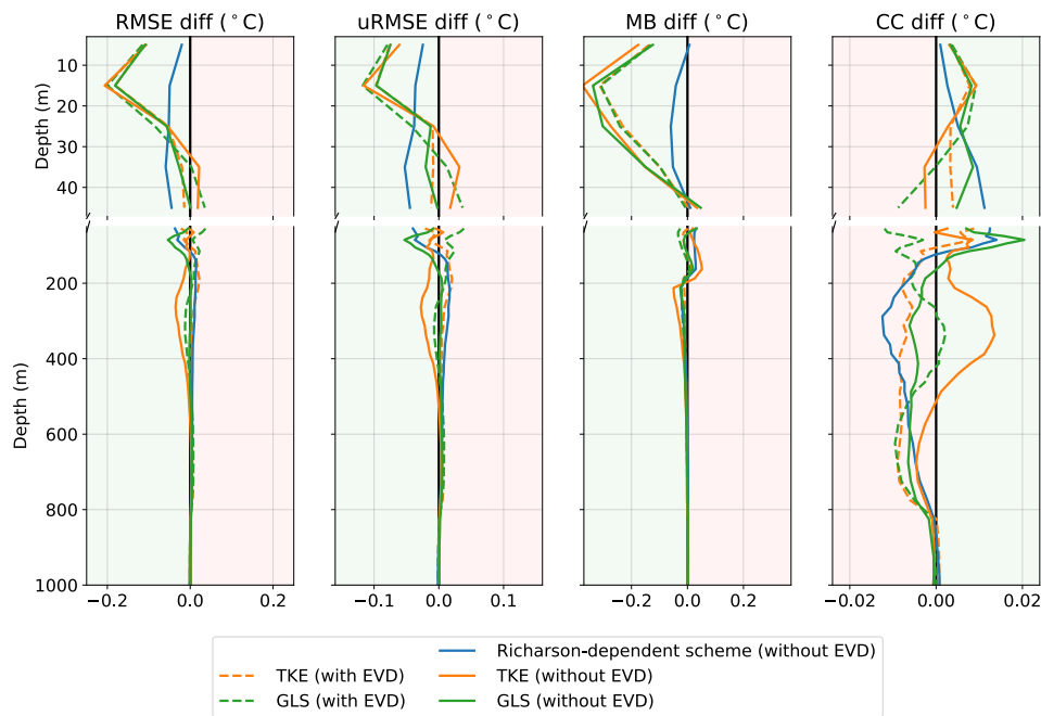
Figure 6: Temperature error difference (equation 1) with respect to the control simulation for the four metrics in equations C1–C4. Dashed lines indicate simulations with EVD and continuous lines without EVD. The transparent background color highlights regions of improvement (green) and worsening (red) compared to the control simulation.
