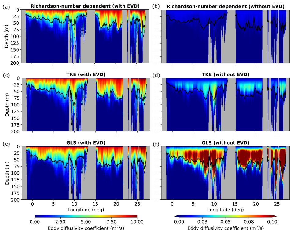
Figure 3: Vertical eddy diffusivity coefficient along the zonal section at 37.5°N (black line in Fig. 1a) averaged over January 2021 for different model configurations: (a) Richardson-dependent mixing scheme with EVD activated, and (b) without EVD activated; (c) TKE closure scheme with EVD activated, and (d) without EVD activated; (e) GLS scheme with EVD activated, and (f) without EVD activated. The black contours in each panel denote the depth of the mixed layer, while grey shading indicates land. Note the different eddy diffusivity scales for the experiments with and without EVD.
