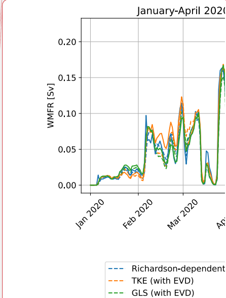
Deleted: Figure 10: Daily water mass formation rate in the south Adriatic Pit. Curves are colour-coded by different vertical mixing schemes, with and without convective adjustment as indicated in the legend.
