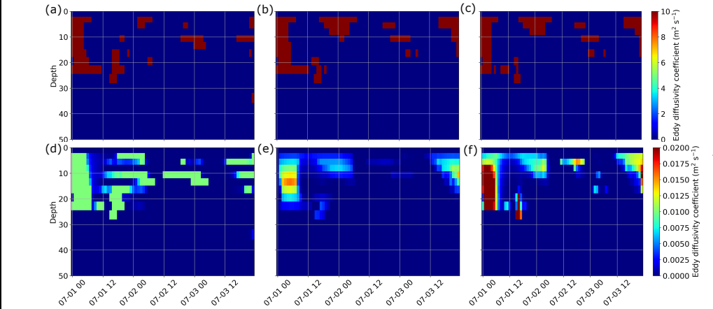
Figure 12: Hovmöller diagrams of the hourly eddy diffusivity coefficient between 1 and 3 July 2021 (upper 50 m) for the six simulations with (a) Richardson-number dependent scheme with EVD, (b) TKE with EVD, (c) GLS with EVD, (d) Richardson-number dependent scheme without EVD, (e) TKE without EVD, (f) GLS without EVD.
