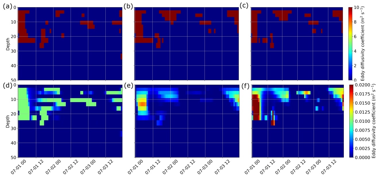
Figure 12: Hovmöller diagrams of the hourly eddy diffusivity coefficient between 1 and 3 July 2021 (upper 50 m) for the six simulations with (a) Richardson-number dependent scheme with EVD, (b) TKE with EVD, (c) GLS with EVD, (d) Richardson-number dependent scheme without EVD, (e) TKE without EVD, (f) GLS without EVD.
