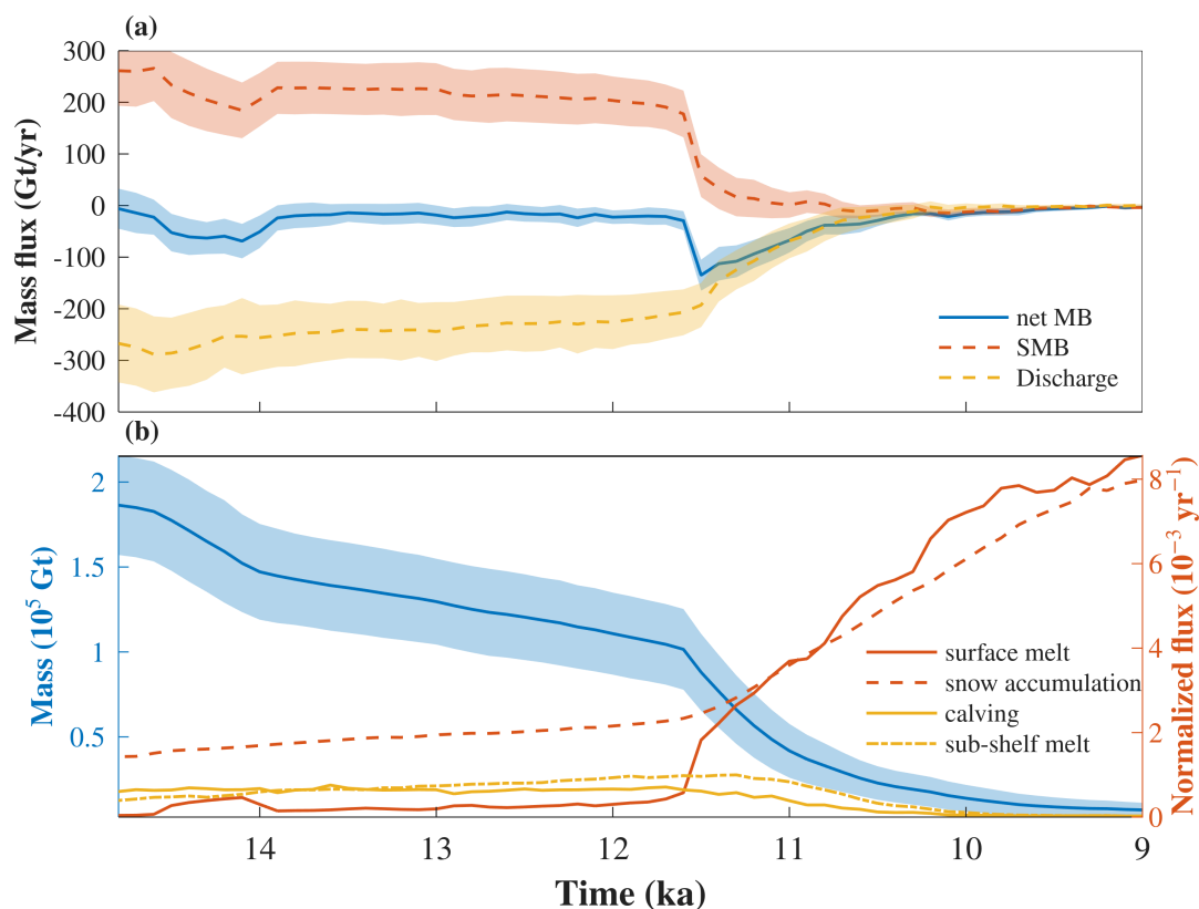
Figure A10. Mass balance components (output) of the IIS from 15 to 9 ka for experiments without hydrofracturing. (a) Mass balance components of grounded ice including net mass balance (blue), surface mass balance (SMB, orange dashed), and ice discharge at the grounding line (yellow dashed), with shading indicating uncertainty ( \pm 1\sigma ). (b) Total ice mass (blue, left axis) and mass fluxes normalized by the ice sheet total mass (right axis).
