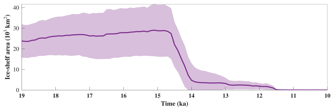
Figure A8. Time series of the ice shelf area during the last deglaciation for the \text{NROY}_{\text{tier1}} subset. The line represents the means and the shaded area the 2\sigma range.
