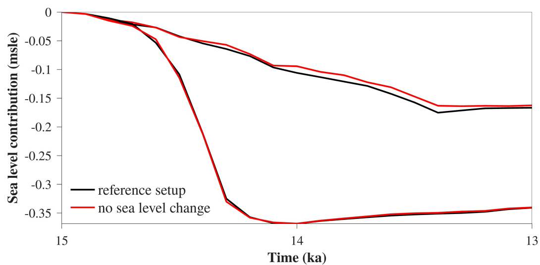
Figure A12. Sea level contribution relative to 15 ka from experiments with sea level change (black) and without sea level change (red) for 2 NROY tier1 parameter vectors (run identification number nn1131, and nn1395, the latter showing the strongest sensitivity in the ensemble).
