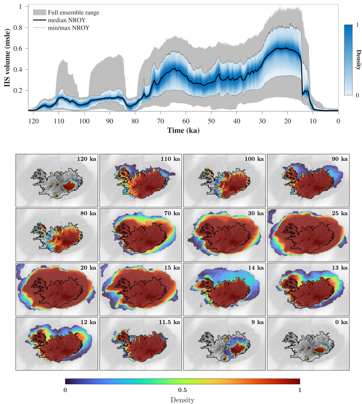
Figure 6. (a) Time series of IIS volume during the last glacial cycle. Initial full ensemble (gray shaded area) and sieved non-ruled out yet ( NROY_{tier1} ) sub-ensemble (blue distribution) with median NROY_{tier1} (black curve). (b) Density distribution of grounded ice within the NROY_{tier1} sub-ensemble at different time slices.
