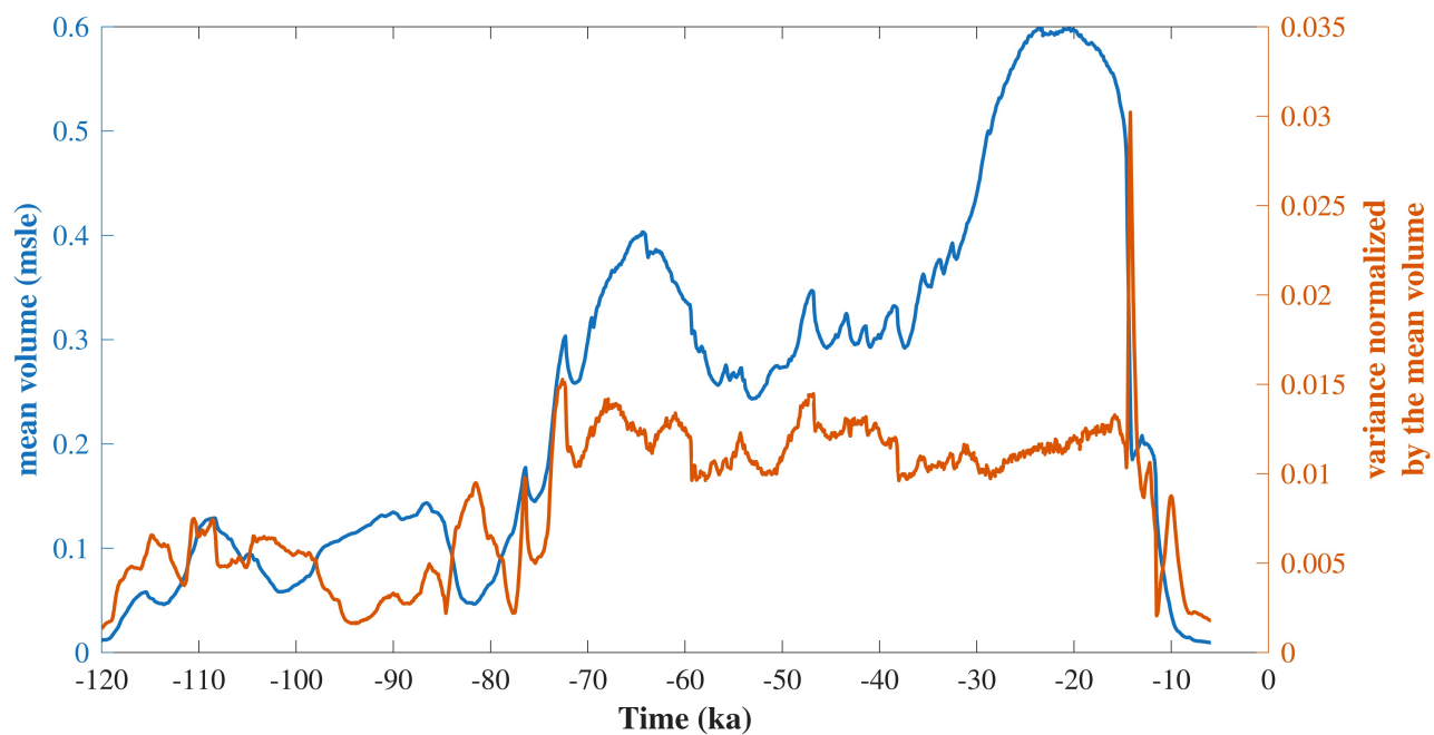
Figure A4. Time series of IIS mean volume (left axis) and variance normalized by the mean volume (right axis) during the last glacial cycle for the \text{NROY}_{\text{tier1}} subset.
