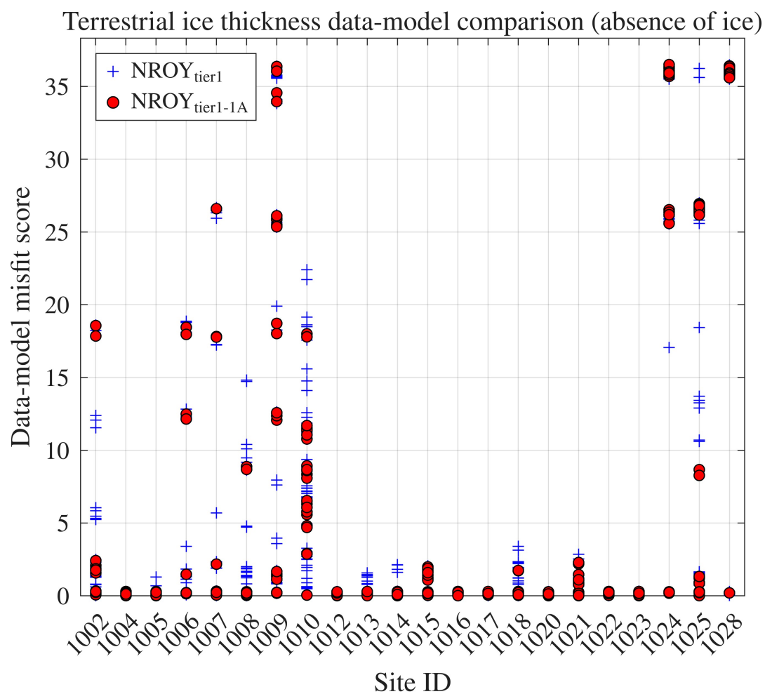
Figure A2. Past ice thickness misfit scores (absence of ice). The data ID locations are shown in Fig. A1.
