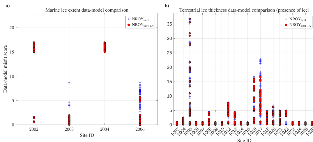
Figure 5. Past ice extent (a) and past ice thickness (b) misfit scores. The data ID locations are shown in Fig. A1.
