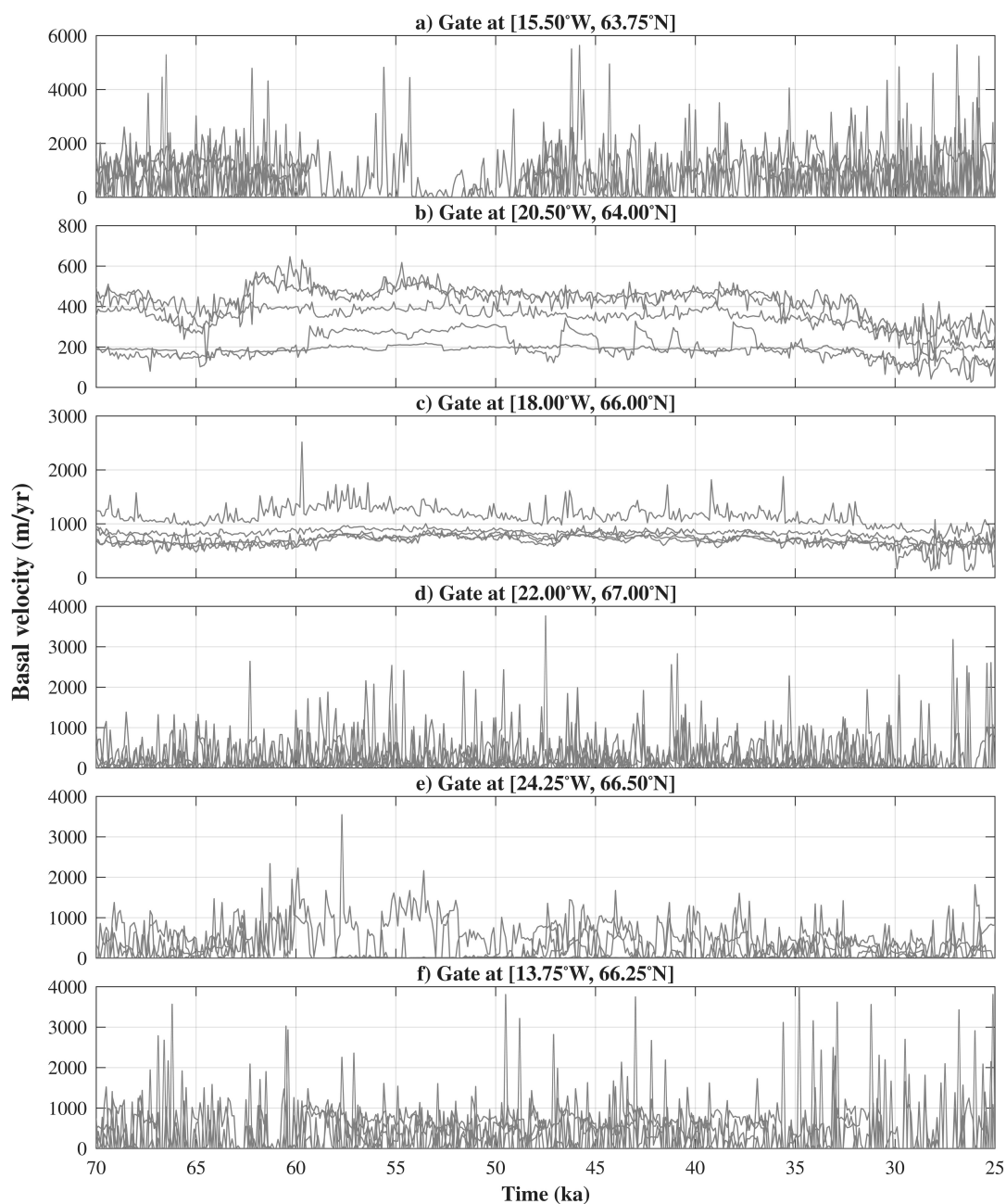
Figure A5. Basal velocity at six ice stream gates of the IIS for 5 NROY tier1 runs.
