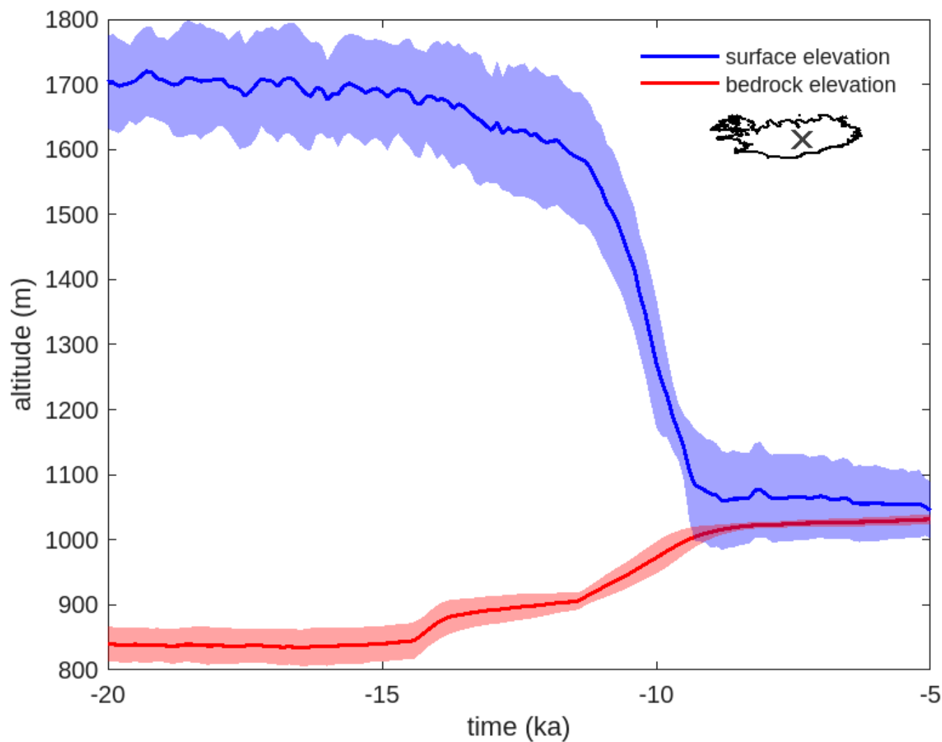
Figure A9. Surface and bedrock elevation at the center of the IIS for the NROY tier1 subset. The lines represent the means and the shaded areas the 2\sigma range.
