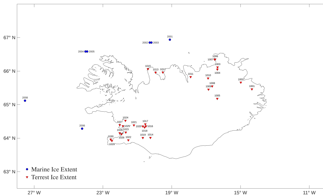
Figure A1. Iceland observational constraint database with site locations and identification numbers for past ice thickness data (paleoH), and past ice extent data (paleoExt).
