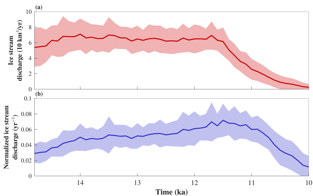
Figure A11. Ice stream discharge (a) and ice stream discharge normalized by the ice sheet volume (b) of the tested subset without hydrofracturing. The lines represent the means and the shaded areas the 2\sigma range. Ice stream discharge was calculated over gates placed within bathymetric troughs and valleys.
