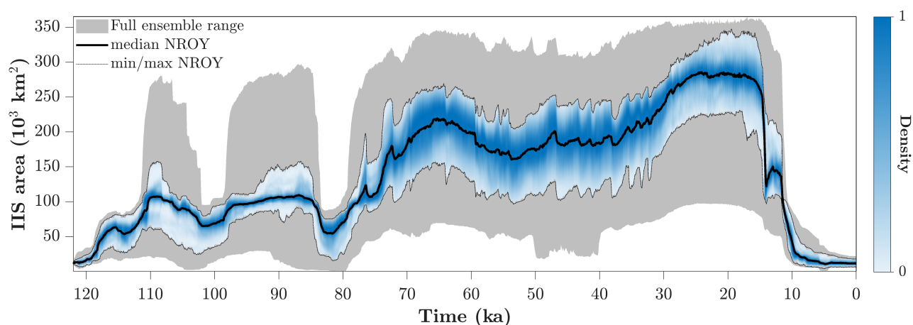
Figure A3. Time series of IIS area during the last glacial cycle. Initial full ensemble (gray shaded area) and sieved non-ruled out yet ( \text{NROY}_{\text{tier1}} ) sub-ensemble (blue distribution) with median \text{NROY}_{\text{tier1}} (black curve).
