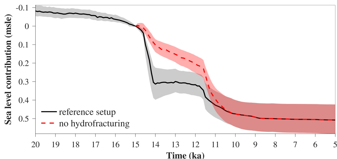
Figure 11. Sea level contribution relative to 15 ka from experiments with hydrofracturing (black) and without hydrofracturing (red), based on the 107 \text{NROY}_{\text{tier1}} parameter vectors. The lines represent the medians and the shaded areas show the 2\sigma ranges.
