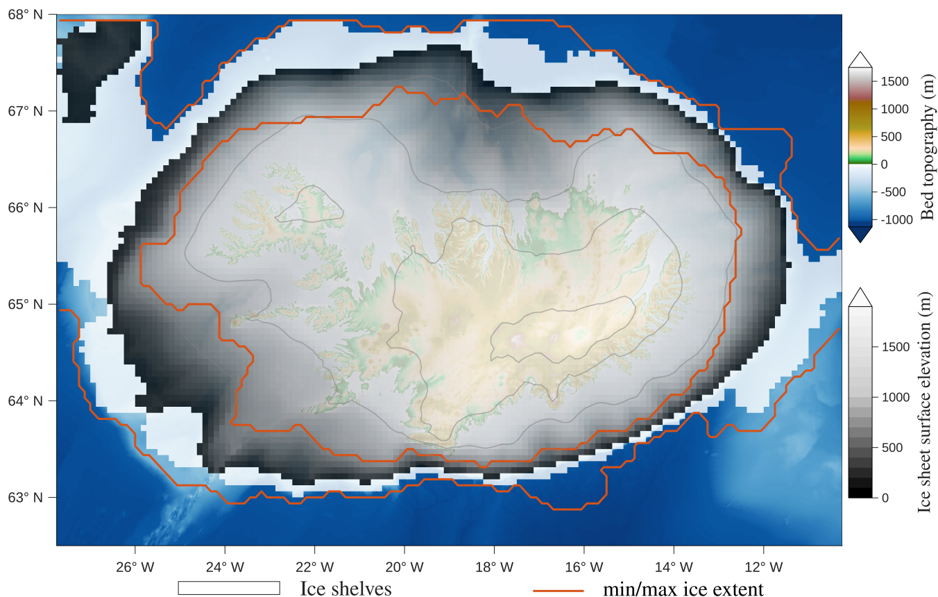
Figure 7. Ice sheet surface elevation (gray shadings) and bedrock elevation (colour shadings) of the mean NROY tier1 at 20 ka. Ice surface-height contours are delineated at 450 m intervals, revealing the double-dome configuration. Indicated ice shelf extent (white filled area) was determined from the ensemble-mean ice shelf geometry, excluding grid cells where mean ice thickness was < 25 m. The minimum and maximum NROY tier1 ice (grounded + floating) extent are shown in orange.
