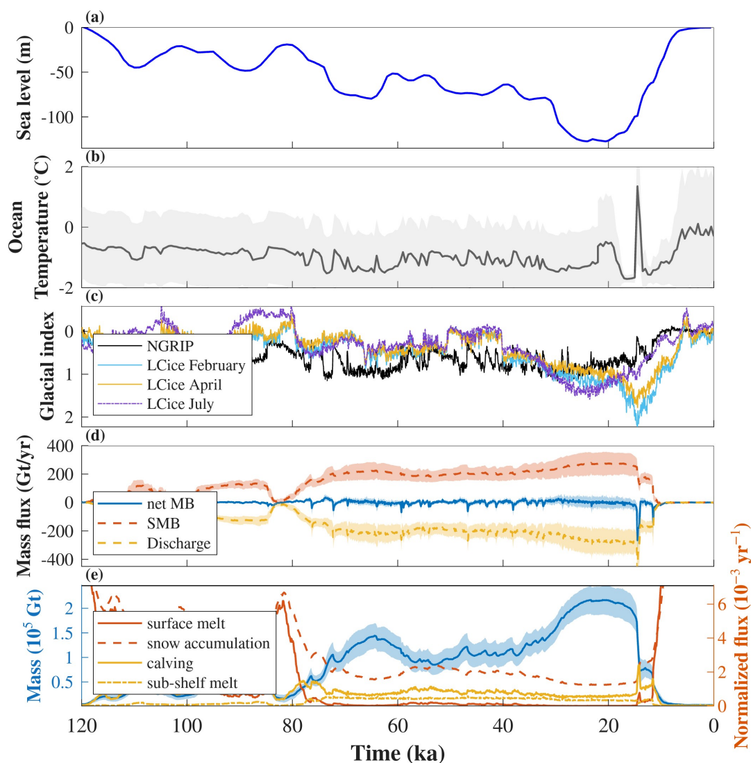
Figure A7. Climate forcing (input) and mass balance components (output) of the IIS over the last glacial cycle (120-0 ka) for the NROY tier1 subset. (a) Global mean eustatic sea level reconstruction. (b) Ocean temperature at 191 m depth from TraCE-21ka deglacial simulation (Liu et al., 2009), with the gray shading indicating uncertainty ( \pm 1\sigma ) around the mean (gray line). (c) Glacial indices derived from smoothed temperature anomalies (50 years running mean, interpolated to 50 year time steps) from the NGRIP ice core (nor, 2004) and seasonal variations from the LCice model (Geng et al., 2025) (February, April, and July). (d) Mass balance components of grounded ice including net mass balance (blue), surface mass balance (SMB, orange dashed), and ice discharge at the grounding line (yellow dashed), with shading indicating uncertainty ( \pm 1\sigma ). (e) Total ice mass (blue, left axis) and normalized mass fluxes (right axis) including surface melt, snow accumulation, calving, and sub-shelf melt.
