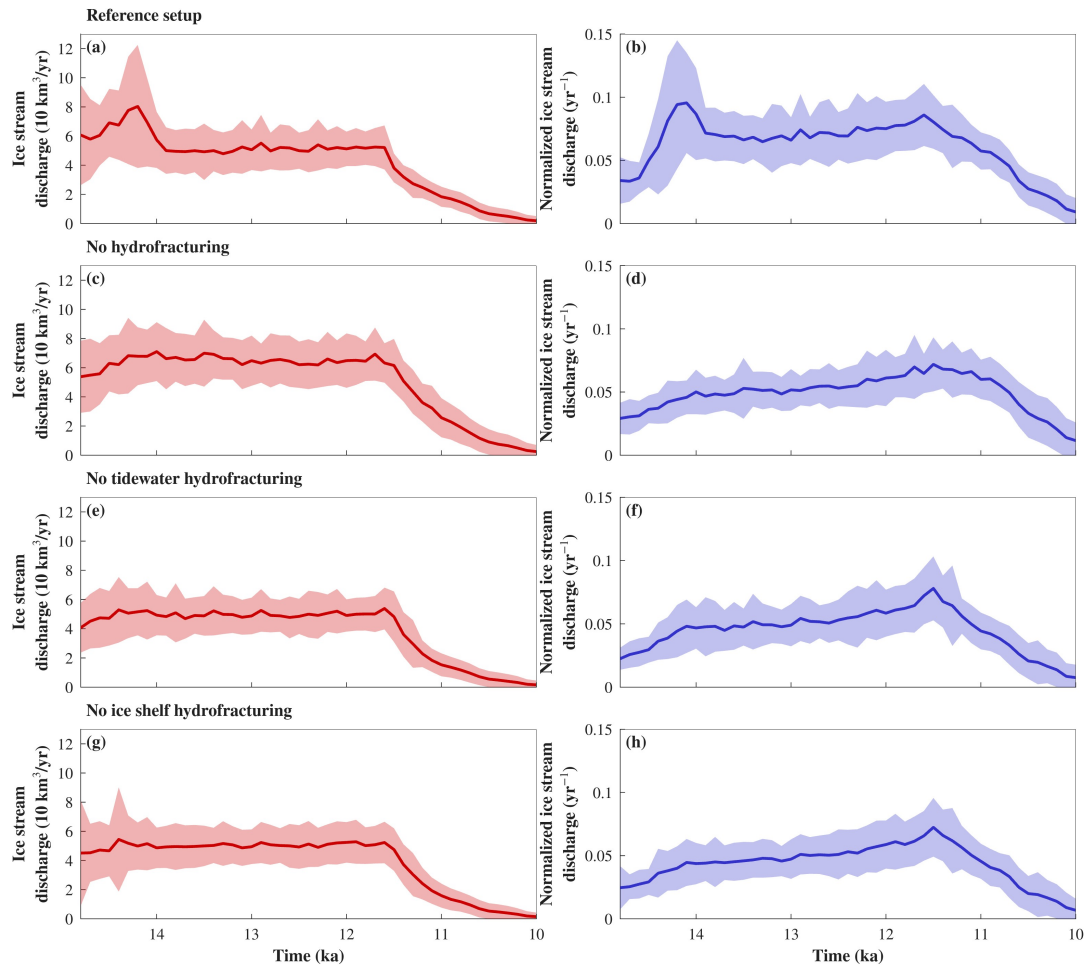
Figure A14. Ice stream discharge (left column) and ice stream discharge normalized by the ice sheet volume (right column) for the different tested subensembles. The rows correspond to the NROY_{\text{tir1}} reference setup (a, b), no hydrofracturing (c, d), no tidewater hydrofracturing (e, f), and no ice shelf hydrofracturing (g, h). The lines represent the means and the shaded areas the 2\sigma range. Ice stream discharge was calculated over gates placed within bathymetric troughs and valleys.
