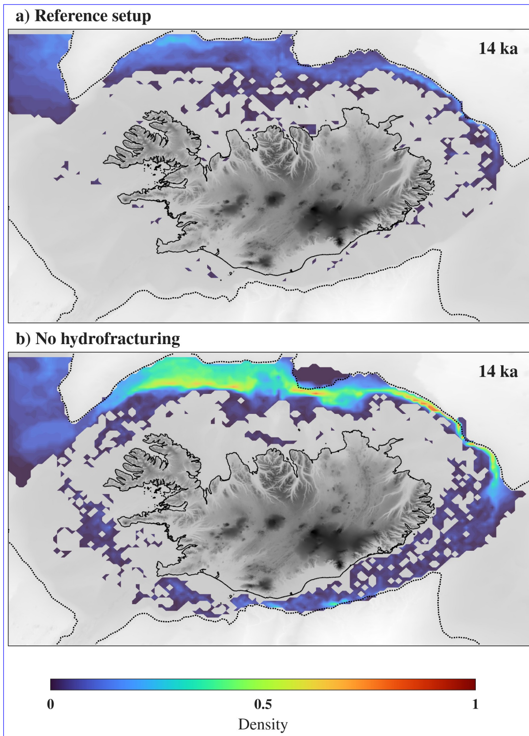
Figure A13. Ice stream discharge Density distribution of floating ice for the NROY tier1 sub-ensemble (a) and ice stream discharge normalized by the ice sheet volume for experiments without hydrofracturing (b) of the tested subset without hydrofracturing at 14 ka. The lines represent the means and the shaded areas -860 m contour is represented by the 2 \sigma range. Ice stream discharge was calculated over gates placed within bathymetric troughs and valleys black dotted line.
