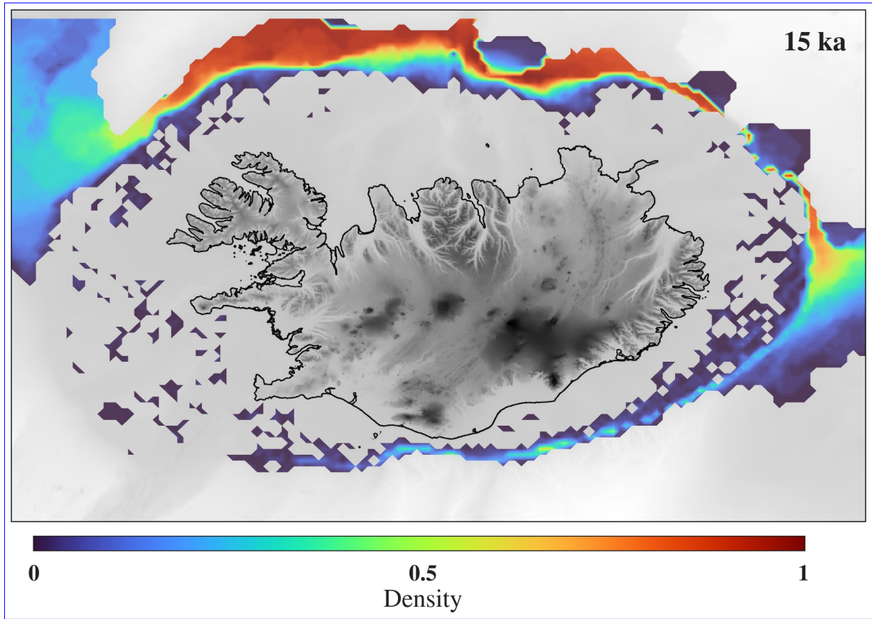
Figure A9. Density distribution of floating ice within the NROY tier1 sub-ensemble at 15 ka. To avoid ice extending to the grid boundary, the GSM is configured to strongly calve ice where present-day depth is greater than 860 m, as indicated by the black dotted line.
