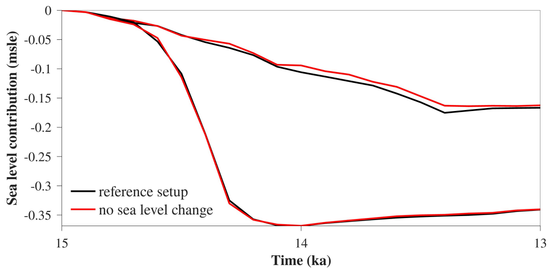
Figure A15. Sea level contribution relative to 15 ka from experiments with sea level change (black) and without sea level change (red) for 2 NROY tier1 parameter vectors (run identification number nn1131, and nn1395, the latter showing the strongest sensitivity in the ensemble).
