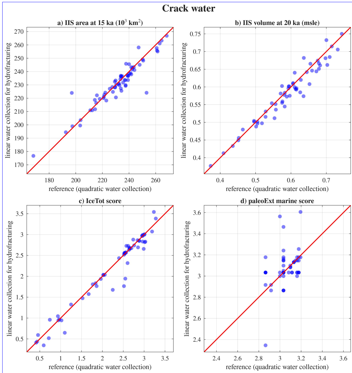
Figure A17. Sensitivity of the IIS to crack water collection parameterizations for hydrofracturing. Scatter plots compare the reference quadratic water collection (x-axis) against a linear water collection (y-axis). (a) IIS grounded ice area at 15 ka ( 10^3 \text{ km}^2 ). (b) IIS ice volume at 20 ka (msle). (c) Total ice thickness misfit score (IceTot). (d) Marine paleo-extent misfit score (paleoExt). The red solid line indicates the 1:1 relationship.
