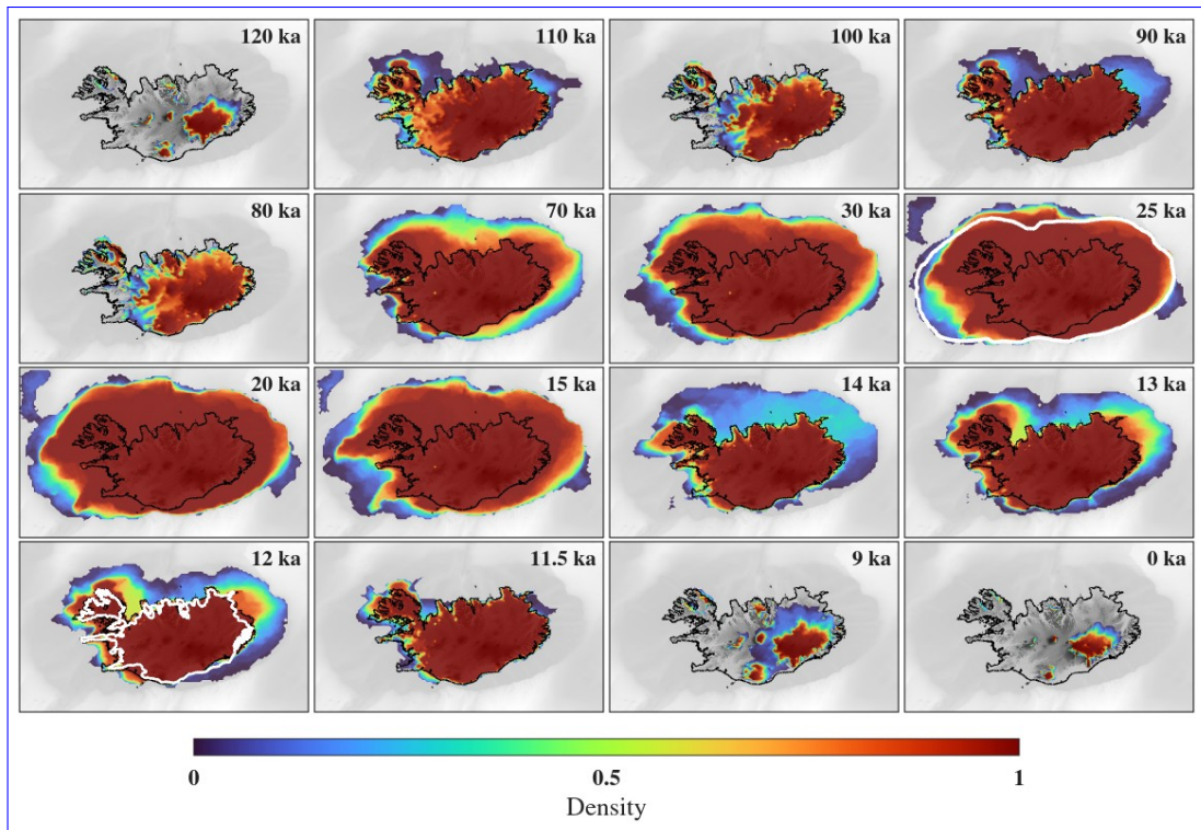
Figure 6. (a) Time series of IIS volume during the last glacial cycle. Initial full ensemble (gray shaded area) and sieved non-ruled out yet (NROY tier1 ) sub-ensemble (blue distribution) with median NROY tier1 (black curve). (b) Density distribution of grounded ice within the NROY tier1 sub-ensemble at different time slices. White contours on the 25, and 12 ka panels show empirical ice-margin reconstructions for 25.5 \pm 2.5 ka (Benediktsson et al., 2022b, 2023a), and 12.5 \pm 3.0 (Benediktsson et al., 2023b), respectively.
