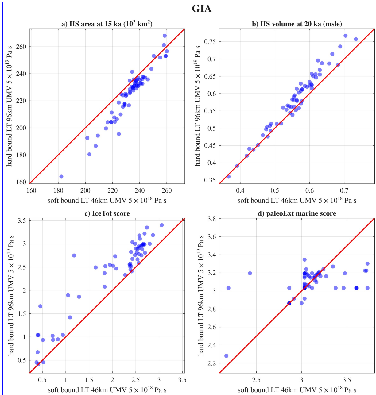
Figure A16. Sensitivity of the IIS to Glacial Isostatic Adjustment (GIA) Earth model parameters. Scatter plots compare a soft bound Earth model (lithosphere thickness 46 km, upper mantle viscosity 5 \times 10^{18} \text{ Pa s} ; x-axis) against a hard bound Earth model (lithosphere thickness 96 km, upper mantle viscosity 5 \times 10^{19} \text{ Pa s} ; y-axis). (a) IIS grounded ice area at 15 ka ( 10^3 \text{ km}^2 ). (b) IIS ice volume at 20 ka (msle). (c) Total ice thickness misfit score (IceTot). (d) Marine paleo-extent misfit score (paleoExt). The red solid line indicates the 1:1 relationship.
