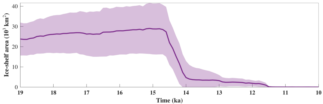
Figure A10. Time series of the ice shelf area during the last deglaciation for the NROY tier1 subset. The line represents the means and the shaded area the 2\sigma range.
