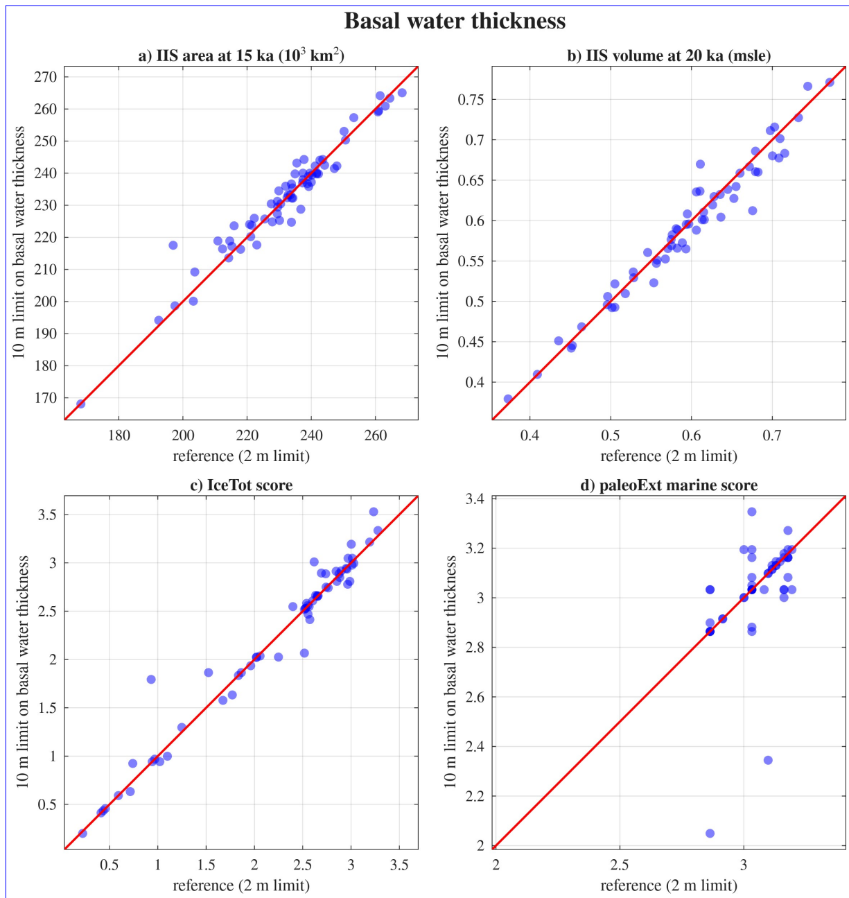
Figure A18. Sensitivity of the IIS to the basal water thickness limit. Scatter plots compare the reference 2 m limit (x-axis) against a 10 m limit on basal water thickness (y-axis). (a) IIS grounded ice area at 15 ka ( 10^3 \text{ km}^2 ). (b) IIS ice volume at 20 ka (msle). (c) Total ice thickness misfit score (IceTot). (d) Marine paleo-extent misfit score (paleoExt). The red solid line indicates the 1:1 relationship.
