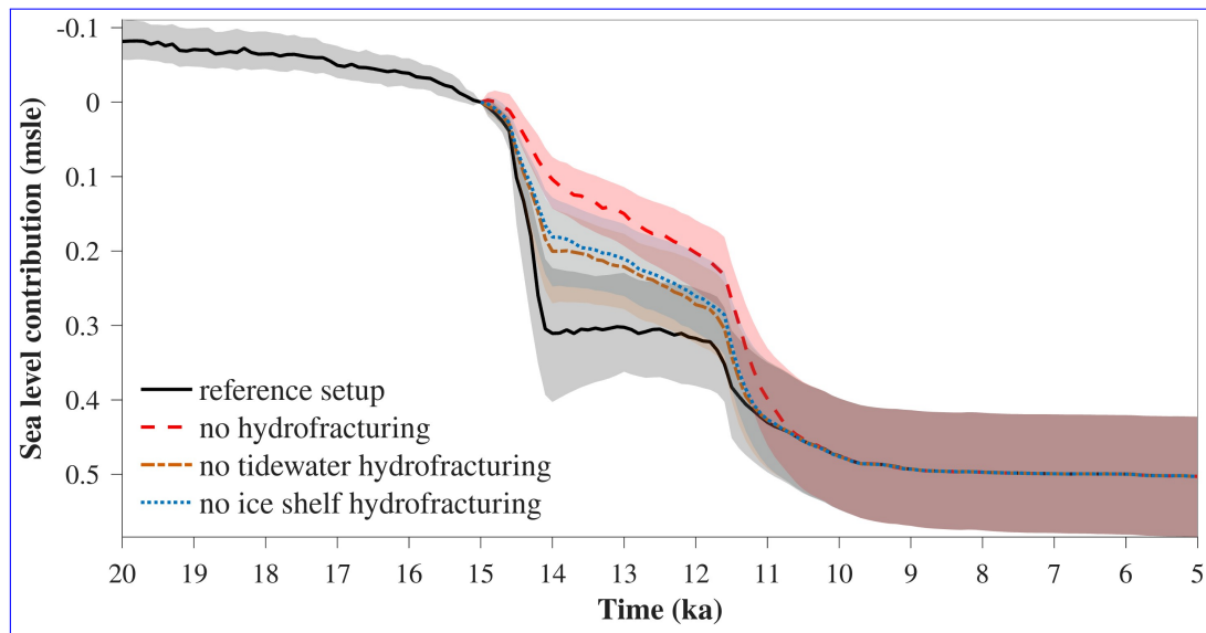
Figure 11. Sea level contribution relative to 15 ka from experiments with hydrofracturing (black) and, without hydrofracturing (red), without hydrofracturing only for tidewater margins (orange), and without hydrofracturing only for ice shelf (blue) based on the 107 NROY tier1 parameter vectors. The lines represent the medians and the shaded areas show the 2\sigma ranges.
