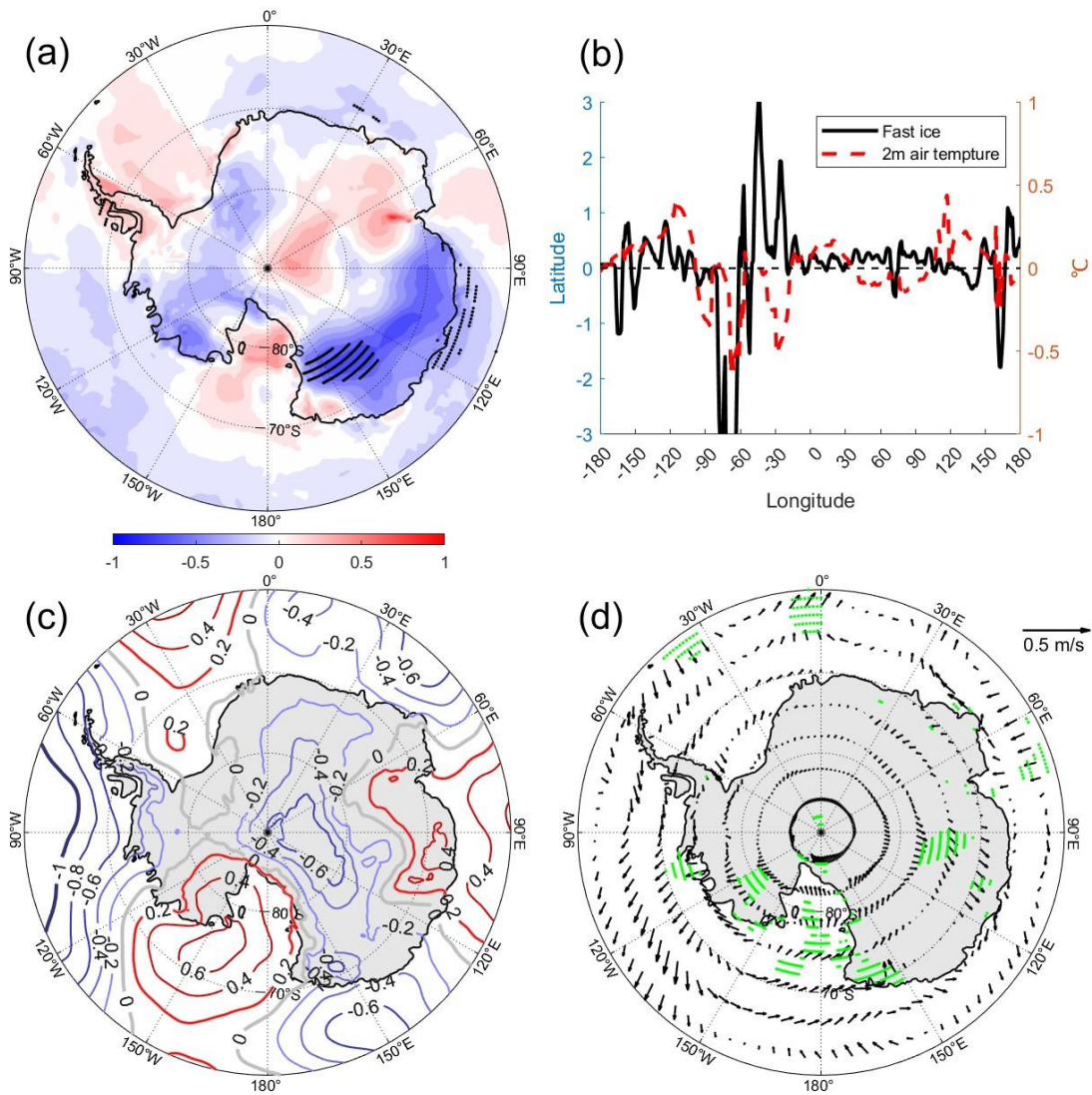
Figure 9. The same as Figure 6, but for summer.
