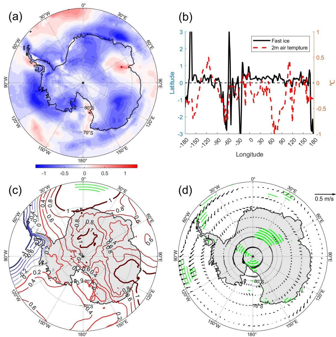
Figure 8. The same as Figure 7, but for winter.
