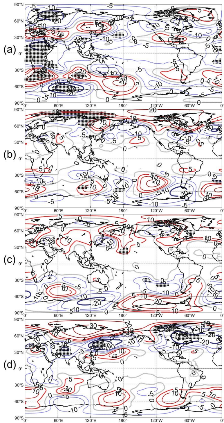
Figure 6: Regression of 200 hPa geopotential height (in gpm) onto the PC1: (a) autumn, (b) winter, (c) spring, and (d) summer. Regions with black dots indicate areas above 95% confidence level.
