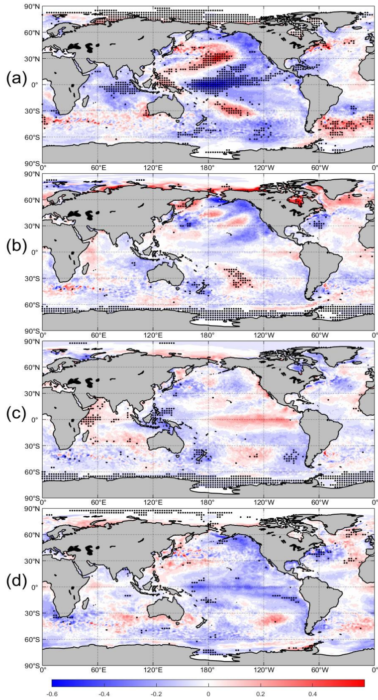
Figure 4: Regression of SST (in ^{\circ}\text{C} ) onto the PC1: (a) autumn, (b) winter, (c) spring, and (d) summer. Regions with black dots indicate areas passing the 95% confidence level.
