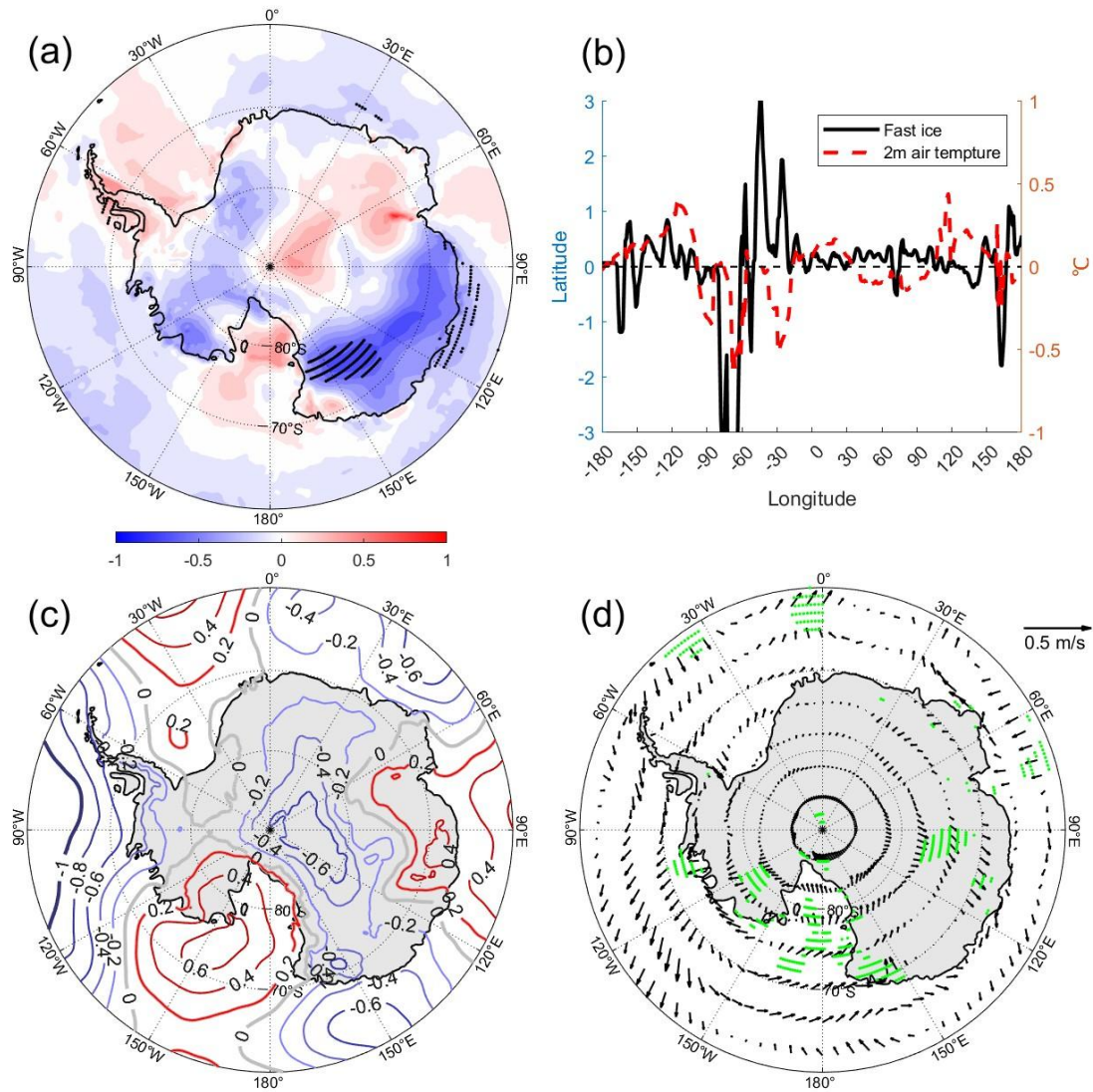
Figure 10. The same as Figure 7, but for summer.
