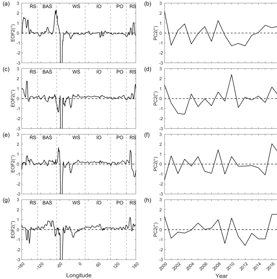
Figure 3: The same as figure 2 but for the second EOF mode.
