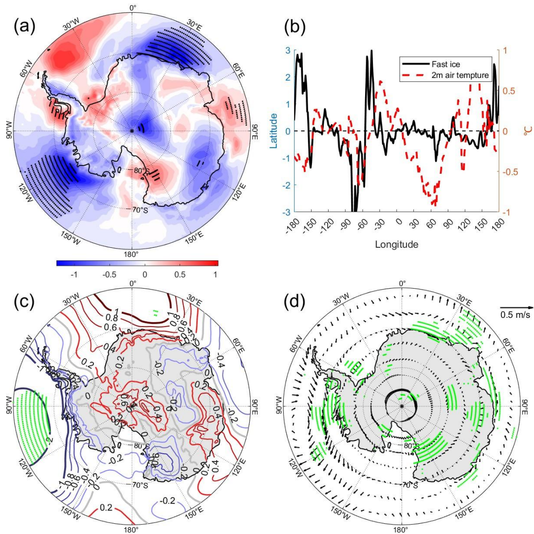
Figure 7: Regression of atmospheric variables onto the PC1 during autumn: (a) 2m air temperature (in ^{\circ}\text{C} ), (b) 2m air temperature (dashed) in fast ice region and fast ice coverage (solid), (c) MSLP (in hPa), (d) 10m wind field. Green and black dots indicate above 95% confidence level.
