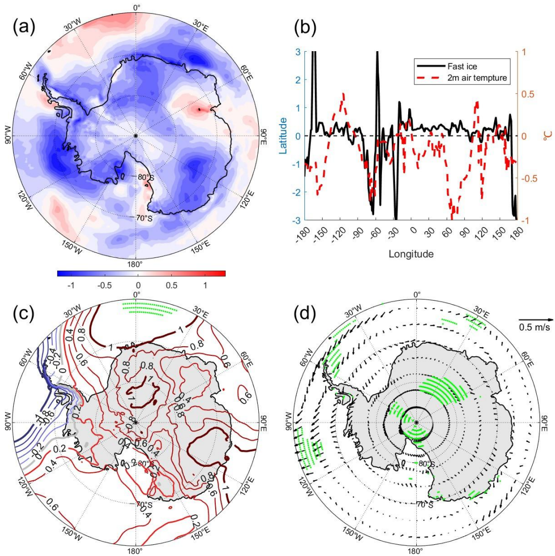
295 Figure 8. The same as Figure 7, but for winter.
