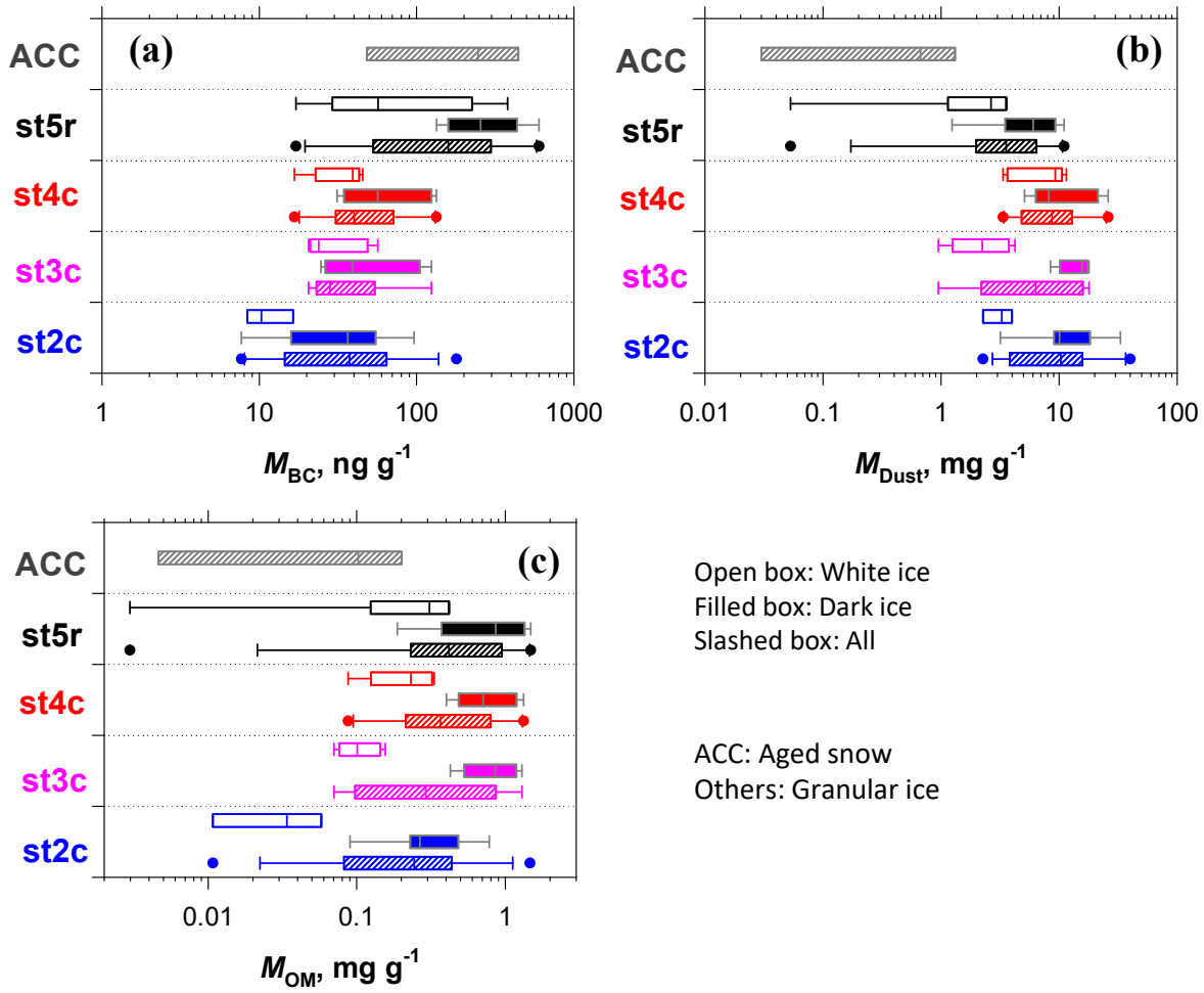
Figure 4: Box plots of the mass concentration of BC, mineral dust, and organic matter in water ( M_{BC} , M_{Dust} , and M_{OM} ) for surface ice samples collected during 22 July – 2 August in 2024. The left boundary of the box shows the 25th percentile. The line within the box represents the median. The right boundary of the box stands for the 75th percentile. The whiskers left and right of the box respectively show the 90th and 10th percentiles.
