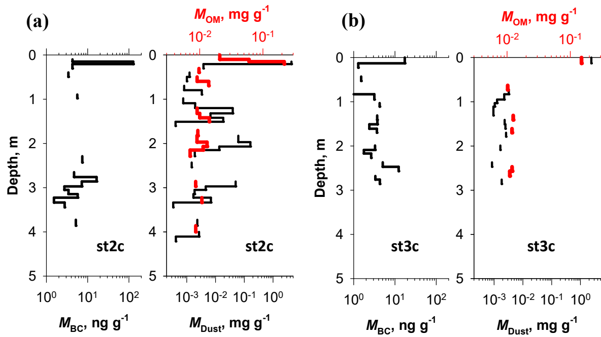
Figure 8: Vertical profile of BC, organic matter, and mineral dust for ice core samples drilled at st2c on 31 August 2022 (a) and at st3c on 1 September 2022. Cases for which no data were obtained because of storage vial cracking are blanked.
