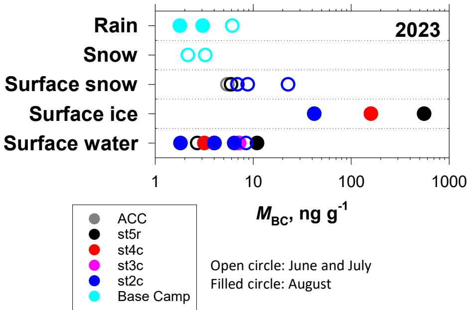
Figure 3: Mass concentrations of BC in water ( M_{BC} ) for surface snow, surface ice, surface water, snow, and rain samples collected during 30 June – 12 August in 2023.
