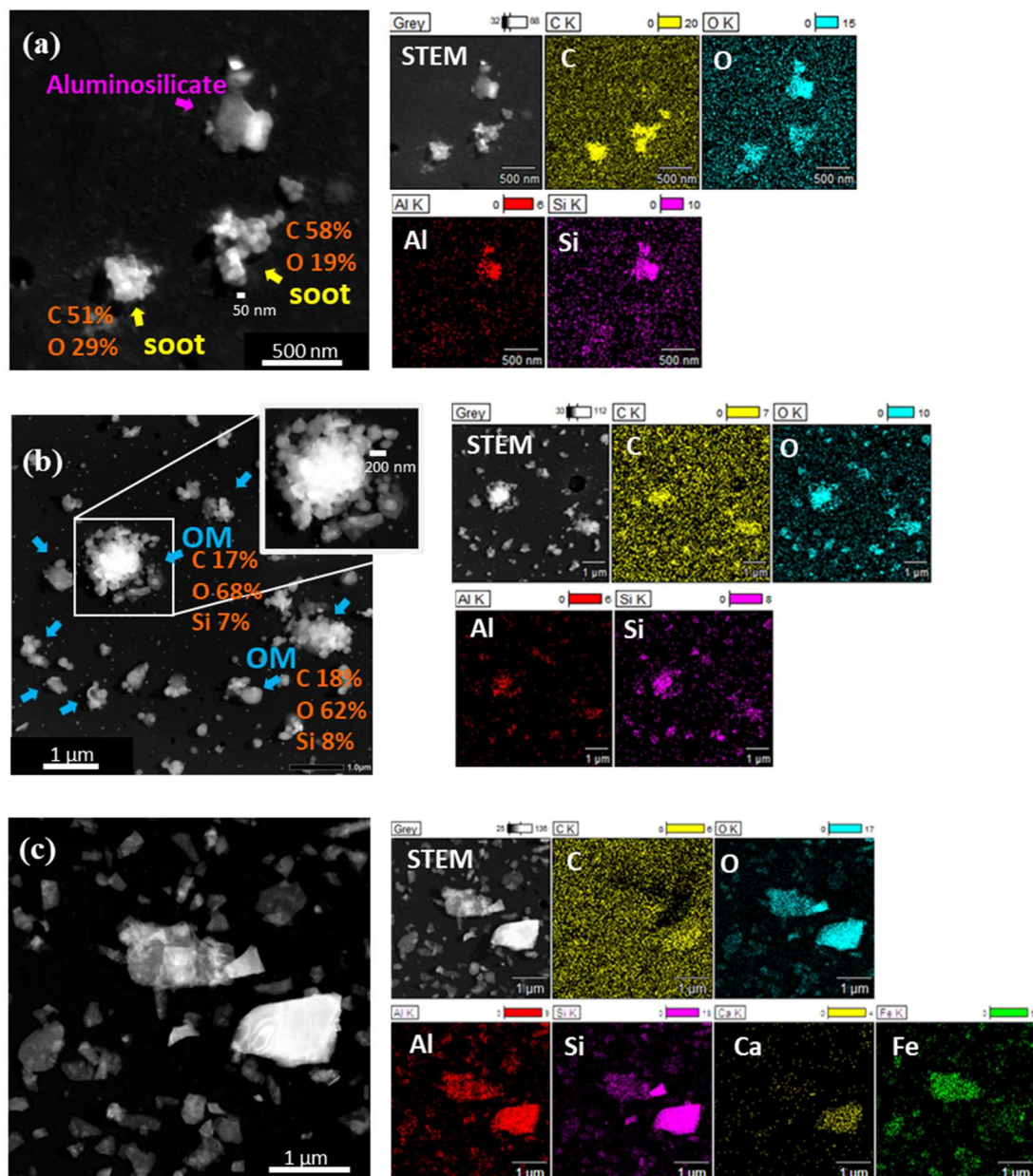
Figure 6: STEM images and elemental maps of water-insoluble particles collected at the smallest particle stage: (a) soot and aluminosilicate in a snow sample at base camp (23BC#04); (b) fine OM particles in surface ice samples at st5r (23BC#25), and fine aluminosilicate particles in surface ice sample at st2c (23BC#30).
