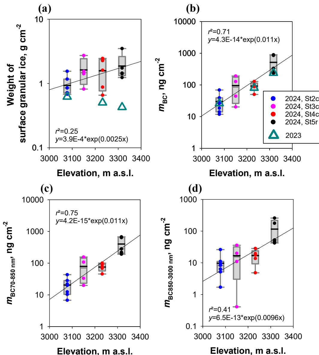
Figure 10: Relation of elevations with weight of surface granular ice per unit area (a) and total BC (b) in 2023 and 2024, and size-segregated BC mass (c and d) in surface granular ice for st5r, 4c, 3c, and 2c in 2024. Dark ice samples, which covered most of the surface, were used, whereas white ice was excluded because of its minor area.
