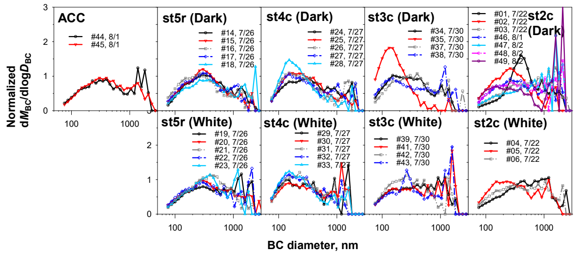
Figure 5: Normalized mass-size distributions of BC in the samples: 2023 and 2024.
