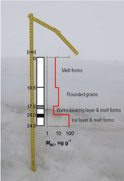
Figure 7: Vertical profile of BC and snow types for snow pit at the ACC site, 2023.
