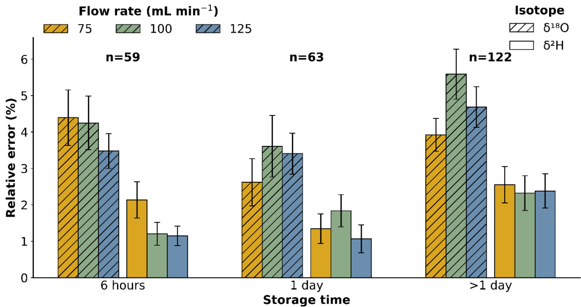
Figure 8. Relative error (%) for δ 18 O (hatched bars) and δ 2 H (solid bars) as a function of storage time (6 hours, 1 day, and >1 day) and sampling flow rates (75, 100, and 125 mL min -1 ). The number of observations (n) for each storage category is shown above the bars. Error bars represent the standard deviation.
