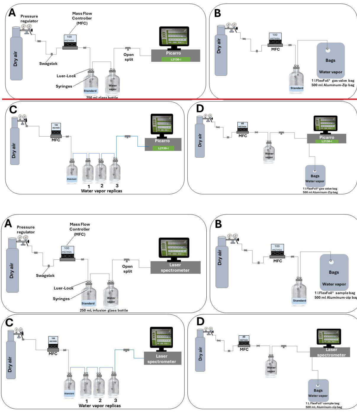
Figure 2. Technical implementation of the experiments. The schemes show the technical components used throughout the experiments sal stages: (A) setup for continuous generation of reference water vapor from a liquid isotopic standard and direct analysis via laser spectroscopy (Picarro L2130-i); (B) configuration for filling 1 L FlexFoil gas-valve sample bags and 500 mL Aluminum-zip storage bags with reference vapor; (C) system for simultaneous filling of three 250 mL infusion glass bottle replicates to ensure consistent water vapor isotopic composition for flow rate experiments; and (D) measurement configurations for stored samples, including a dry air push system with a T-junction open split for 250 mL infusion glass bottles and bags (left), and a direct inlet connection for gas bag analysis (right). In all configurations, gas flow rates were precisely controlled using a pressure regulator and an electronic mass flow controller (MFC).
