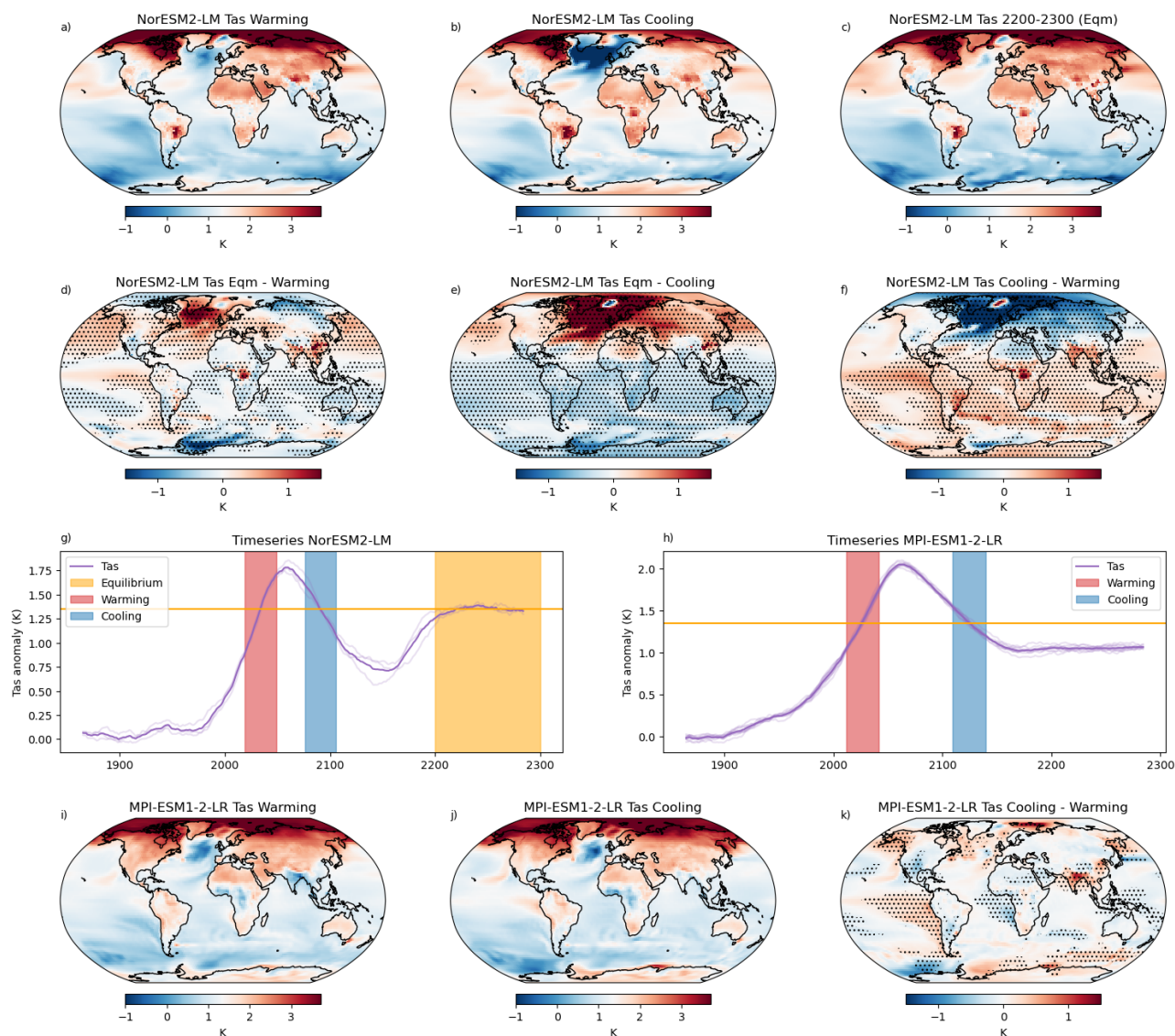
Figure 8. Global and regional near-surface air temperature projections in (a-g) NorESM2-LM and (h-k) MPI-ESM1.2-LR in the esm-ssp534-over scenario. (a-c): regional changes in NorESM2-LM for (a) warming; (b) cooling; (c) long-term stabilisation around a 1.35°C GWL. (d-f): Differences between (d) equilibrium and warming; (e) equilibrium and cooling; (f) cooling and warming in NorESM2-LM; (g-h) 31-year-smoothed timeseries of GSAT for (g) NorESM2-LM, showing times of warming (red), cooling (blue) and stabilisation (yellow) at the 1.35°C GWL and (h) MPI-ESM1.2-LR showing warming (red) and cooling (blue). (i-k) regional temperature at 1.35°C GWL in MPI-ESM1.2-LR for (i) warming; (j) cooling and (k) cooling minus warming. In (d-f) and (k), stippling shows areas where the differences are more than twice the standard deviation of the ensemble mean. In (g) and (h), red and blue shaded regions show the 31-year period around the ensemble mean 1.35°C GWL, and individual ensemble members may use data from slightly earlier or later periods.
