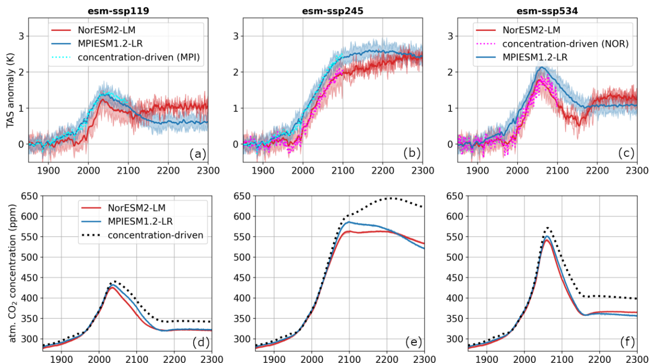
Figure 3. The evolution of the global mean temperature anomaly (a-c) and the atmospheric CO 2 concentration (d-f) in NorESM2-LM and MPI-ESM1.2-LR for esm-ssp119 (a,d), esm-ssp245 (b,e) and esm-ssp534-over (c,f). Shown are the ensemble mean, as well as the full range spanned by the ensemble members for the emissions-driven simulations. Where available, the parallel data from the concentration-driven simulations is given with dotted lines (temperature for ssp119 in MPI-ESM1.2-LR and for ssp534-over in NorESM2-LM, and CO 2 concentration time series from Meinshausen et al. (2020) for all three scenarios).
