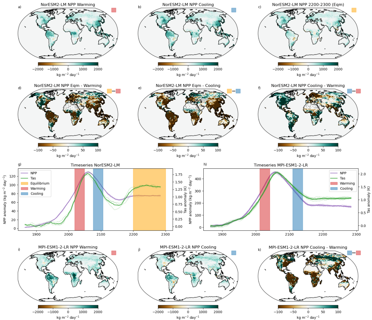
Figure 10. As figure 9, for net primary productivity. In (a-c) and (i,j), anomalies are shown relative to pre-industrial. In (g) and (h), global means of both mean GSAT anomaly (green) and precipitation-total net primary productivity (purple) are shown.
