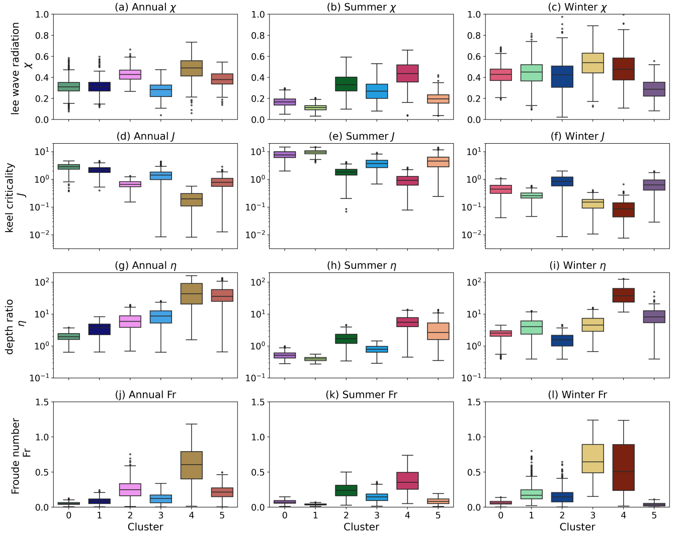
Figure 6. Distribution of nondimensional variables across six GMM clusters for different averaging periods: (a, d, g, j) annual, (b, e, h, k) summer months (JJA), and (c, f, i, l) winter months (DJF). For each averaging period, the spatial distributions of the clusters are shown in Fig. 4. Each subplot corresponds to a single parameter: (a-c) \chi , (d-f) J , (g-i) \eta , and (j-l) Fr . Individual boxes show the interquartile range, median, and outliers for each cluster. Note that keel criticality parameter J (d-f) and depth ratio \eta (g-i) are plotted on a log scale to easily compare across clusters and seasons.
