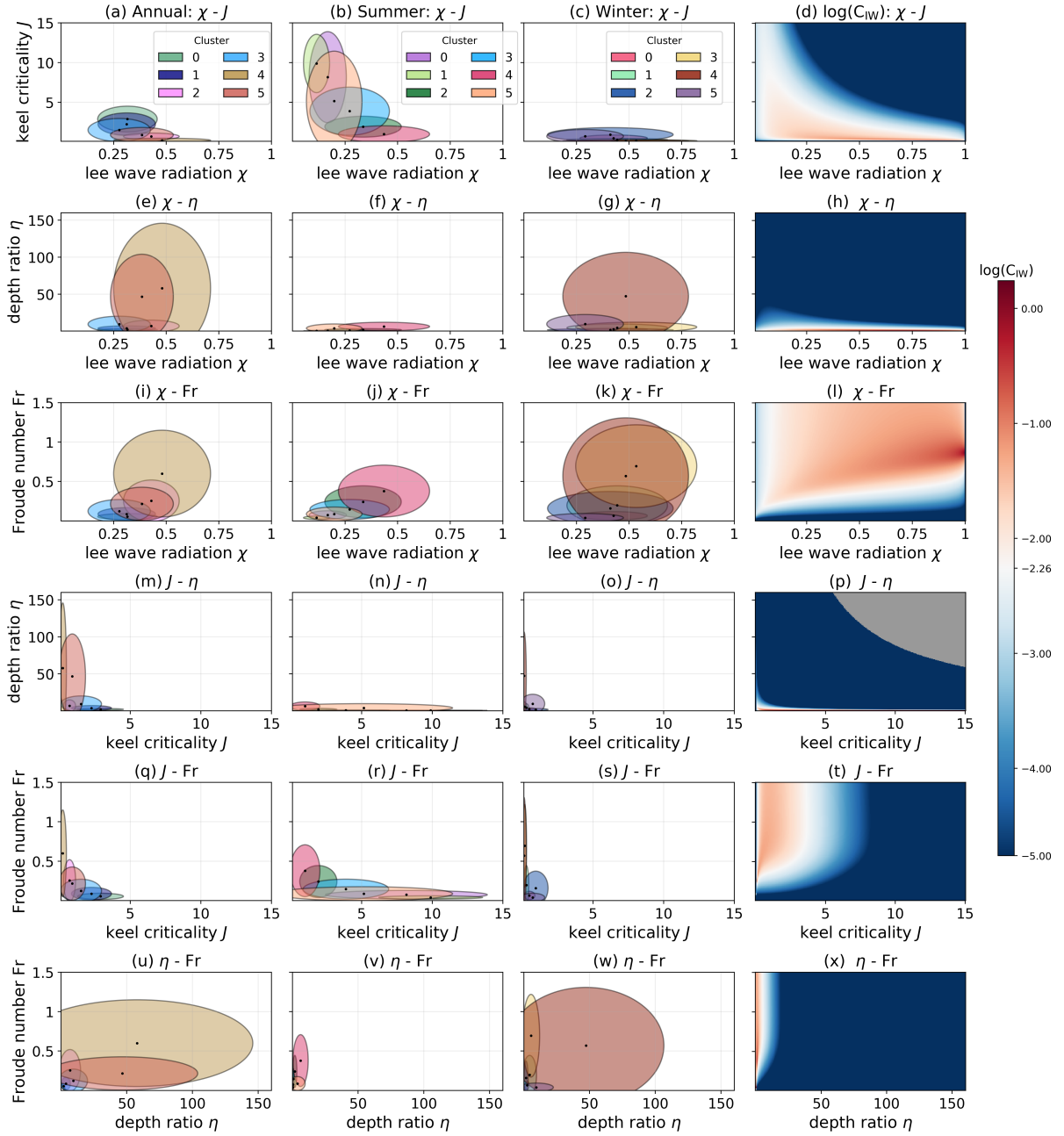
Figure 9. (left three columns) Pairwise ellipse plots showing the cluster-mean values and associated variability across six GMM-identified regimes (columns from left to right: Annual, Summer (JJA), Winter (DJF)). Each colored ellipse is centered at the cluster mean for the variable pair shown and spans two standard deviations along each axis, capturing the internal spread of that cluster. (right column) internal wave drag C_{IW} induced by the ice keel calculated from the parameterization expression over the joint pairwise parameter range. The values of C_{IW} are plotted on a logarithmic scale and the white values (center of the colorbar) corresponds to the canonical ice-ocean drag coefficient value of C_D = 5.5 \times 10^{-3} ( \log(C_D) = -2.26 ). Subplots on each row correspond to the following pairs: (a-d) \chi - J , (b-h) \chi - \eta , (i-l) \chi -Fr, (m-p) J - \eta , (q-t) J -Fr, and (u-x) \eta -Fr. Note that the grey shaded region in (p) represents undefined values in the parameterization due to the large values of J and \eta .
