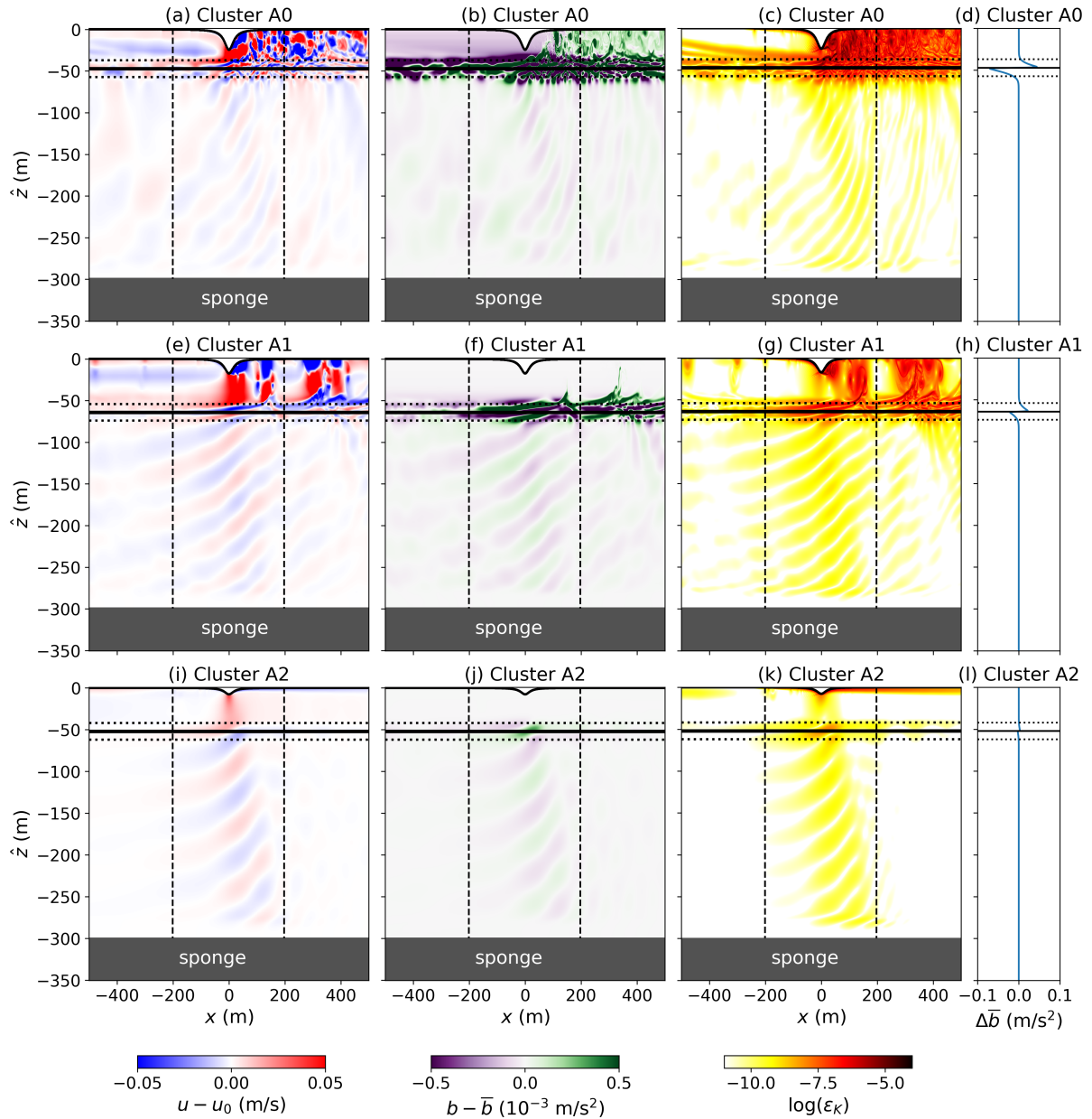
Figure 7. Snapshots from numerical simulations set with nondimensional parameters for GMM clusters A0 (a-d), A1 (e-h), and A2 (i-l): (a, e) turbulent horizontal velocity u - u_0 , (b, f) buoyancy perturbations, i.e., deviations from horizontally-averaged \bar{b}(z) , (c, g) log of kinetic energy dissipation \epsilon_K , and (d, h) buoyancy deviation from initial conditions \Delta\bar{b} = \bar{b}(z) - b_0(z) . The thick black horizontal black lines in each subplot indicate the pycnocline \hat{z} = z_0 and horizontal dotted lines delineate \hat{z} = z_0 \pm 10 m. In (a-c, e-g), dashed vertical lines delineate the region x \in [-200, 200] m, which is used for horizontal averages and integrals. All snapshots are for the last timestep (after 6 hours) of simulation time.
