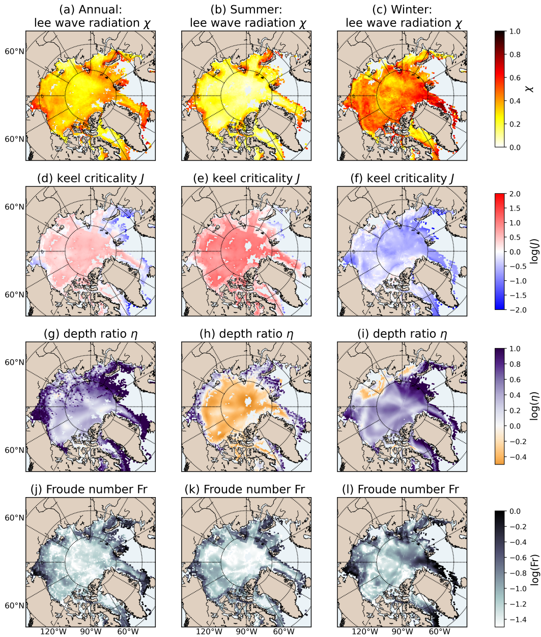
Figure 2. Spatial distribution of time-averaged four nondimensional parameter over the Arctic Ocean: (a-c) \chi defined in Eqn. (1), (d-f) J defined in Eqn. (2), (g-i) \eta defined in Eqn. (8), and (j-l) Fr defined in Eqn. (9). Parameters are averaged over different time periods: (a, d, g, j) annually, (b, e, h, k) summer months (JJA), and (c, f, i, l) winter months (DJF). The post-processing of the variables is described in § 3. Note that colorbars vary across subplots and the magnitudes of J , \eta and Fr are shown on a logarithmic scale. Figure is made with Matplotlib Basemap toolkit library ( https://matplotlib.org/basemap/stable/ )
