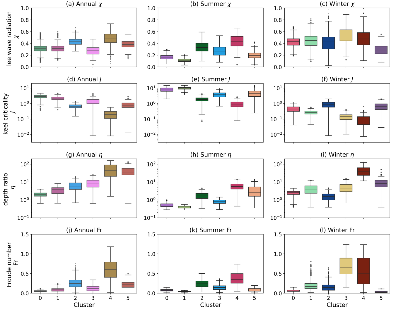
Figure 6. Distribution of nondimensional variables across six GMM clusters for different averaging periods: (a, d, g, j) annual, (b, e, h, k) summer months, and (c, f, i, l) winter months. For each averaging period, the spatial distributions of the clusters are shown in Fig. 4. Each subplot corresponds to a single parameter: (a-c) \chi , (d-f) J , (g-i) \eta , and (j-l) Fr . Individual boxes show the interquartile range, median, and outliers for each cluster. Note that keel criticality parameter J (d-f) and depth ratio \eta (g-i) are plotted on a log scale to easily compare across clusters and seasons.
