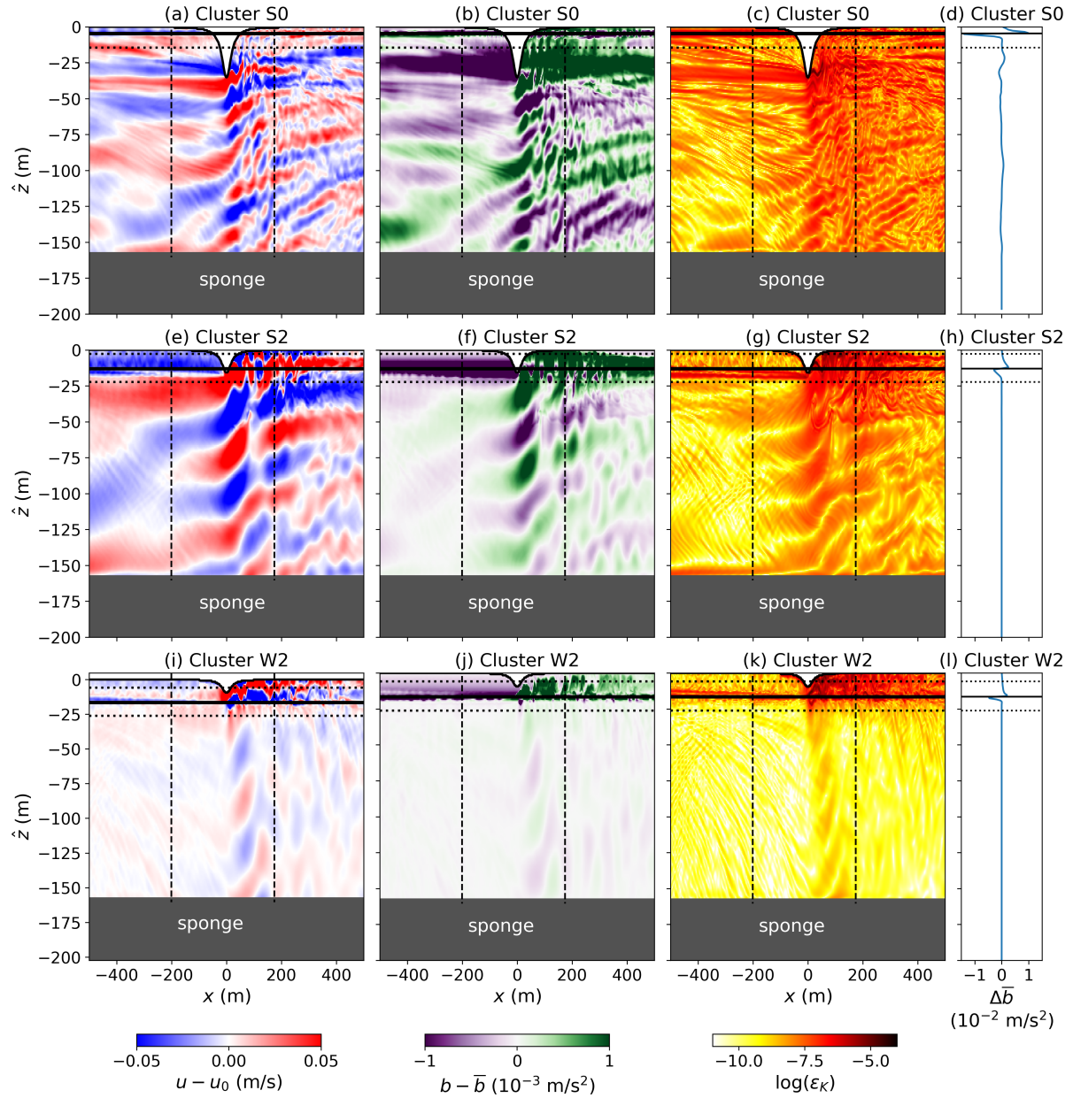
Figure 11. Snapshots from numerical simulations set with nondimensional parameters for GMM clusters S0 (a-d), S2 (e-h), and W2 (i-l): (a, e) turbulent horizontal velocity u - u_0 , (b, f) buoyancy perturbations, i.e., deviations from horizontally-averaged \bar{b}(z) , (c, g) log of kinetic energy dissipation \epsilon_K , and (d, h) buoyancy deviation from initial conditions \Delta\bar{b} = \bar{b}(z) - b_0(z) . The thick black horizontal black lines in each subplot indicate the pycnocline \hat{z} = z_0 and horizontal dotted lines delineate \hat{z} = z_0 \pm 10 m. In (a-c, e-g), dashed vertical lines delineate the region x \in [-200, 200] m, which is used for horizontal averages and integrals. All snapshots are for the last timestep (after 6 hours) of simulation time.
