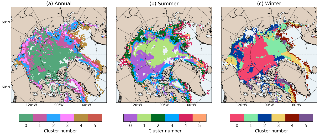
Figure 4. The spatial distribution of six statistically inferred regimes ( K=6 ), each represented by a unique color, over the Arctic Ocean domain, derived from a GMM fitted to standardized time-averaged nondimensional parameter values across all spatial grid points. The values are based on the values averaged over different time intervals: (a) annually, (b) over the summer months, and (c) over the winter months. Clusters within each temporal averaging space are all ordered in the descending proportion of data points that belong to each cluster (i.e., most data points belong to cluster 0). Figure is made with Matplotlib Basemap toolkit library ( https://matplotlib.org/basemap/stable/ ).
