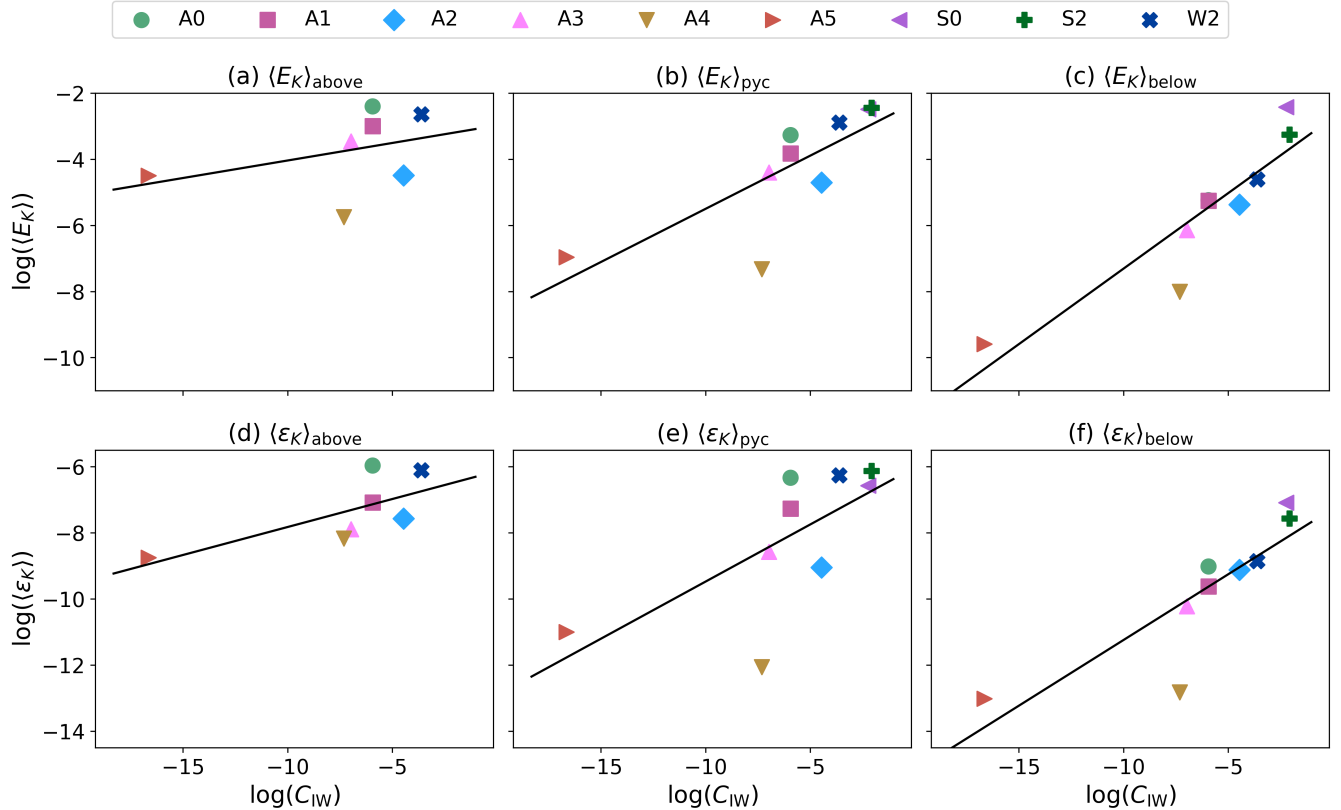
Figure 12. KE metrics (a-c) KE E_K and (d-f) KE dissipation \epsilon_K calculated from numerical simulations plotted against IW drag C_{IW} estimated from the McPhee and Kantha (1989) parameterization. KE metrics are area-averaged over different regions of the simulation domain: (a, d) above the pycnocline above, (b, e) within the pycnocline pyc, and (c, f) below the pycnocline below) as defined in Eqns. (20)-(22). Each scatter symbol corresponds to a different simulation as denoted in the legend (annual clusters A0 – 5, summer clusters S0 and S2, and winter cluster W2). Nondimensional parameters for these simulations are shown in Table 1 and raw values of \langle E_K \rangle and \langle \epsilon_K \rangle can be found in Table 2.
