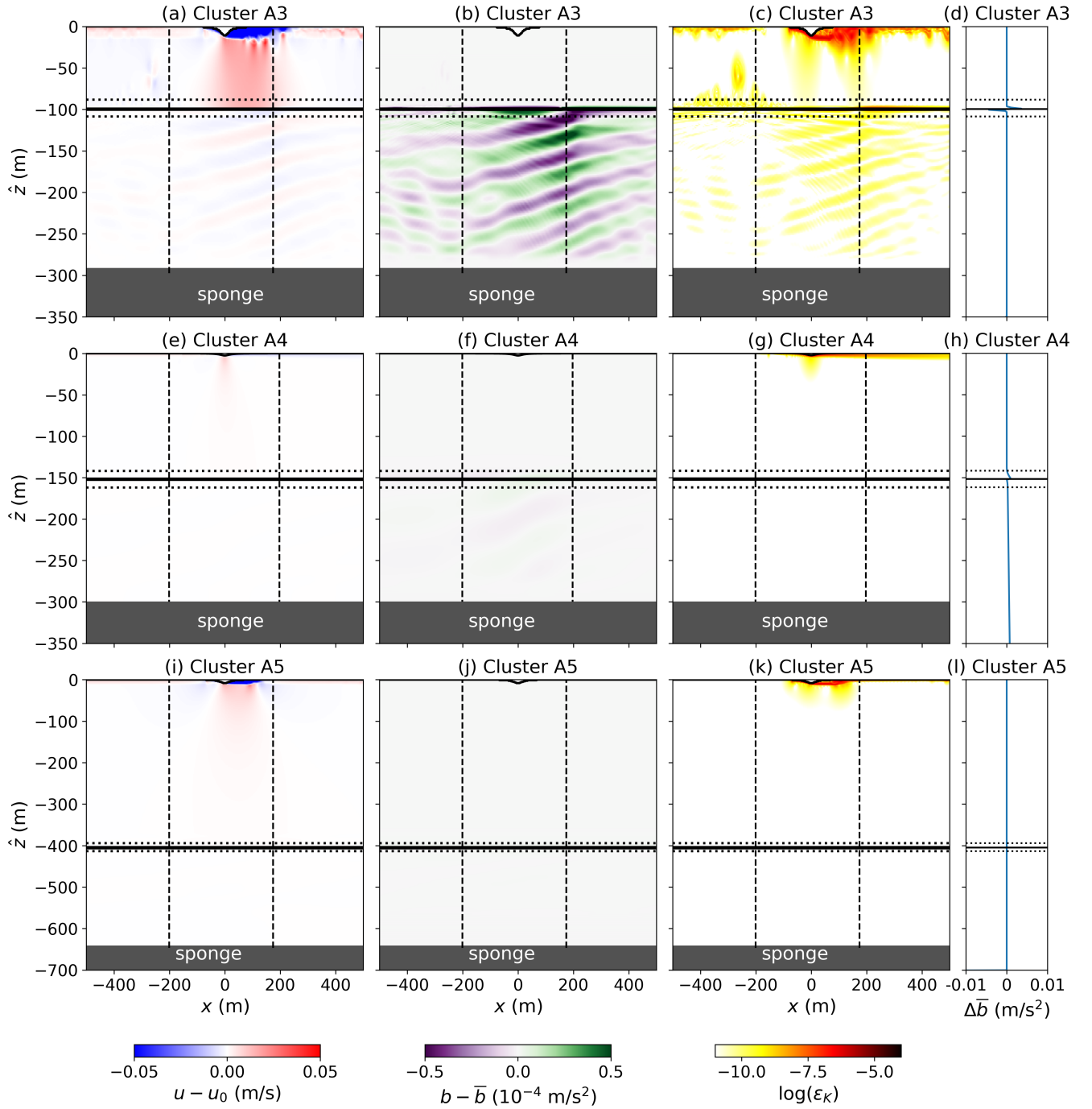
Figure 8. Same as Figure 7 but for (a-d) Cluster 3, (e-h) Cluster 4, and (i-d) Cluster 5. Note that the colorbar in (b, f, j) for the buoyancy plots are different from those in Figure 7.
