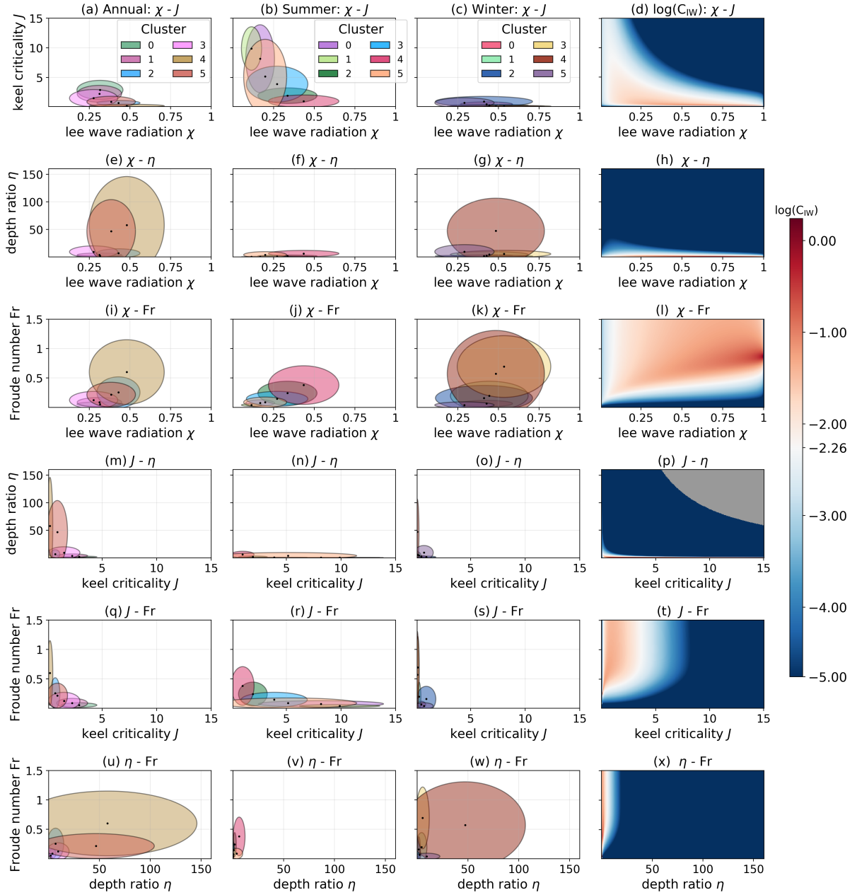
Figure 9. (left three columns) Pairwise ellipse plots showing the cluster-mean values and associated variability across six GMM-identified regimes (columns from left to right: Annual, Summer, Winter). Each colored ellipse is centered at the cluster mean for the variable pair shown and spans two standard deviations along each axis, capturing the internal spread of that cluster. (right column) internal wave drag C_{IW} induced by the ice keel calculated from the parameterization expression over the joint pairwise parameter range. The values of C_{IW} are plotted on a logarithmic scale and the white values (center of the colorbar) corresponds to the canonical ice-ocean drag coefficient value of C_D = 5.5 \times 10^{-3} ( \log(C_D) = -2.26 ). Subplots on each row correspond to the following pairs: (a-d) \chi - J , (b-h) \chi - \eta , (i-l) \chi - Fr , (m-p) J - \eta , (q-t) J - Fr , and (u-x) \eta - Fr . Note that the grey shaded region in (p) represents undefined values in the parameterization due to the large values of J and \eta .
