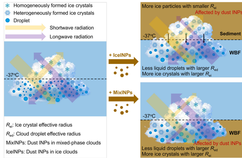
Figure 10. Schematic of the effects of dust INPs in mixed-phase and ice clouds on clouds and radiation. Dust INPs in mixed-phase clouds enhance the Wegener–Bergeron–Findeisen (WBF) process, producing fewer but larger droplets and more, larger ice crystals, which reduce shortwave albedo, increase longwave transmittance, and lead to a net warming effect. In ice clouds, dust INPs intensify heterogeneous nucleation, generating more but smaller ice crystals; their sedimentation further enhances the WBF process in mixed-phase clouds. The much stronger changes in ice clouds amplify the warming effect, dominated by longwave radiation, resulting in an overall net warming.
