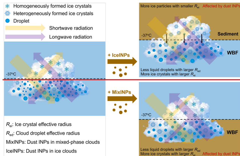
Figure 10. Schematic of the effects of dust INPs in mixed-phase and ice clouds on clouds and radiation. Dust INPs in mixed-phase clouds enhance the Wegener–Bergeron–Findeisen (WB) process, producing fewer but larger droplets and more, larger ice crystals, which reduce shortwave albedo, increase
