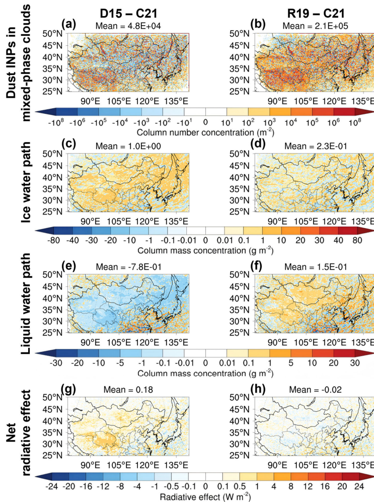
Figure 9. Simulated spatial distributions of (a–b) dust INP column number concentrations (vertically integrated) in mixed-phase clouds, (c–d) ice water path, (e–f) liquid water path, and (g–h) net radiative effect at the top of the atmosphere. The left column shows differences between the MixINPs_DeMott2015 scenario (DeMott2015, D15) and the MixINPs scenario (Chen2021, C21), and the right column shows differences between the MixINPs_Reicher2019 scenario (Reicher2019, R19) and the MixINPs scenario (Chen2021, C21). The mean value over the plotted region is shown above each panel. The simulated results are averages of hourly values from March to May 2018.
