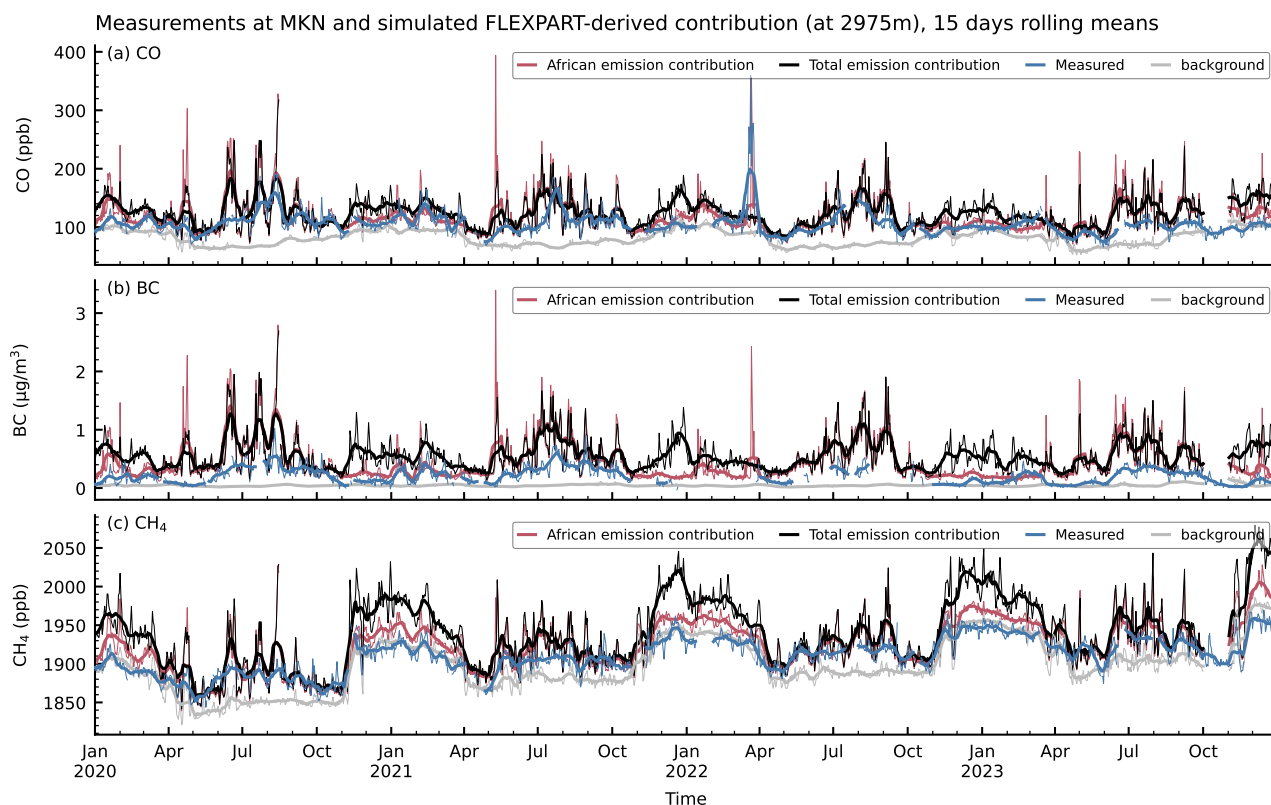
Figure 5. CO, BC and CH4 CH 4 measurements at Mt. Kenya and total simulated contributions accounting for fire, wetland, and anthropogenic emissions in the African domain (red) and the full domain (black). The background is derived from CAMS background data folded with FLEXPART footprints. Thin lines show daily averages, bold lines show data smoothed with a 15-days rolling mean.
