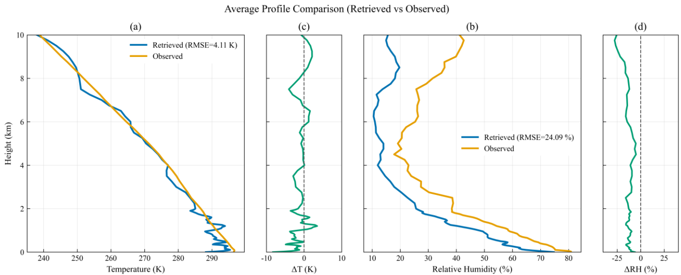
405 Figure 7: Statistical comparison of atmospheric profiles between the uncorrected NSGA-II retrievals and the collocated radiosonde observations for 38 matched cases collected during the Jiaozhou Bay field experiment. Panels (a) and (b) present the mean temperature and relative humidity profiles, respectively, after time matching and interpolation onto the common retrieval grid. Panels (c) and (d) show the corresponding profile differences, defined directly as the mean retrieved profiles minus the mean radiosonde profiles shown in panels(a) and (b).
