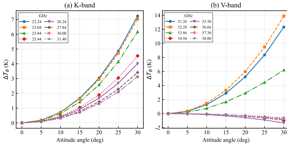
465 Figure 8: Sensitivity of brightness temperature ( \Delta T_B ) to viewing angle for selected K-band (a) and V-band (b) channels. A reference atmospheric profile was generated using the ITU-R P.835 standard atmosphere, and channel brightness temperatures were simulated under different viewing angles using gaseous absorption from the ITU-R P.676 model. Here, \Delta T_B denotes the difference between the brightness temperature at a given viewing angle and the nadir-view reference ( 0^\circ ). Each curve corresponds to a specific frequency channel, as indicated in the legends. The results show a nonlinear increase in \Delta T_B with viewing angle for several channels, 470 indicating that attitude-induced changes in observation geometry can introduce systematic brightness-temperature deviations and thereby affect retrieval accuracy.
