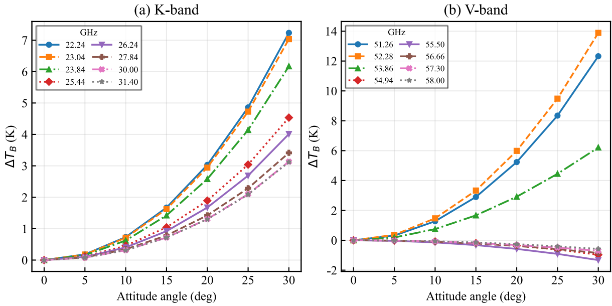
470 Figure 8: Sensitivity of brightness temperature ( \Delta T_B ) to viewing angle for selected K-band (a) and V-band (b) channels. A reference atmospheric profile was generated using the ITU-R P.835 standard atmosphere, and channel brightness temperatures were simulated under different viewing angles using gaseous absorption from the ITU-R P.676 model. Here, \Delta T_B denotes the difference between the brightness temperature at a given viewing angle and the nadir-view reference ( 0^\circ ). Each curve corresponds to a specific 475 frequency channel, as indicated in the legends. The results show a nonlinear increase in \Delta T_B with viewing angle for several channels, indicating that attitude-induced changes in observation geometry can introduce systematic brightness-temperature deviations and thereby affect retrieval accuracy.
