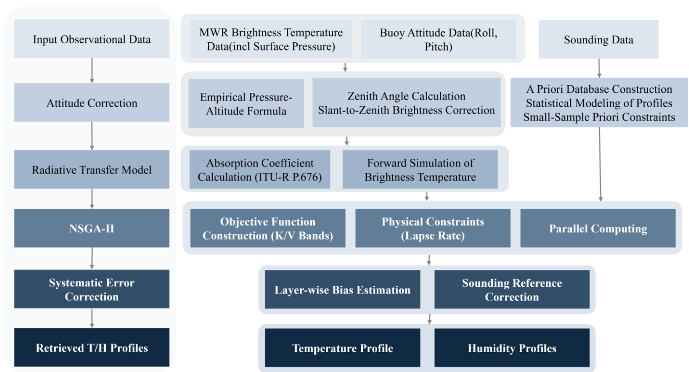
190 Figure 5: Schematic flowchart of the atmospheric temperature and humidity profile inversion method based on a microwave radiometer on a buoy platform. The workflow includes attitude correction of microwave radiometer observations, radiative transfer modeling and brightness temperature simulation, construction of multi-objective functions with physical constraints, NSGA-II optimization, and systematic error correction, resulting in the final retrieved temperature and humidity profiles.
