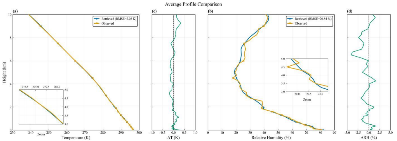
480 Figure 9: Comparison of retrieval results after applying the systematic error correction model. Panels (a) and (b) display the corrected temperature and relative humidity profiles, respectively. The blue solid lines represent the MWR retrieval results corrected by subtracting the systematic error profiles ET(h) and EH(h) as defined in Eqs. (6) and (7). The orange-yellow solid lines represent the reference radiosonde observations. Panels (c) and (d) display the residual error profiles after correction. Based on the 38 valid matchups, the Root Mean Square Error (RMSE) for the corrected profiles is reduced to 2.08 K for temperature and 20.95% for humidity across the 0–10 km vertical range. The corrected profiles shown in this figure are based on the independent testing subset and are not used in the construction of the bias correction model.
