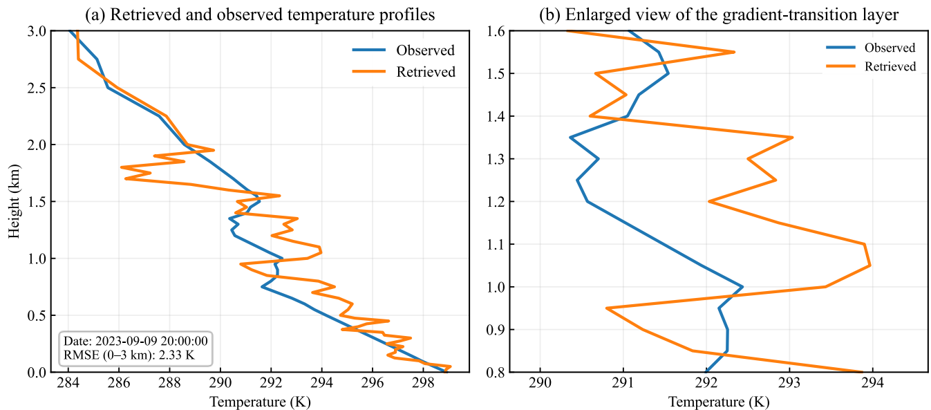
530 Figure 10: Representative case illustrating the effect of the imposed bounds and adjacent-layer continuity constraints on the retrieved temperature profile. The blue line denotes the collocated radiosonde profile, and the orange line denotes the retrieved profile. Panel (a) shows the full temperature profile from 0 to 3 km, while panel (b) presents an enlarged view of a lower-tropospheric
