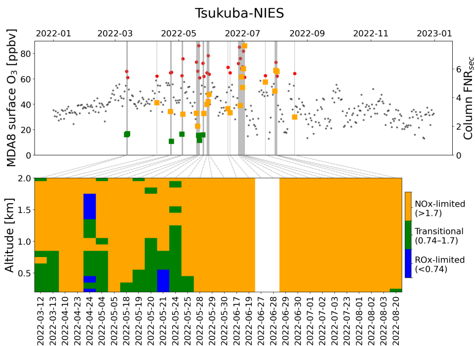
Figure 9: Sensitivity analysis of O 3 during MDA8 exceedance events at Tsukuba-NIES. The top panel presents MDA8 surface O 3 , with non-exceedance days indicated by black dots and exceedance events days shown as red points with grey shadows. Squares depict the column FNR sec derived from Pandora sky-scan measurements around local noon (12:00 ± 2:00). The bottom panel illustrates the vertical formation sensitivity of O 3 corresponding to exceedance events. The squares and color bars are colored according to FNR sec threshold values determined from the GEOS-Chem model.
