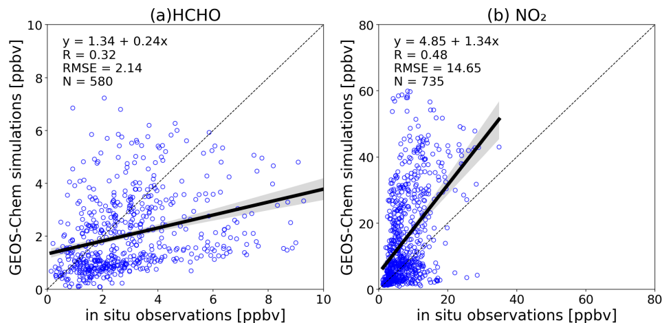
Figure 1: Scatter plots of the surface HCHO (a) and NO 2 (b) comparing in situ measurements with GEOS-Chem model simulation at Tokyo-TMU. The y-axis represents GEOS-Chem simulations, and the x-axis represents in situ observations. The dashed line indicates the 1:1 line.
