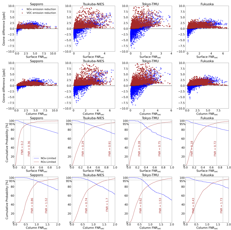
385 Figure 7: Response of surface O 3 to NO x and VOC emission perturbations resulting from the GEOS-Chem simulations. The scatter plots depict the O 3 difference between GEOS-Chem Run-2 and Run-3 (blue), and between Run-2 and Run-4 (brown), as a function of surface FNR sec (first row) and tropospheric column FNR sec (second row). The VOC-limited regime was associated with negative
