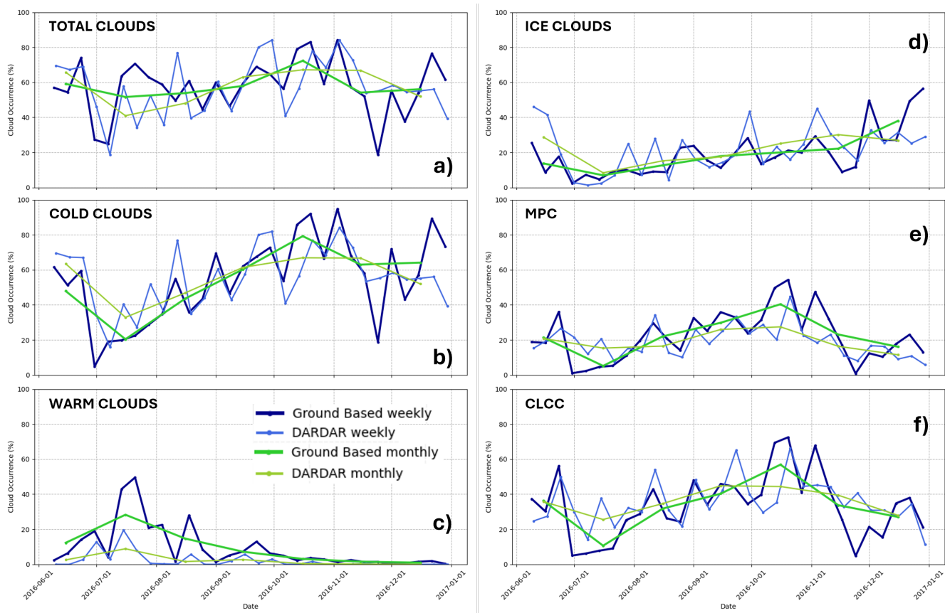
Figure 1. Comparison of DARDAR and ground-based observations of : (a) total, (b) cold, (c) warm, (d) ice, (e) mixed-phase, and (f) cold liquid-containing cloud occurrence up to 3000 m above ground level at Ny-Ålesund (78°55’N, 11°56’E). Weekly (blue) and monthly (green) occurrences are shown. Ground-based observations are represented by thicker, darker lines.
