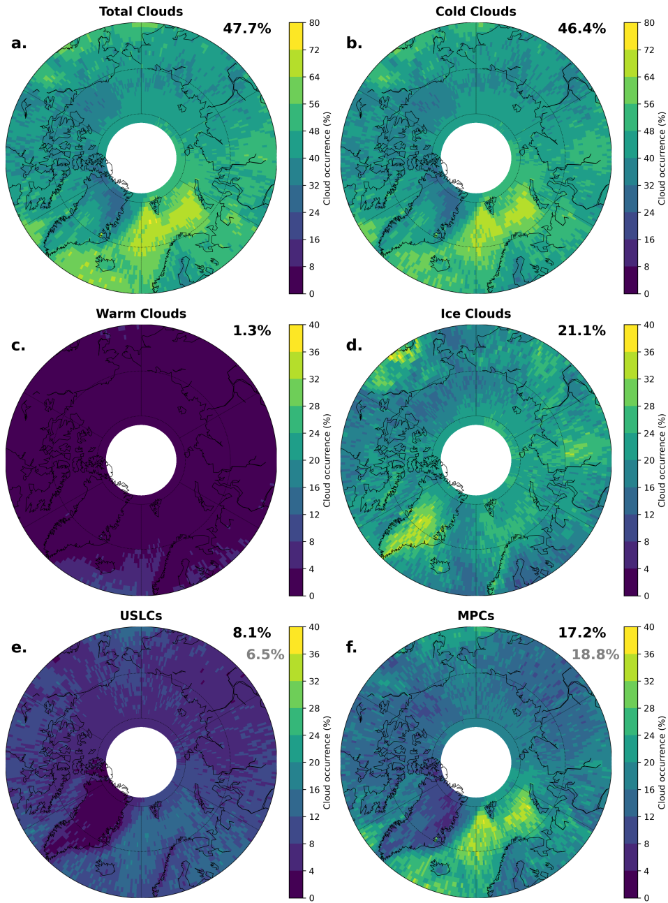
Figure 3. Stereographic projections of the occurrence of low-level (between the clutter height and 3 km AGL) cloud types between 2007 and 2016: (a) total clouds, (b) cold clouds, (c) warm clouds, (d) ice clouds, (e) USLCs, and (f) MPCs. The black numbers shown in the upper right of each subfigure are relative to the median occurrence over the entire study area. The gray numbers indicate the median occurrence of clouds whose phase classification may be affected by radar clutter.
