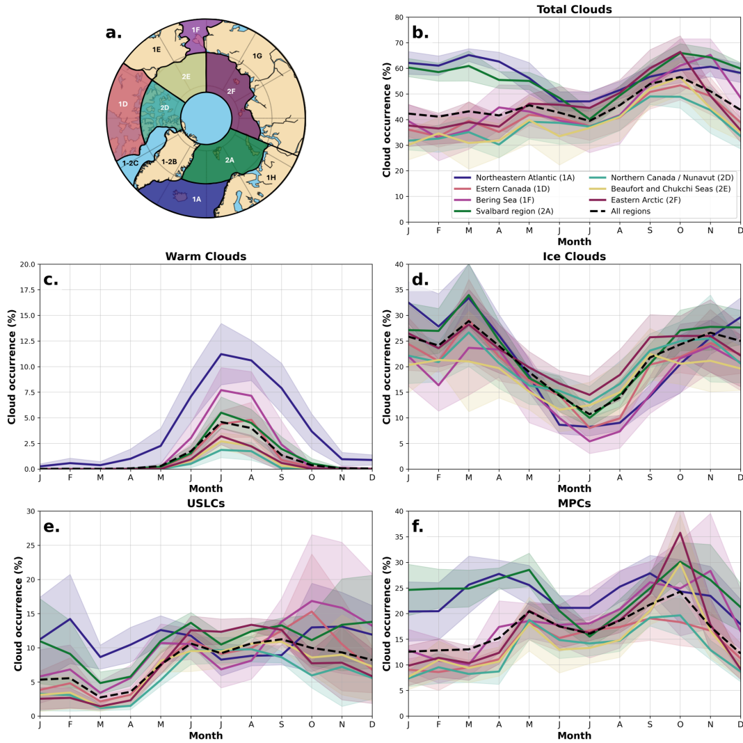
Figure 4. Monthly occurrence variations for different types of low-level clouds (between the clutter height and 3 km AGL) between 2007 and 2016: (b) total clouds, (c) warm clouds, (d) ice clouds, (e) USLCs, and (f) MPCs. Regionalization (a) with colored regions for monthly analysis. The colored areas around the curves represent the interquartile range. Zone 1 represents the low-latitude regions from 60°N to 70°N, excluding the Russian continental region. The letters for the different regions start from the North Atlantic zone (1A) and run from west to east. Zone 2 is the second high-latitude ring, from 70°N to 82°N. Regions in this latitude band are referred to in the same way as the first ring.
