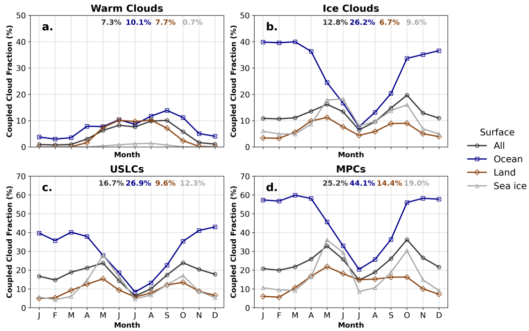
Figure 9. Monthly evolution of low-level (between clutter height and 3 km AGL) coupled cloud fractions over different surface types (ocean, land, sea ice, and all surfaces). Panels show (a) warm clouds, (b) ice clouds, (c) USLCs, and (d) MPCs.
