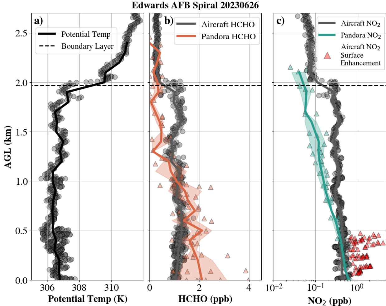
Figure 3. Vertical profiles of (a) potential temperature, (b) HCHO, and (c) NO 2 . The boundary layer height is denoted as the dotted lines. The in situ airborne data are the gray markers and binned to 100 m (solid line). The shaded region represents measurement uncertainty. Pandora data are orange (HCHO) and blue (NO 2 ) markers (solid lines are data binned to 100 m). The shaded region represents \pm one standard deviation. The red triangles in (c) are the NO 2 enhancement observed in the southeast quadrant in Fig. 2, defined as the upper 25 th percentile of the near surface observations (< 0.5 km).
