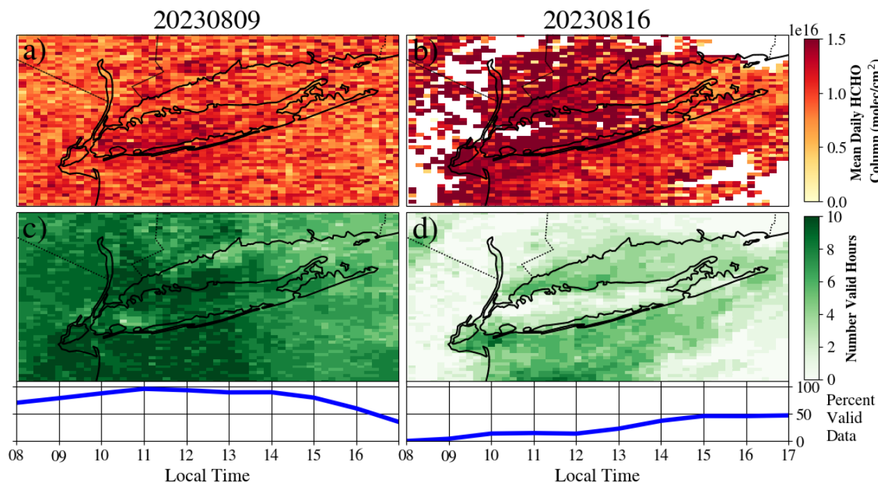
Figure 7. (a,b) Daily average TEMPO HCHO columns for NYC3 and NYC4 from 8-17 EDT. (c,d) Number of data points included in the average for each grid box and time series of the percentage of valid data in the domain.
