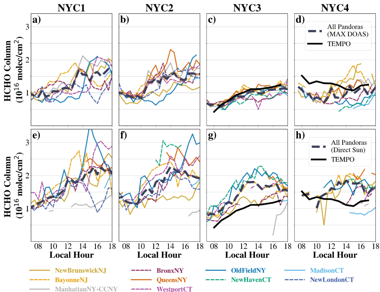
Figure 5. MAX DOAS tropospheric column (a-d) and DS total column (e-h) HCHO from NYC Pandoras on the four flight days averaged to 30 minutes. The individual stations are colored, and the mean value is shown as the dotted gray line. The hourly NYC domain (Fig. 4) average TEMPO HCHO column is included on NYC3 and NYC4 as the solid black line.
