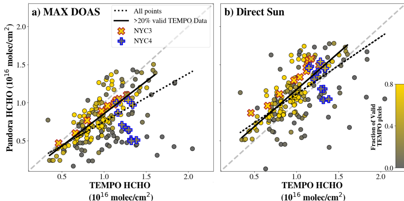
Figure 8. Average TEMPO HCHO column for the entire NYC domain (Fig. 4) versus average NYC Pandora MAX DOAS tropospheric column (a) and Direct Sun total column (b) from August 2 nd to August 31 st , 2023. Each marker represents one hour of data and are colored by the percentage of available TEMPO data for the domain. Data from NYC3 and NYC4 are outlined as the red X's and blue crosses, respectively. Theil Sen lines of best fit for all data (dotted) and those with > 20% valid data (solid) are included.
