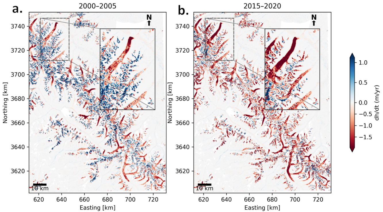
385 Figure 8: Glacier surface elevation change (Hugonnet et al, 2021). a-b: show the elevation change map for different periods (2000-2005 & 2015-2020). The colour bar represents the 2 nd -98 th percentile of elevation change. The inset in panel a & b shows the tongue of the Drang Drung glacier and its neighbouring glaciers.
