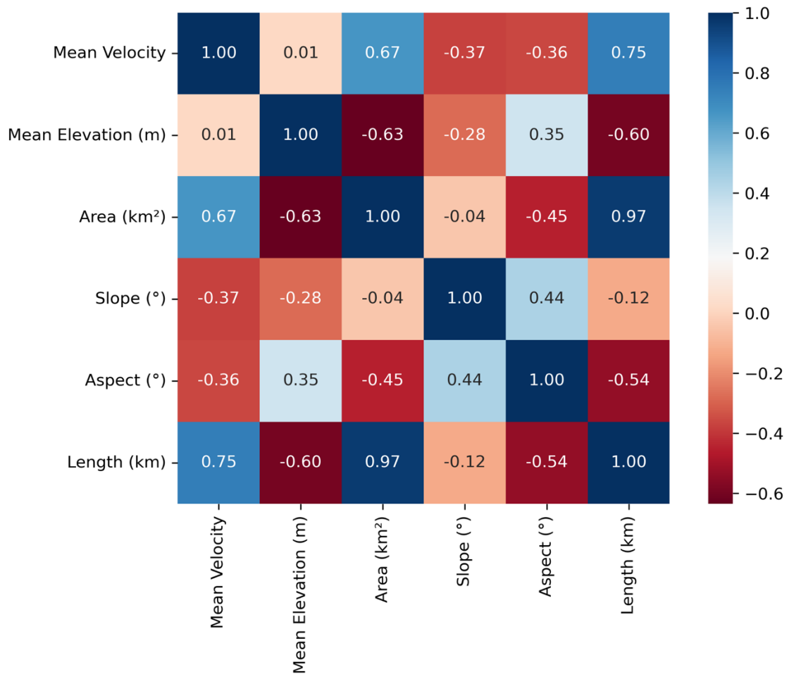
400 Figure 9: Correlation matrix between mean surface velocity and non-climatic variables such as Mean elevation (m), Area (km 2 ), Slope (in degrees), Aspect (in degrees) and length (km)
