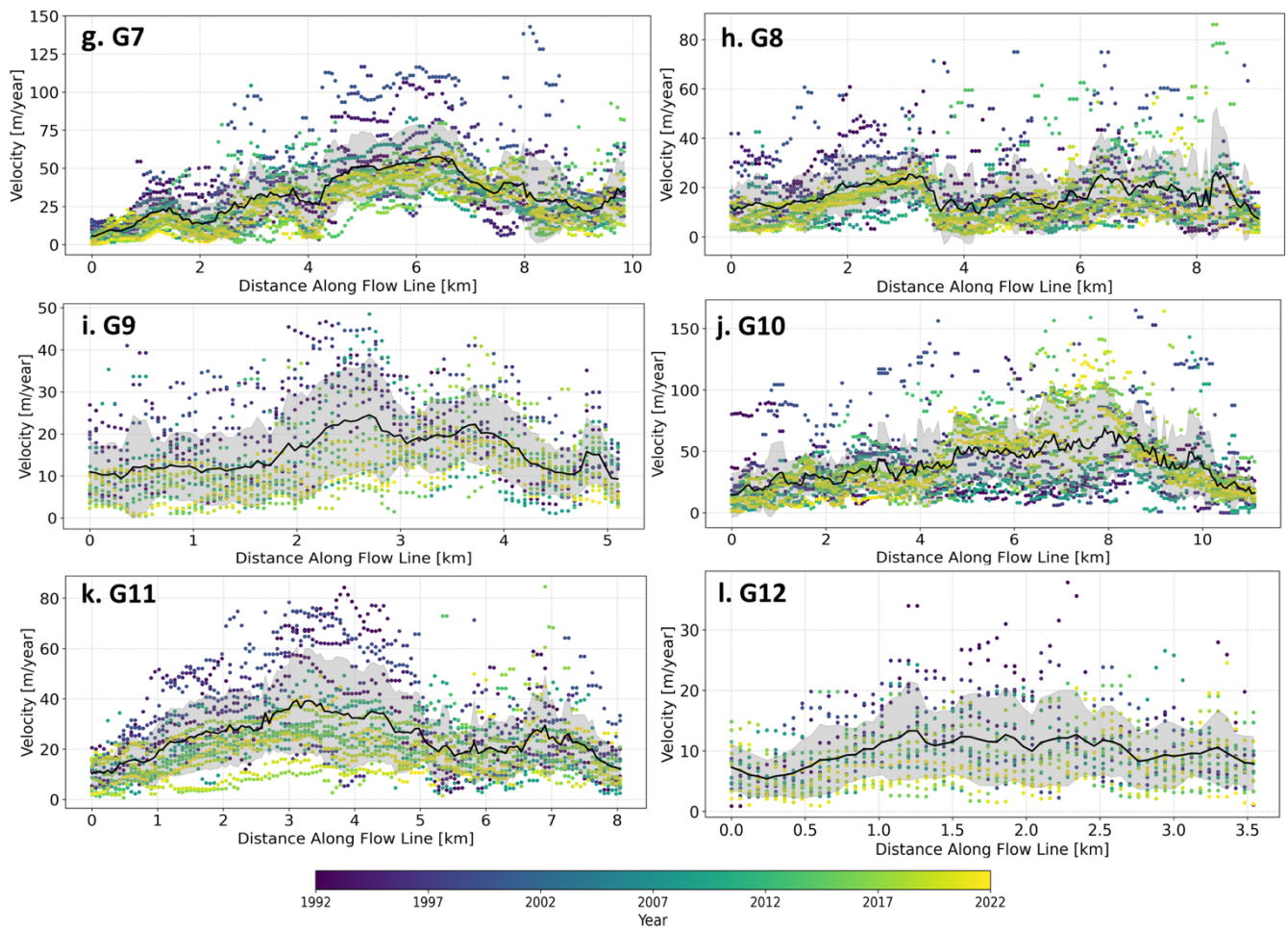
345 Figure 5: (a-l) Scatter plots showing the glacier velocity profile along the central flowline for all the glaciers from 1992–2023. The x-axis represents the distance along the flowline (km) from the start of the terminus (marked by the origin). The different colours represent data points from different years. The black thick line refers to the mean velocity across the time period.
