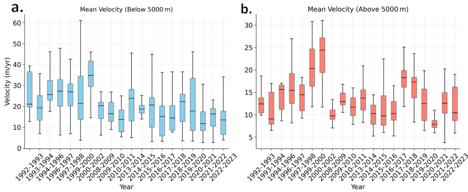
320 Figure 4: Box plots for the mean velocity ( \text{m year}^{-1} ) for the region of glaciers with elevation a) below 5000m; and b) above 5000m. In each panel, the median velocity trend is denoted by the black horizontal line, the interquartile range is shown in the coloured box, and the lines and whiskers denote the maximum value (upper) and minimum value (lower), excluding the outliers. Outliers are not included in the plot.
