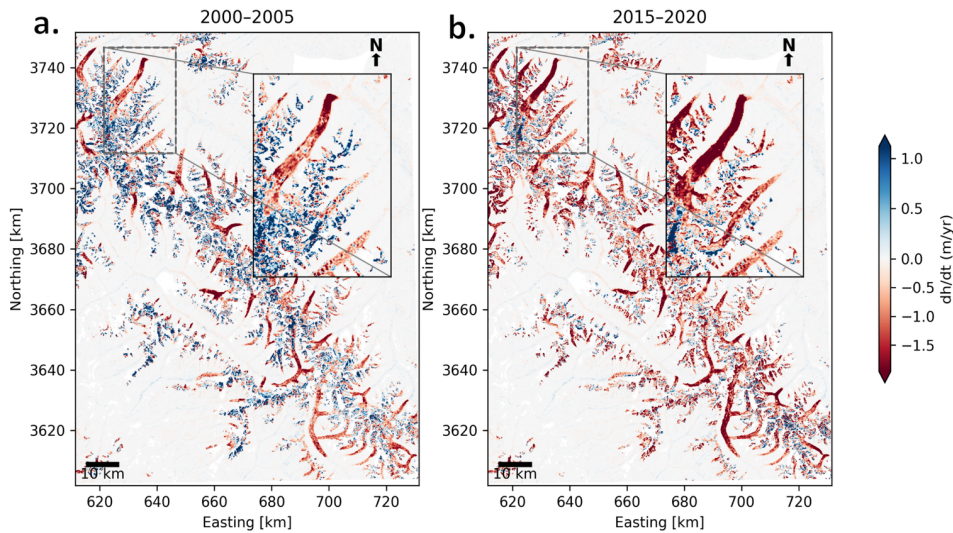
395 Figure 8: Glacier surface elevation change (Hugonnet et al, 2021). a-b: show the elevation change map for different periods (2000-2005 & 2015-2020). The colour bar represents the 2 nd -98 th percentile of elevation change. The inset in panel a & b shows the tongue of the Drang Drung glacier and its neighbouring glaciers.
