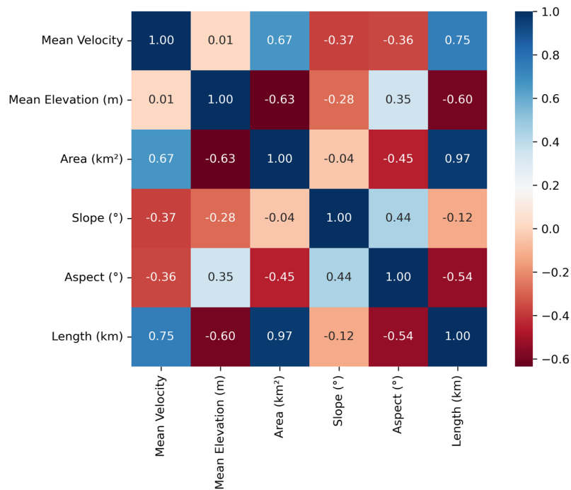
410 Figure 9: Correlation matrix between mean surface velocity and non-climatic variables such as Mean elevation (m), Area (km 2 ), Slope (in degrees), Aspect (in degrees) and length (km)
