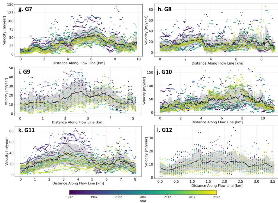
355 Figure 5: (a-l) Scatter plots showing the glacier velocity profile along the central flowline for all the glaciers from 1992-2023. The x-axis represents the distance along the flowline (km) from the start of the terminus (marked by the origin). The different colours represent data points from different years. The black thick line refers to the mean velocity across the time period.
