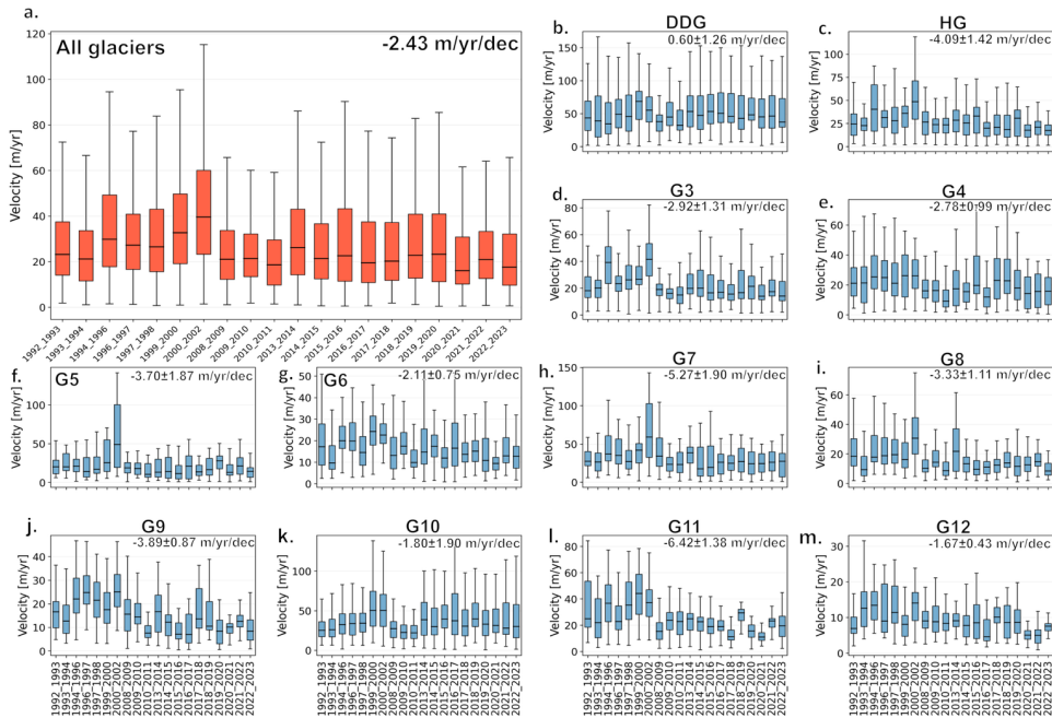
305 Figure 3: a) Mean velocity ( \text{m year}^{-1} ) for all the glaciers. (b-m) Mean velocities ( \text{m year}^{-1} ) for individual glaciers from DDG to G12. Each panel shows the interquartile range (shaded orange and blue box) with the median denoted by the black horizontal line, lines and whiskers denote the maximum value (upper) and minimum value (lower), excluding the outliers. The trend is reported in the upper right corner of each panel (which considers the data gap).
