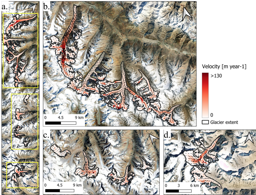
300 Figure 2: Glacier velocity in \text{m year}^{-1} from 2020-2021 for the selected glaciers (with extents outlined in black), subdivided into three different groups. The left vertical panel (a) shows all the glaciers investigated with insets on the right outlined by yellow boxes; b) velocity for glaciers DDG, HG, G3, G4 and G5; c) velocity for glaciers G6, G7 and G8; d) velocity for glaciers G10 and G11.
