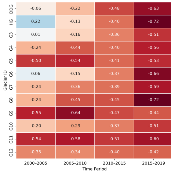
380 Figure 7: Glacier-wide mean elevation change ( dh/dt ) in m year -1 for different periods. Blue denotes thickening and red denotes thinning.
