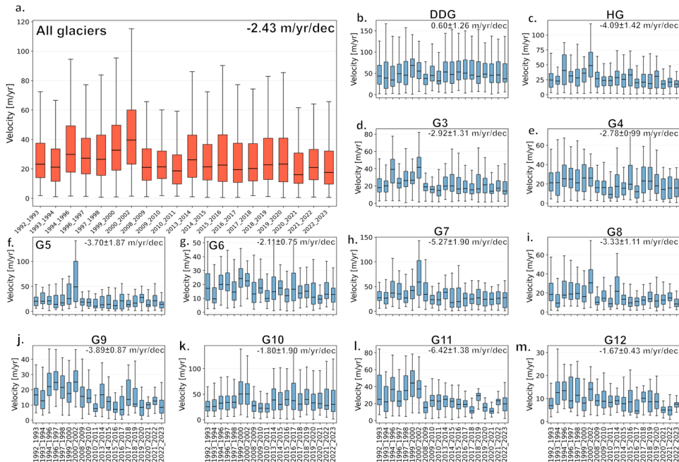
Figure 3: a) Mean velocity (m year -1 ) for all the glaciers. (b-m) Mean velocities (m year -1 ) for individual glaciers from DDG to G12. Each panel shows the interquartile range (shaded orange and blue box) with the median denoted by the black horizontal line, lines and whiskers denote the maximum value (upper) and minimum value (lower), excluding the outliers. The trend is reported in the upper right corner of each panel (which considers the data gap).
