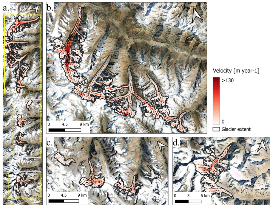
440 Figure 2: Glacier velocity in \text{m year}^{-1} from 2020-2021 for the selected glaciers (with extents outlined in black), subdivided into three different groups. The left vertical panel (a) shows all the glaciers investigated with insets on the right outlined by yellow boxes; b) velocity for glaciers DDG, HG, G3, G4 and G5; c) velocity for glaciers G6, G7 and G8; d) velocity for glaciers G10 and G11.
