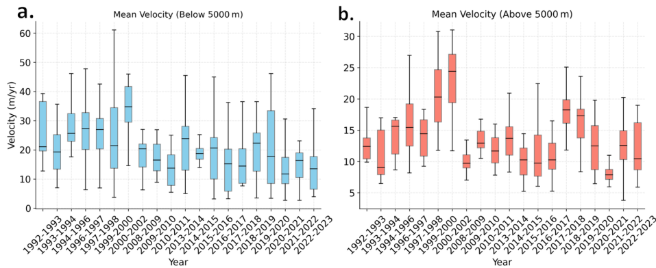
Figure 4: Box plots for the mean velocity ( \text{m year}^{-1} ) for the region of glaciers with elevation a) below 5000m; and b) above 5000m. In each panel, the median velocity trend is denoted by the black horizontal line, the interquartile range is shown in the coloured box, and the lines and whiskers denote the maximum value (upper) and minimum value (lower), excluding the outliers. Outliers are not included in the plot.
