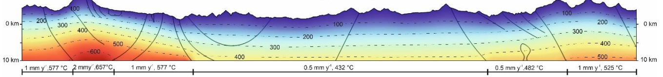
Model 2: Slow exhumation - high radiogenic heat production
