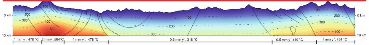
Surface heat flow ( \text{mW m}^{-2} )
