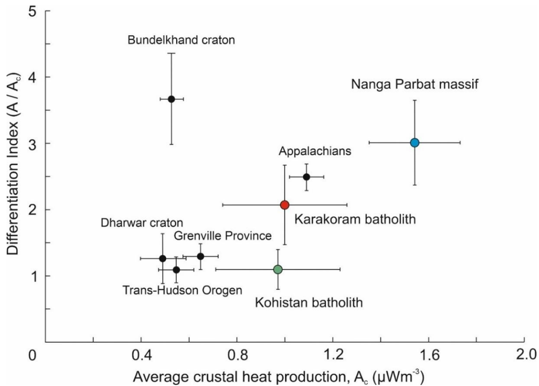
Figure 8: Plot of differentiation index ( D_f ) vs. average crustal heat production ( A_c ) for the Nanga Parbat Massif, Kohistan and Karakoram batholith in comparison with Indian shields (after Podugu et al., 2017) and North American geological provinces (after Perry et al., 2006). Values for the NPM, Kohistan and Karakoram are derived from modelled surface heat flow, whereas the comparison provinces are based on measured heat-flow.
