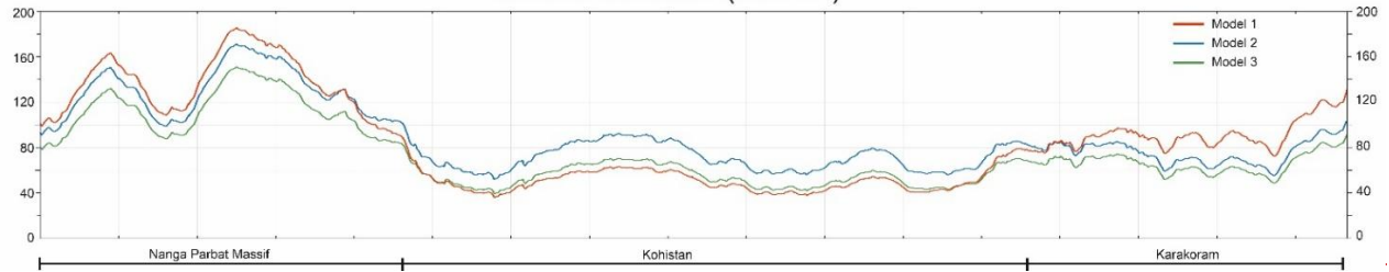
Surface heat flow ( \text{mW m}^{-2} )
