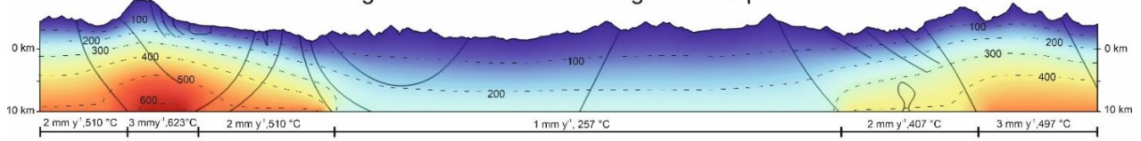
Model 2: Low exhumation - high radiogenic heat production
