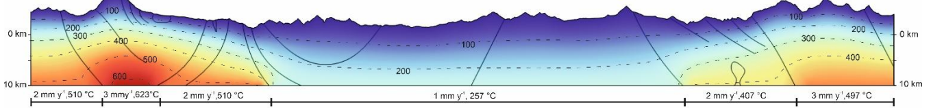
Model 1: Fast exhumation - low radiogenic heat production
