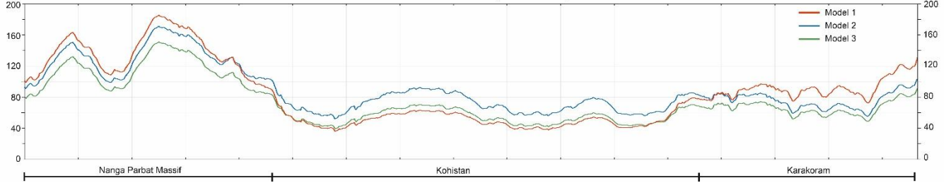
Figure 7: 2D simulation results showing subsurface temperature distribution and surface heat flow with basal temperature input from 1D transient advective-conductive models, which test combination testing combinations of variable exhumation rates and radiogenic heat production scenarios for the Nanga Parbat Massif, Kohistan and Karakoram. Advective and diffusive heat transfer is accounted for by modeling the translation of the respective lithospheric blocks during exhumation.
