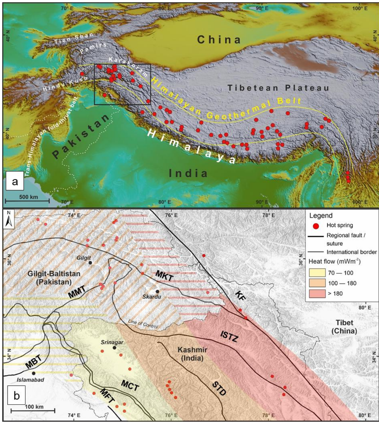
Figure 1: (a) Topographic map of south Asia showing the distribution Distribution of hot springs of the Himalaya Geothermal Belt-HGB (after Hochstein & Zhongke, 1995) within the hinterland of India-Asia collision zone. The black rectangle shows the location of Fig 1.1b. (b) Distribution of geothermal manifestations (as hot springs) in the hinterland of western Himalaya and Karakoram and associated interpolated heat-flow map (modified after Shanker, 1988; Thussu, 2002; Craig et al., 2013). Heat-flow is calculated from geothermal fields in Indian Kashmir and has been projectedextrapolated towards northwest in Pakistan (line filled pattern) by Craig et al., 2013. Abbreviations: KF-Karakoram Fault; ISTZ-Indus Tsangpo Suture Zone; MBT-Main Boundary
