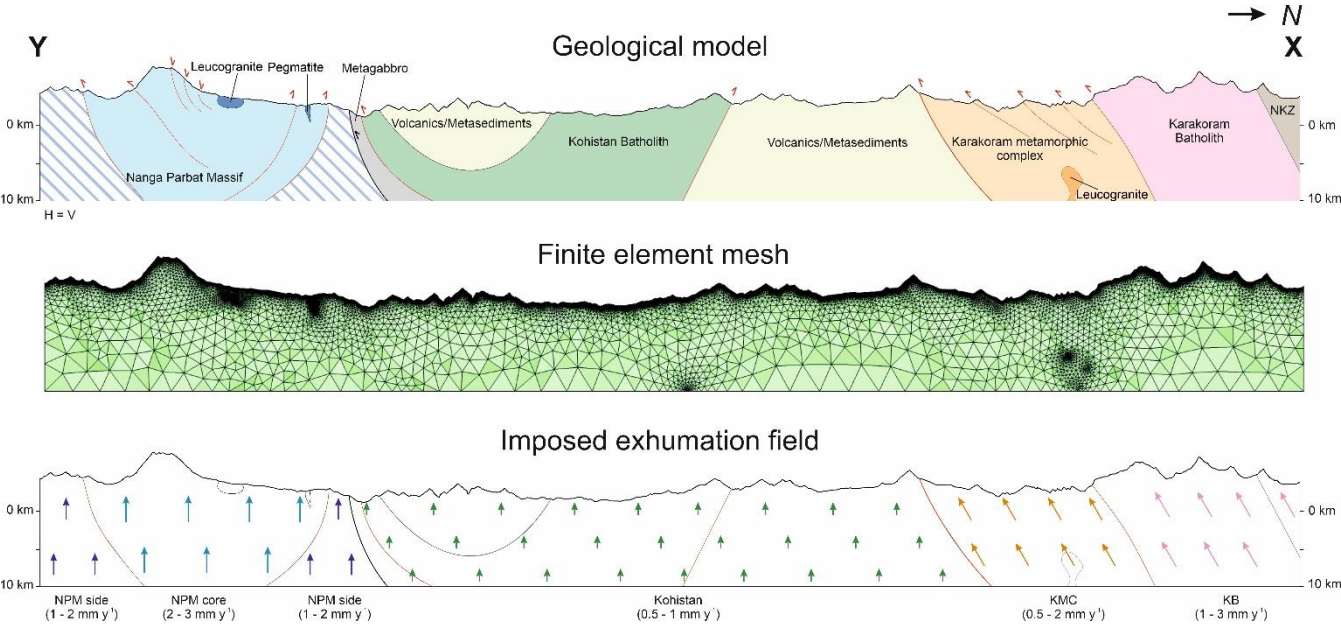
Figure 6: Top: Geological model of the XY profile in Fig 5a showing the subsurface geological structure of the major lithological units up to 10 km below sea level (modified after Searle & Khan, 1996). Bottom Centre: Two-dimensional triangular finite-element mesh containing 7264372,643 elements created in COMSOL Multiphysics® for the dynamic thermal modelling. Bottom: Subdivision of the model domain into kinematic blocks with the imposed translation velocity ranges used in Models 1–3.
