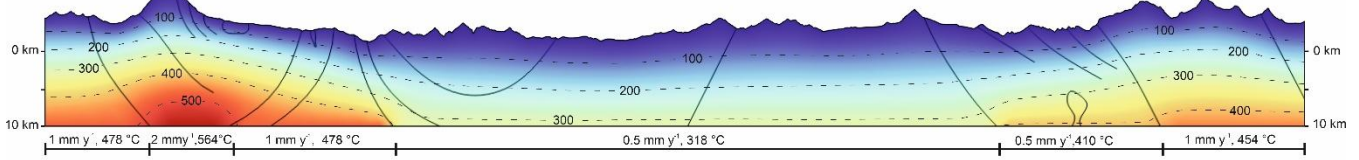
Surface heat flow ( \text{mW m}^{-2} )
