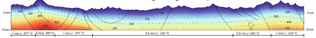
Model 3: Low exhumation - moderate radiogenic heat production
