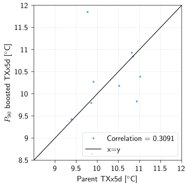
Figure A5. Correlation between TXx5d of parent event and the 90 th percentile of TXx5d among its boosted simulations. Spearman correlation between TXx5d of parent event and the 90 th percentile of TXx5d among its boosted simulations.
