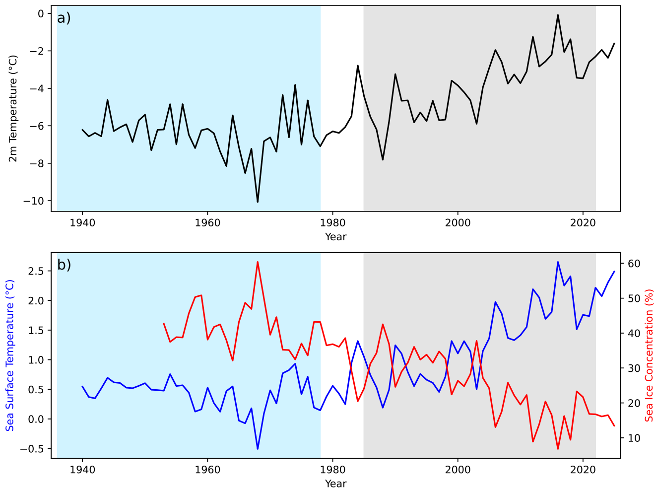
Figure 9. Early spatial Spatial average of ERA5 T2m (a), SST and SIC (b) over Svalbard between 1940 and 2023. The blue (resp. gray) area represents the time frame covered by this study (resp. Li et al., 2025).
