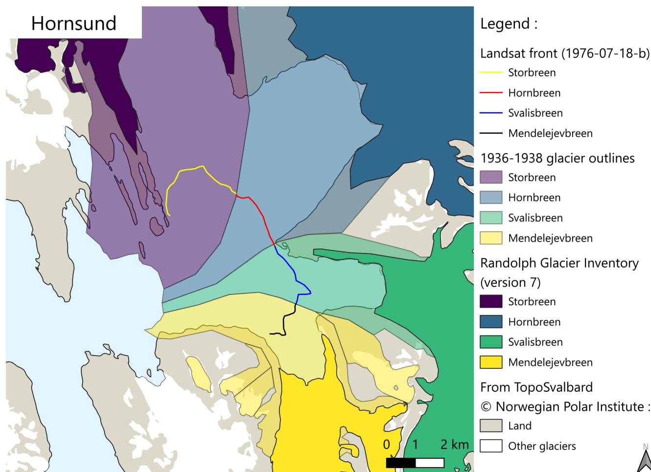
Figure 5. Example of split of glacier fronts in Hornsund (cf. red box in Fig. 4 ). RGI (RGI 7.0 Consortium, 2023, , plain) and 1936 (semi-transparent) outlines are also displayed to show the boundaries between the different glaciers.
