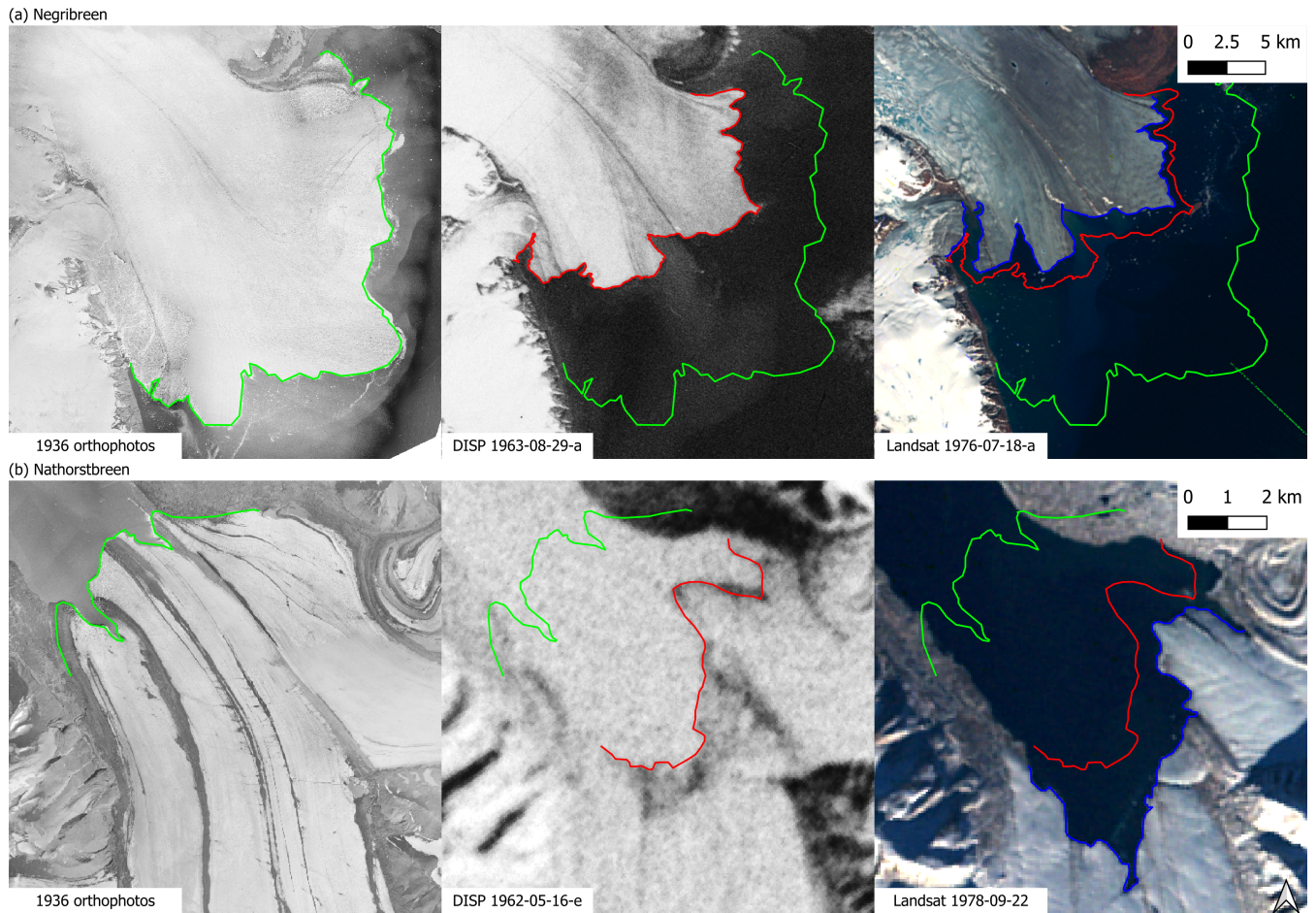
Figure 14. 1936 aerial photograph (left), 1962–1963 DISP (center) and 1976–1978 Landsat MSS (right) images for the Negribreen (a) and Nathrostbreen Nathorstbreen (b) retreats. The green lines (resp. red, blue) correspond to the 1936 (resp. 1962–1963, 1976–1978) fronts. Note the different scales for different glaciers. Image credits: Norwegian Polar Institute (aerial images) and U.S. Geological Survey (DISP and Landsat).
