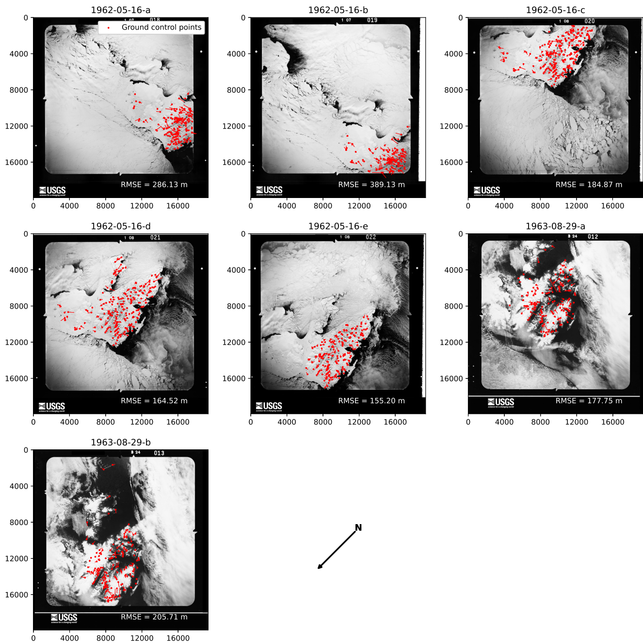
Figure B2. Scatter plots of GCPs' pixel coordinates and residuals for KH-5 ARGON images. GCPs and residuals, expressed in pixel coordinates. The residuals have been multiplied by 50 to enhance readability. The RMSEs are given in the bottom-right corner of each subplot, and the black arrow on the last row indicates the approximate north direction. Image credits: U.S. Geological Survey.
