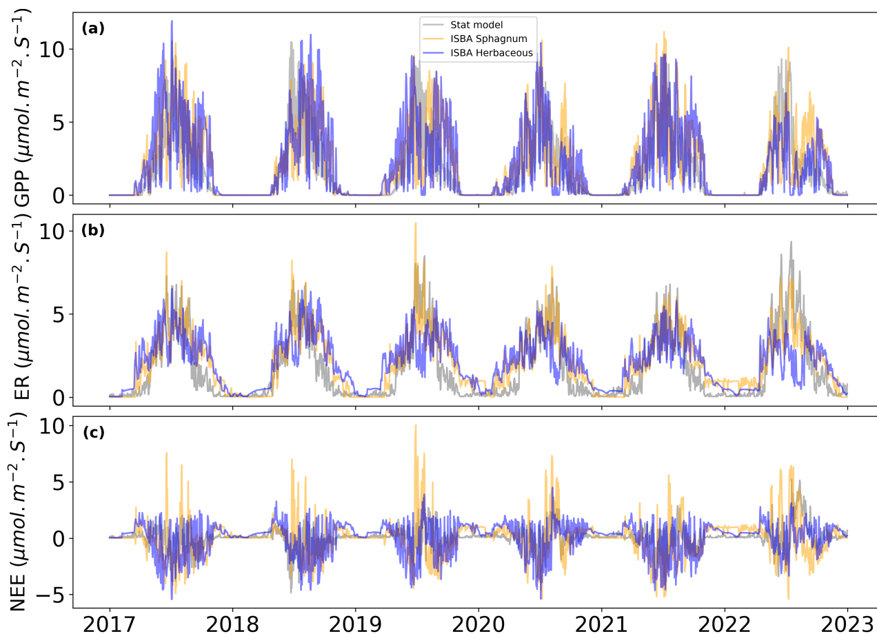
Figure 1. Daily (a) gross primary productivity and (b) ecosystem respiration fluxes compared between statistical models (grey) (Garisoain et al., 2024) and ISBA over the 2017-2022 period for herbaceous (blue) and Sphagnum mosses (orange).
