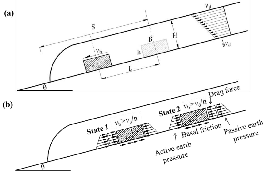
255 Figure 8 Schematic diagram of (a) block moving along with decelerating debris flow, with velocity profile; 260 (b) forces acting on the block: drag force, basal friction, and active/passive earth pressures.
