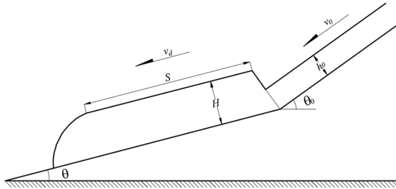
Figure 7 Schematic diagram of leading-edge model
