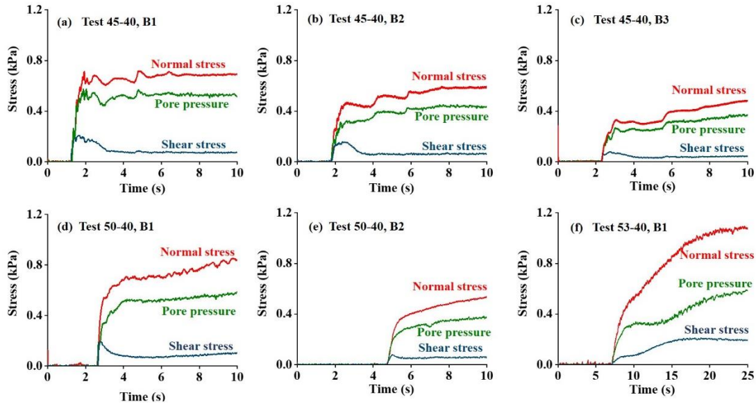
Figure 4. Measured basal normal stress, shear stress, and pore water pressure. (a-c) Test 45-40 at basal sensing module B1 and B2, and B3; (d-e) Test 50-40 at B1 and B2; (f) Test 53-40 at B1.
