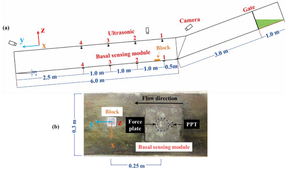
120 Figure 2. Experimental setup and instrumentation: (a) flume set-up; (b) basal sensing module for measurement of normal/shear stresses and pore-water pressure, and a 40 mm × 40 mm × 10 mm block with inertial measurement unit (IMU)
