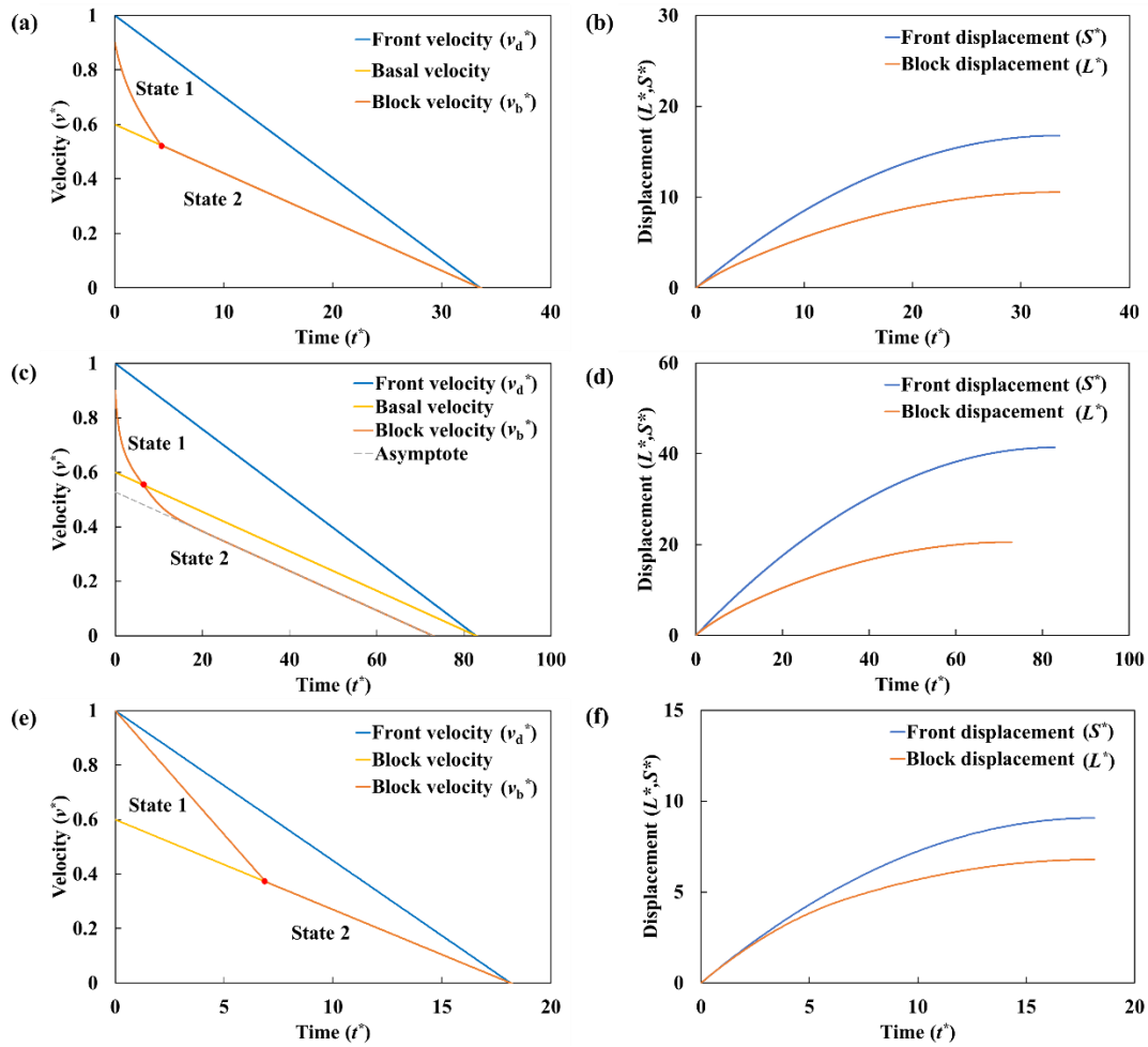
540 Figure 9. The velocity and displacement predicted by the models. Velocity time history of debris flow and block of (a) Model I, (c) and Model II, (e) Model III; displacement time history of debris flow and block of (b) Model I, (d) Model II, and (f) Model III. S^* is debris-flow deposition length (front displacement) and L^* is block displacement. Model I incorporates experimental data from Test 50-40, Model II utilizes data from Test 45-40, and Model III employs data from Test 53-40 (Table 2). Red points demarcate critical thresholds between State 1 and State 2.
