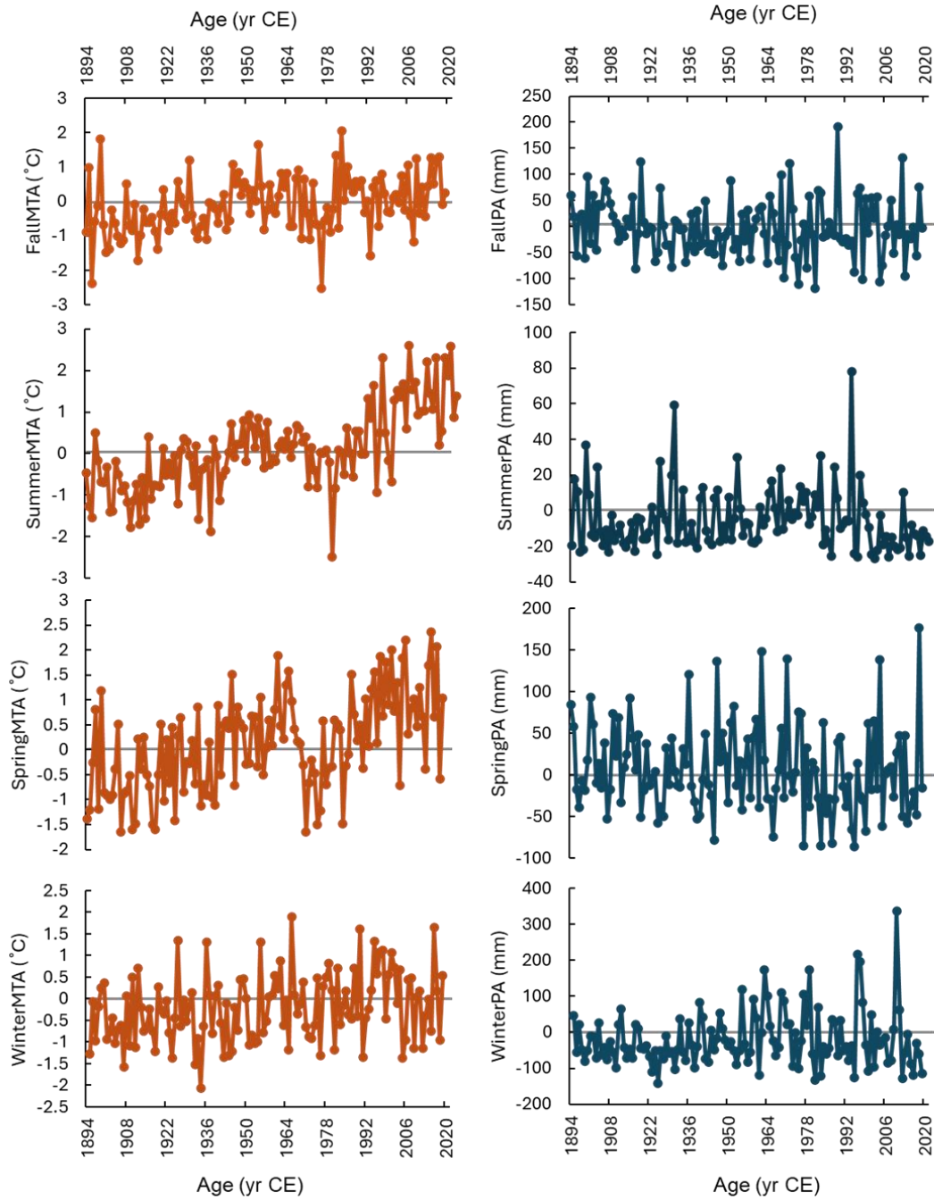
Supplementary Figure 2. Mean seasonal temperature anomalies (Summer-, Spring, Fall- and Winter- MTA), and seasonal precipitation anomalies (Summer-, Spring-, Fall- and Winter- PA) for the period 1894-2020.
