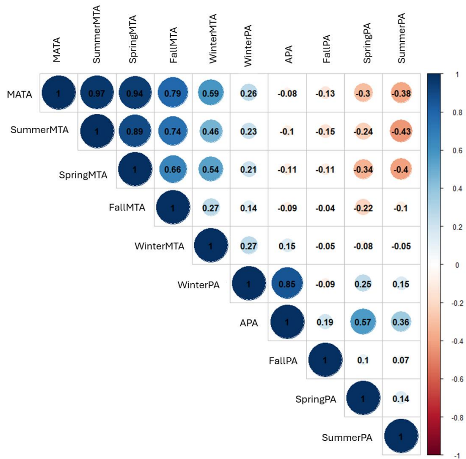
Supplementary Figure 1. Pearson's correlation coefficient matrix between mean annual temperature anomaly (MATA), annual precipitation anomaly (APA), mean seasonal temperature anomalies (Summer-, Spring-, Fall- and Winter- MTA), and seasonal precipitation anomalies (Summer-, Spring-, Fall- and Winter- PA) for the period 1894-2020.
