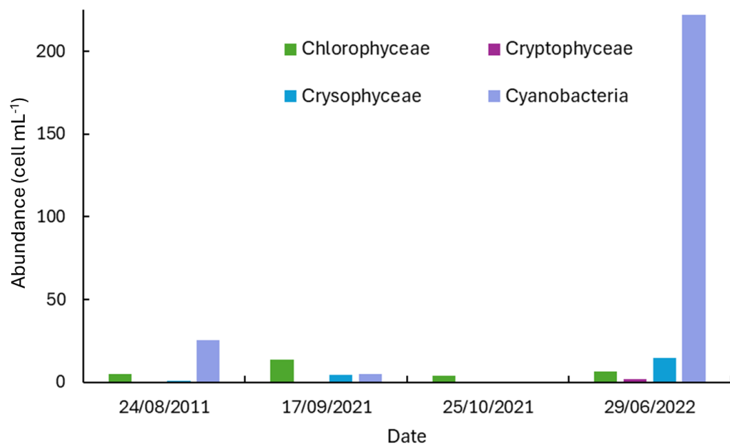
Supplementary Figure 3. Planktonic algae composition and density in Borreguil Lake in selected dates of 2011, 2021 and 2022. 2022 was marked by a massive Saharan dust deposition event.
