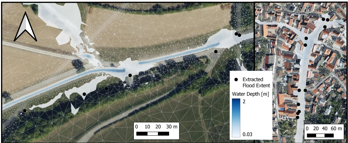
Figure 3. Points of measured flood extent and simulated water extension for the plausibilisation event. Basemaps: Bing Maps © Microsoft Corporation and its data providers.
