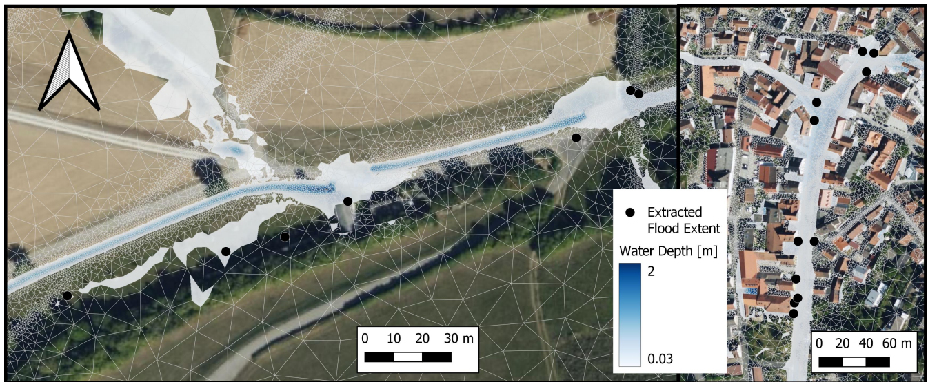
Figure 3. Points of measured flood extent and simulated water extension for the plausibilisation-event event taken for the plausibility assessment . Basemaps: Bing Maps © Microsoft Corporation and its data providers.
