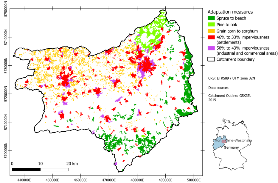
345 Figure 4: Spatial distribution of modeled adaptation measures
